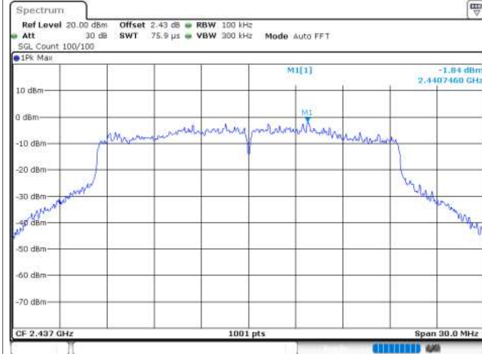
Tx. Spurious NVNT ax20 2437MHz Ant2 Ref
