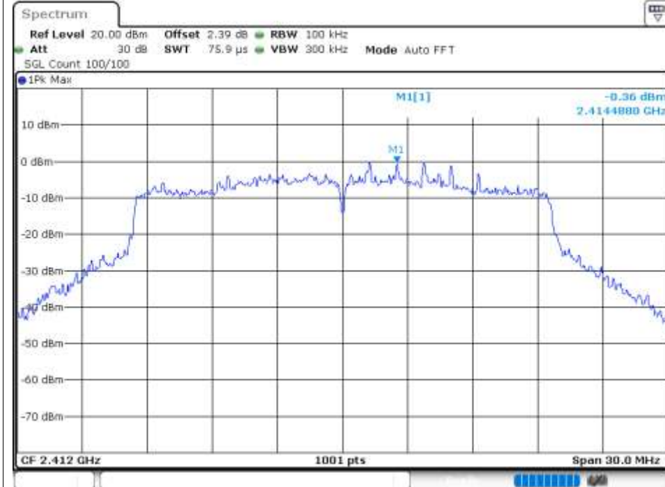
Tx. Spurious NVNT ax20 2412MHz Ant2 Ref
