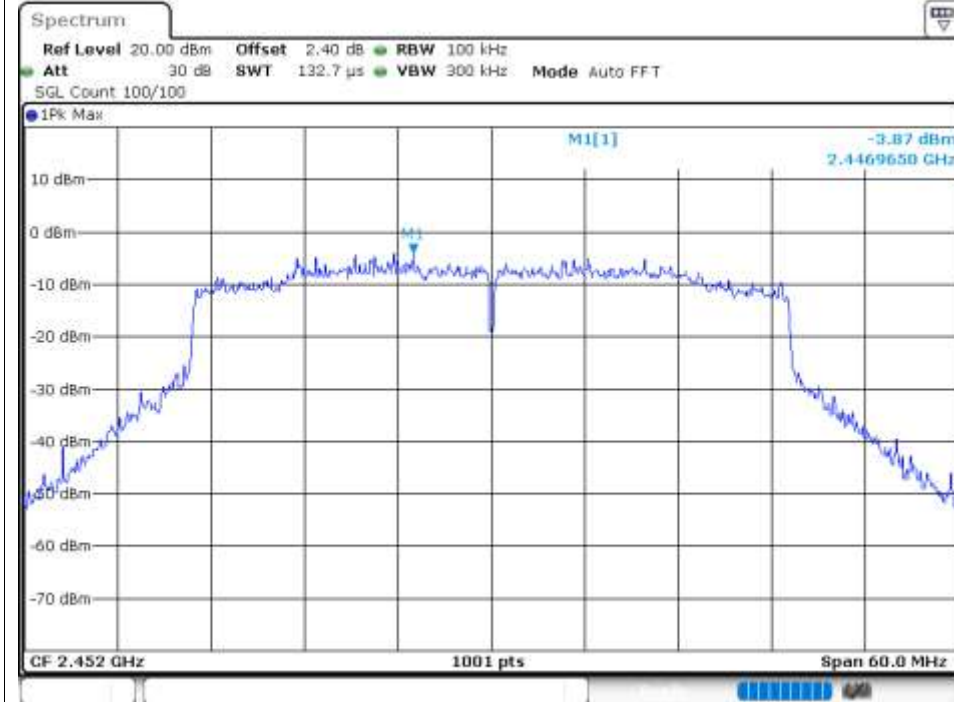
Tx. Spurious NVNT ax40 2452MHz Ant1 Ref
