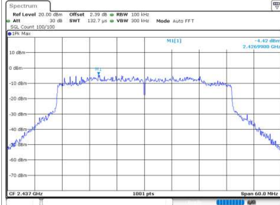
Tx. Spurious NVNT ax40 2437MHz Ant1 Ref
