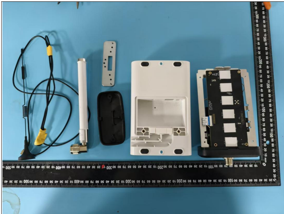
Model equipped with external antenna for LTE
