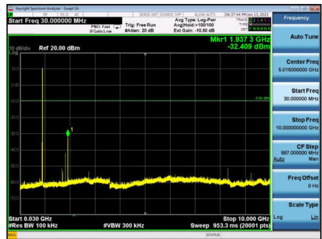
Conducted Spurious Emission: 925.1MHz
