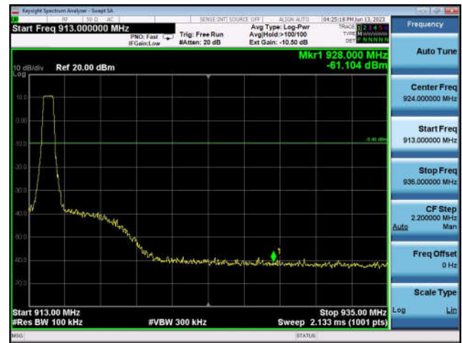
Conducted Band Edge: 914.2MHz
