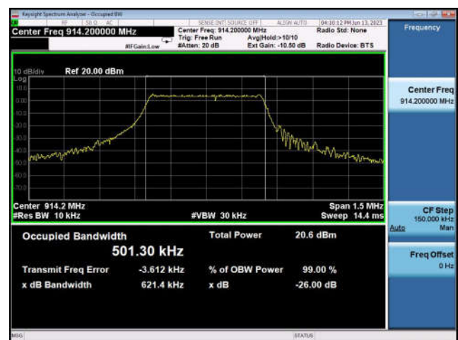
99% OBW: 914.2MHz
