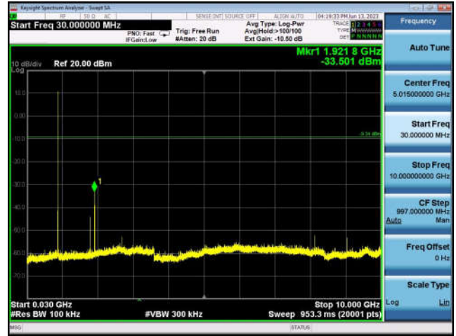
Conducted Spurious Emission: 907.8MHz
