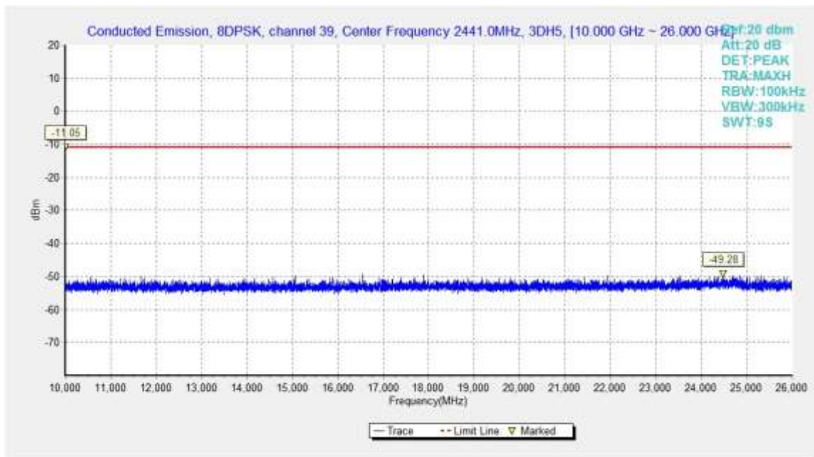
Fig.66. Conducted spurious emission: 8DPSK, Channel 39, 10GHz – 26GHz
