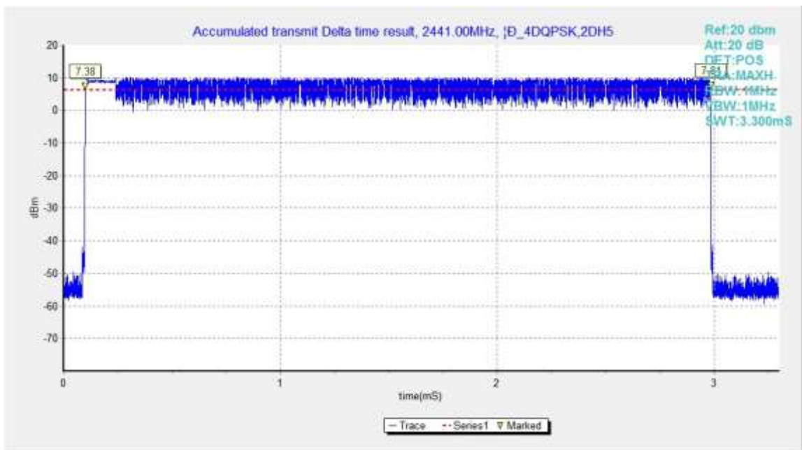
Fig.82. Time of occupancy (Dwell Time): Channel 39, Packet 2-DH5
