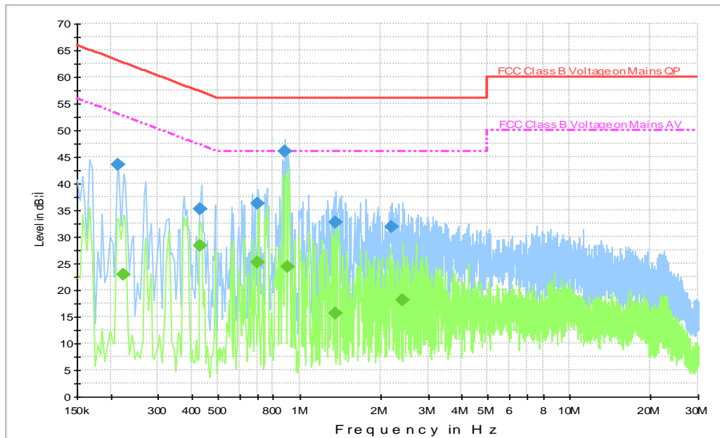
Fig. B11.4 AC Powerline Conducted Emission-802.11a (EUT3 + AE2-4 + AE1-3)
