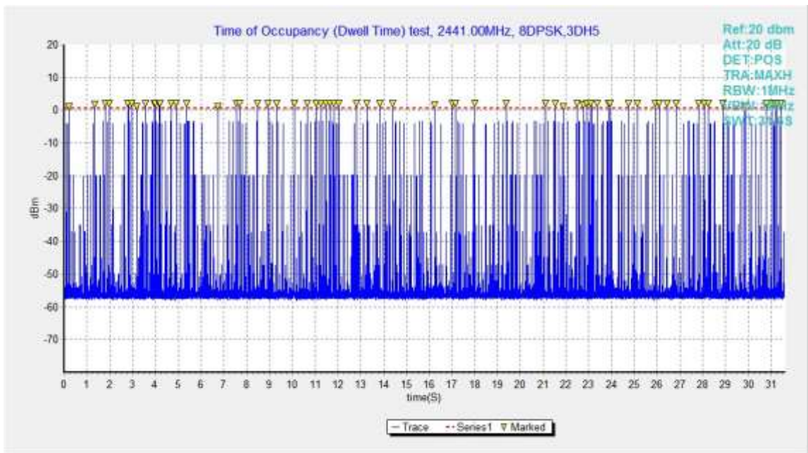
Fig.89. Number of Transmissions Measurement: Channel 39,Packet 3-DH5
