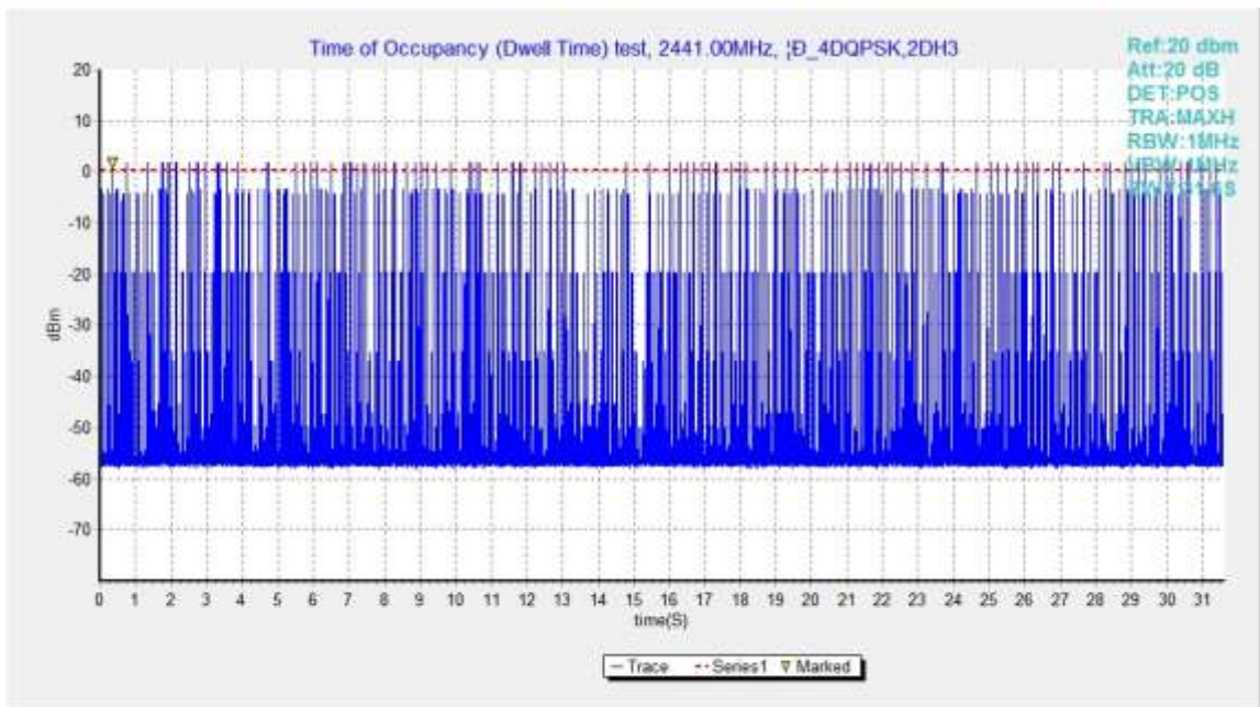
Fig.81. Number of Transmissions Measurement: Channel 39,Packet 2-DH3
