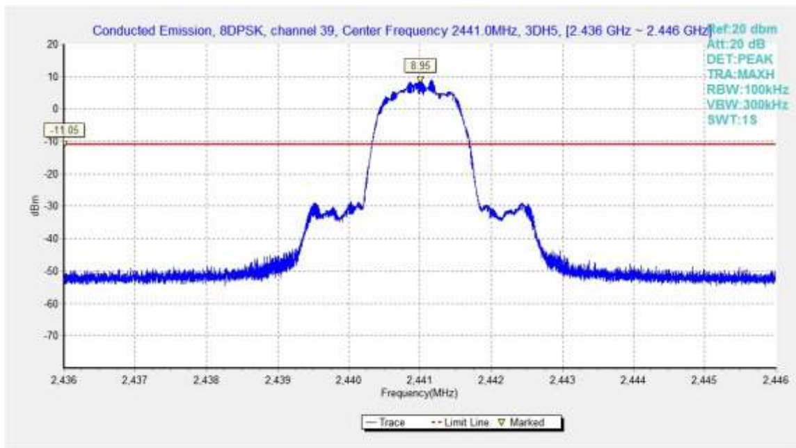
Fig.62. Conducted spurious emission: 8DPSK, Channel 39, 2441MHz
