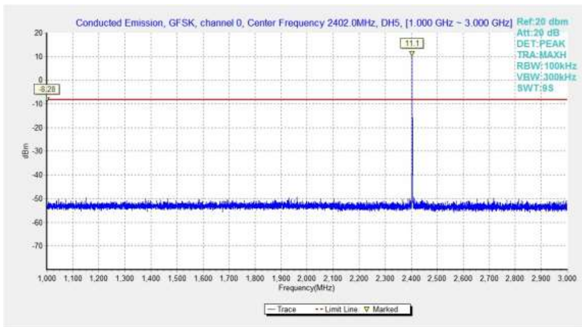
Fig.29. Conducted spurious emission: GFSK, Channel 0, 1GHz - 3GHz
