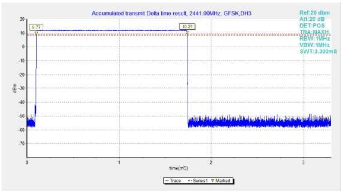
Fig.74. Time of occupancy (Dwell Time): Channel 39, Packet DH3
