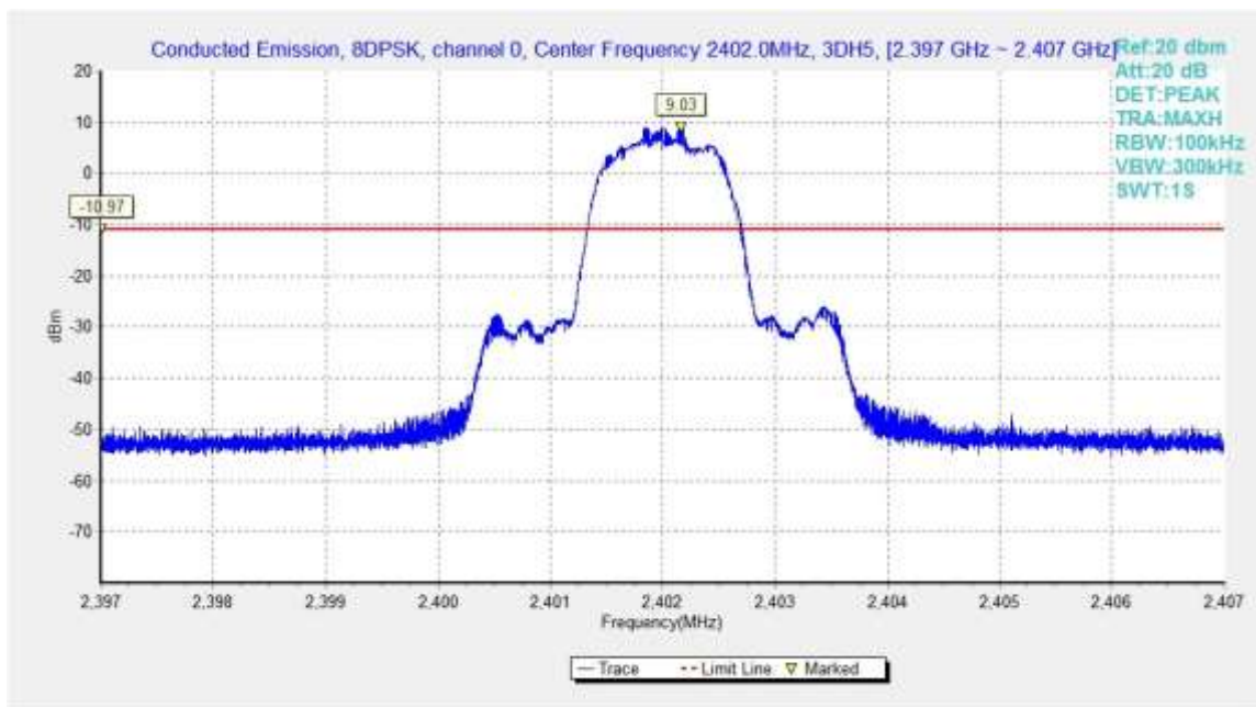
Fig.57. Conducted spurious emission: 8DPSK, Channel 0, 2.402MHz
