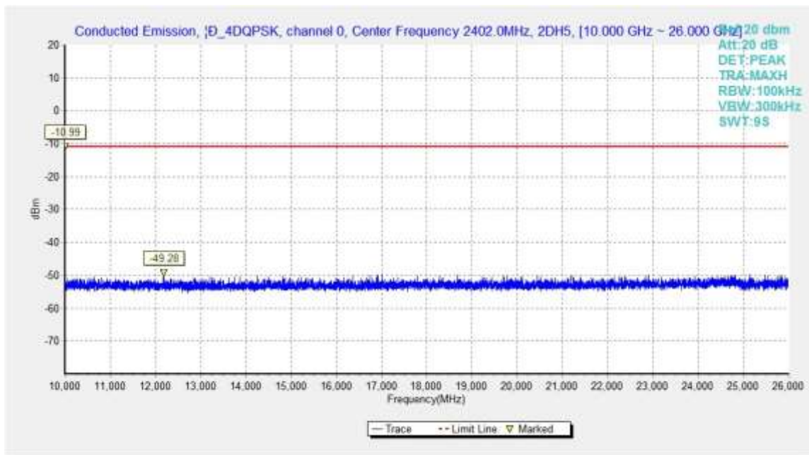
Fig.46. Conducted spurious emission: \pi/4 DQPSK, Channel 0, 10GHz - 26GHz
