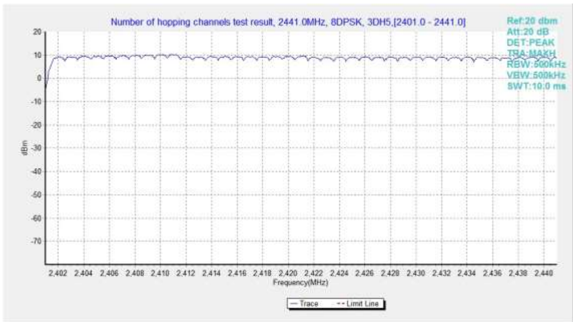
Fig.106. Number of hopping frequencies: 8DPSK, Channel 0 - 39
