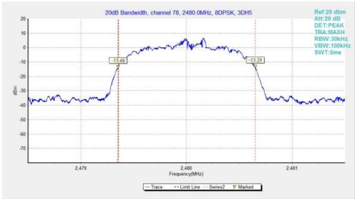
Fig.98. 20dB Bandwidth: 8DPSK, Channel 78
