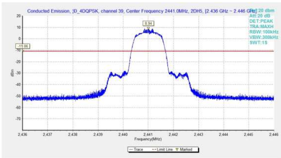
Fig.47. Conducted spurious emission: \pi/4 DQPSK, Channel 39, 2441MHz
