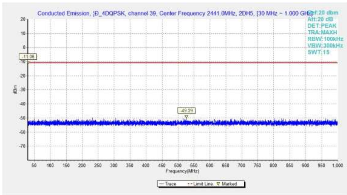
Fig.48. Conducted spurious emission: \pi/4 DQPSK, Channel 39, 30MHz - 1GHz
