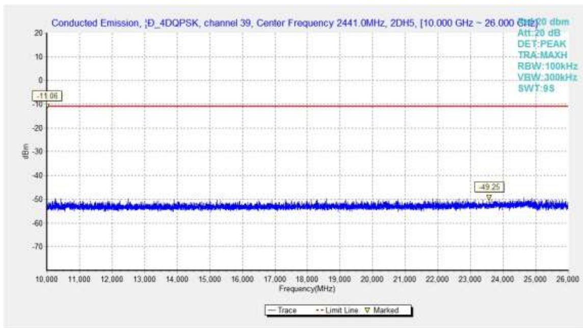
Fig.51. Conducted spurious emission: \pi/4 DQPSK, Channel 39, 10GHz – 26GHz
