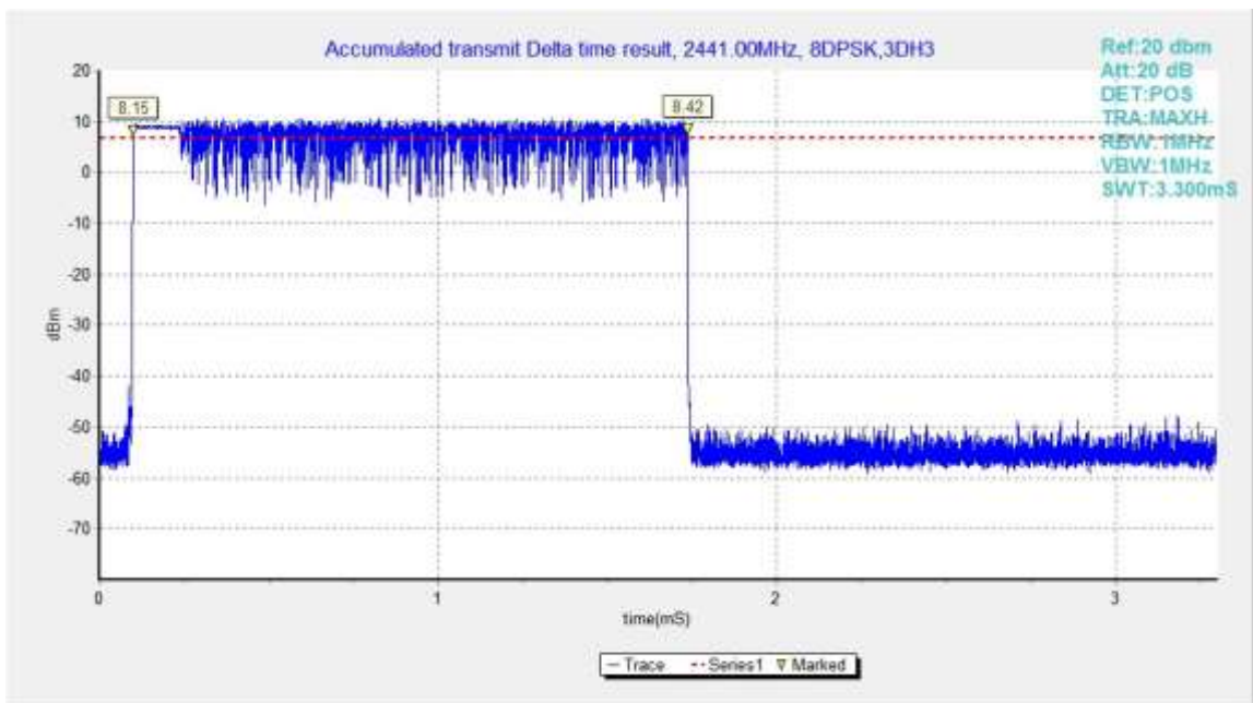
Fig.86. Time of occupancy (Dwell Time): Channel 39, Packet 3-DH3
