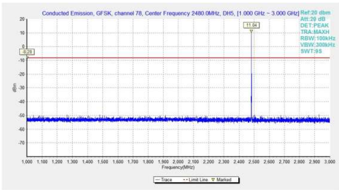
Fig.39. Conducted spurious emission: GFSK, Channel 78, 1GHz - 3GHz
