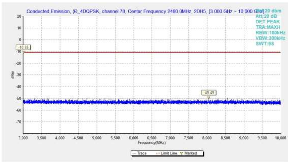
Fig.55. Conducted spurious emission: \pi/4 DQPSK, Channel 78, 3GHz - 10GHz
