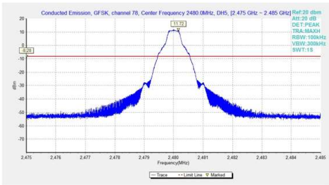
Fig.37. Conducted spurious emission: GFSK, Channel 78, 2480MHz
