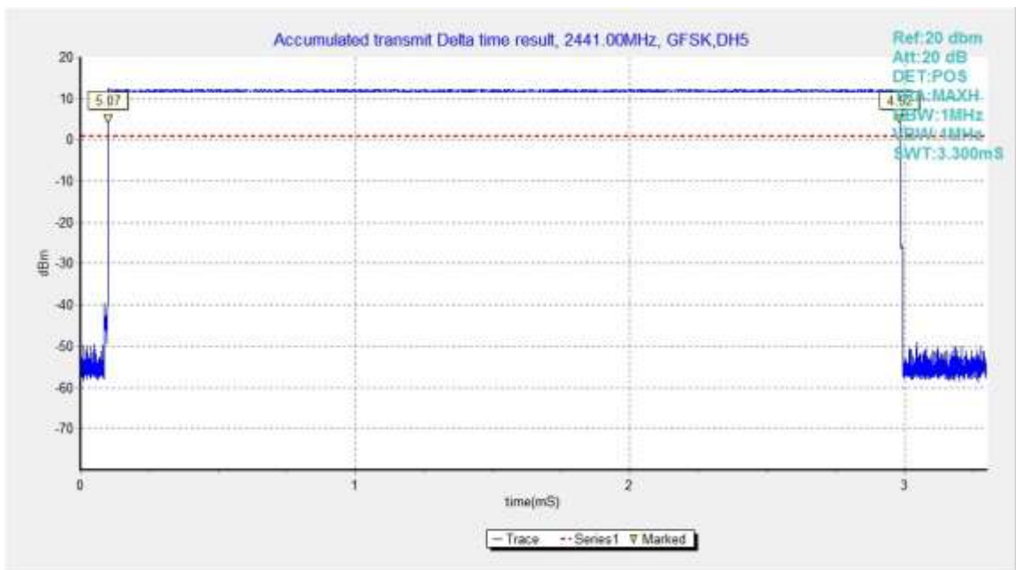
Fig.76. Time of occupancy (Dwell Time): Channel 39, Packet DH5
