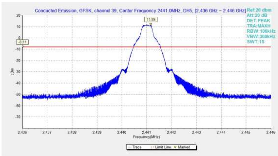
Fig.32. Conducted spurious emission: GFSK, Channel 39, 2441MHz
