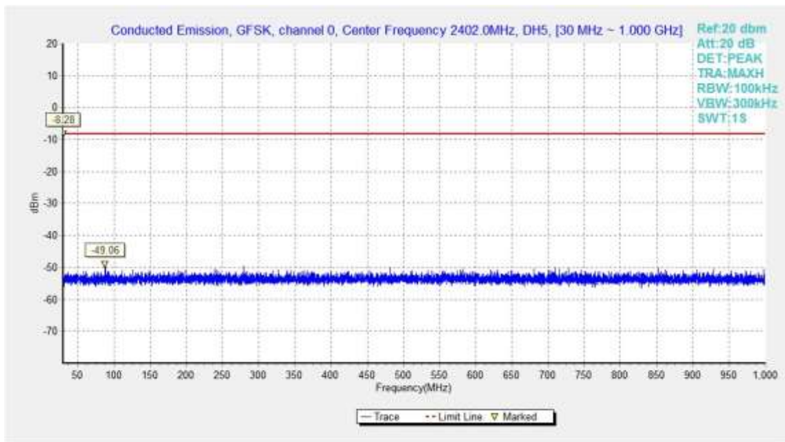
Fig.28. Conducted spurious emission: GFSK, Channel 0, 30MHz - 1GHz
