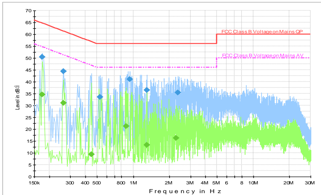
Fig. B11.3 AC Powerline Conducted Emission-802.11a (EUT5 + AE2-3 + AE1-3)
