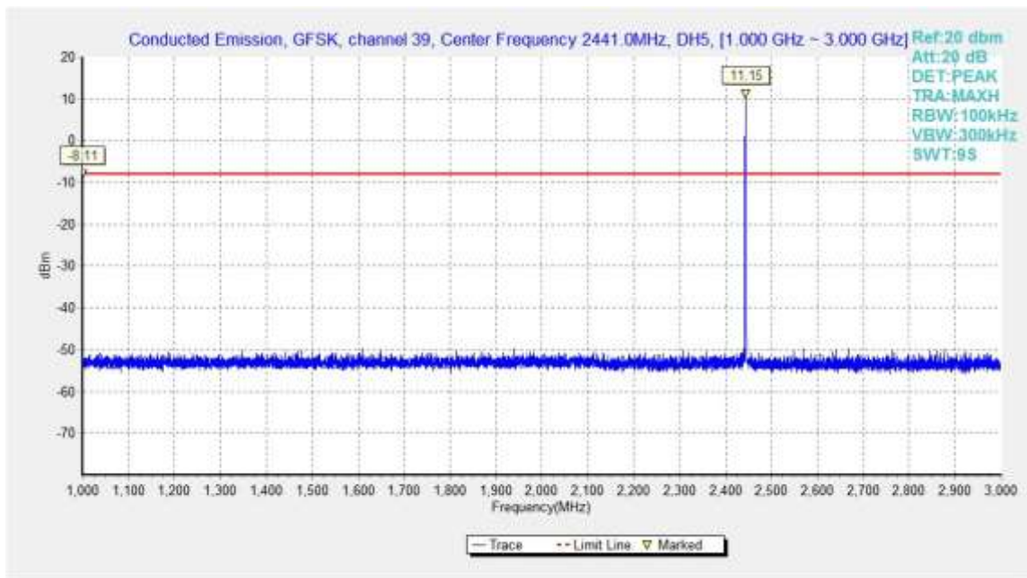
Fig.34. Conducted spurious emission: GFSK, Channel 39, 1GHz – 3GHz
