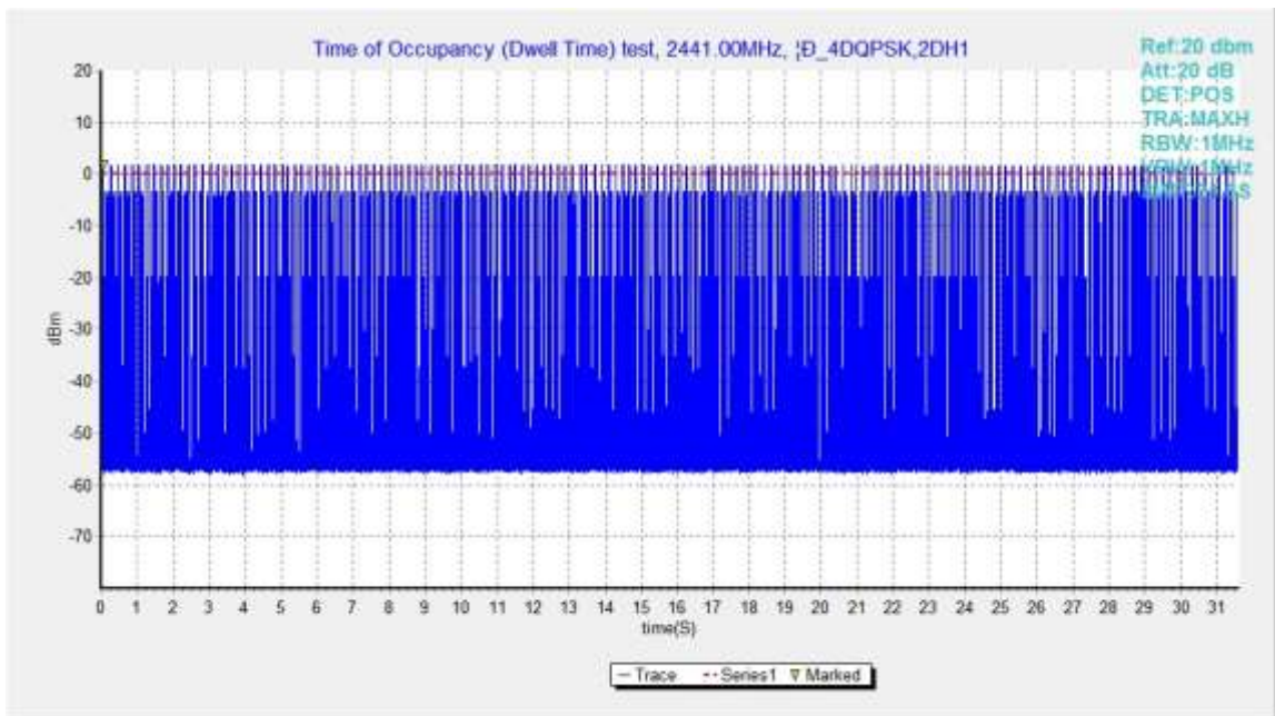
Fig.79. Number of Transmissions Measurement: Channel 39,Packet 2-DH1
