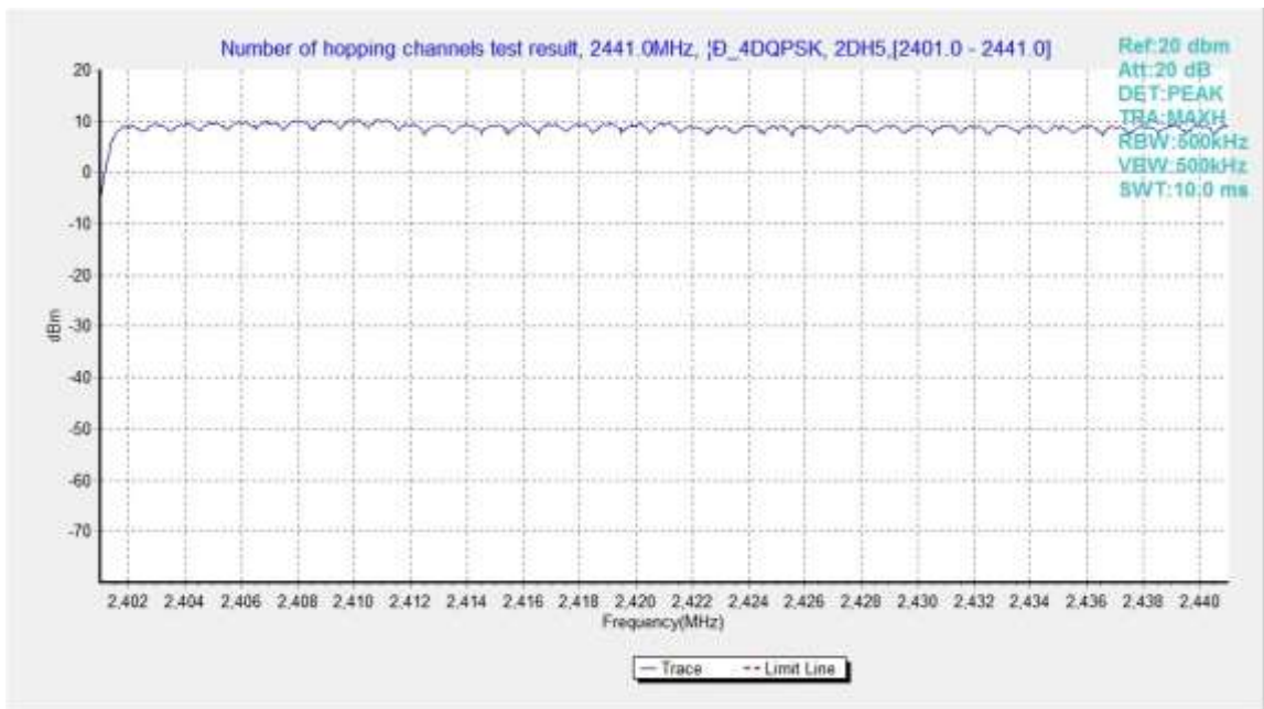
Fig.104. Number of hopping frequencies: \pi/4 DQPSK, Channel 0 - 39
