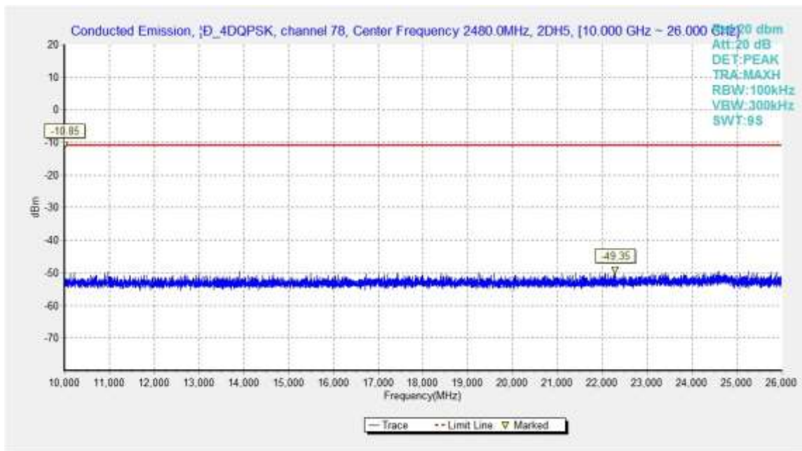
Fig.56. Conducted spurious emission: \pi/4 DQPSK, Channel 78, 10GHz - 26GHz
