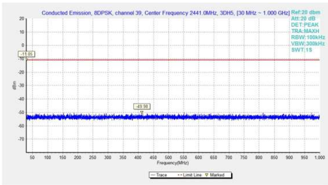
Fig.63. Conducted spurious emission: 8DPSK, Channel 39, 30MHz - 1GHz
