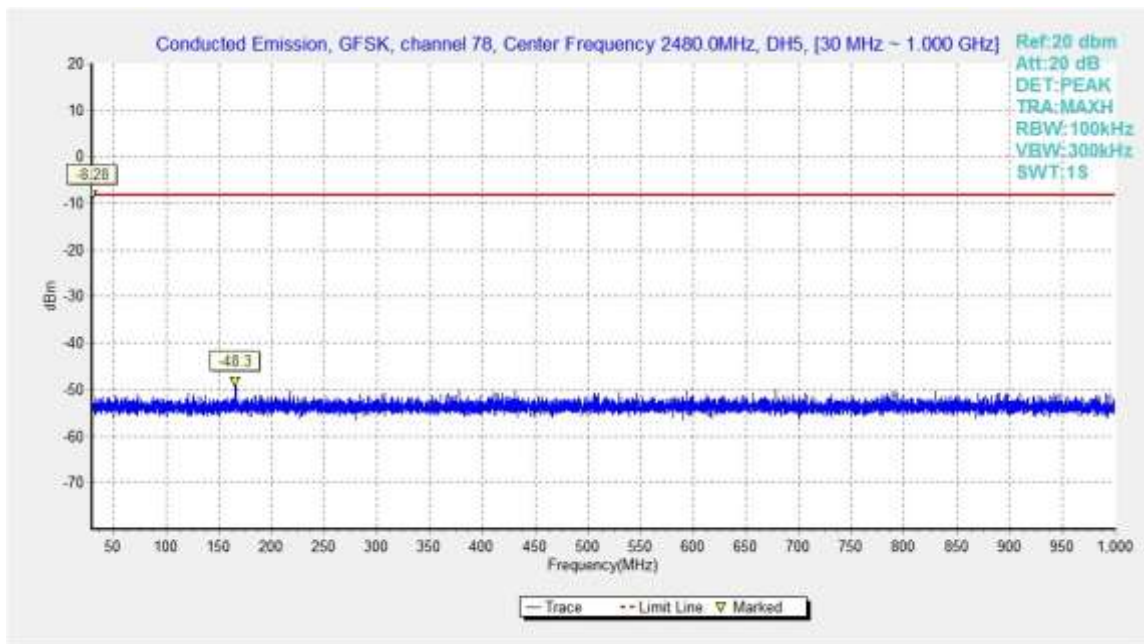
Fig.38. Conducted spurious emission: GFSK, Channel 78, 30MHz - 1GHz
