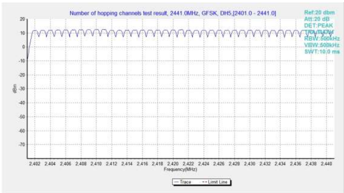
Fig.102. Number of hopping frequencies: GFSK, Channel 0 - 39
