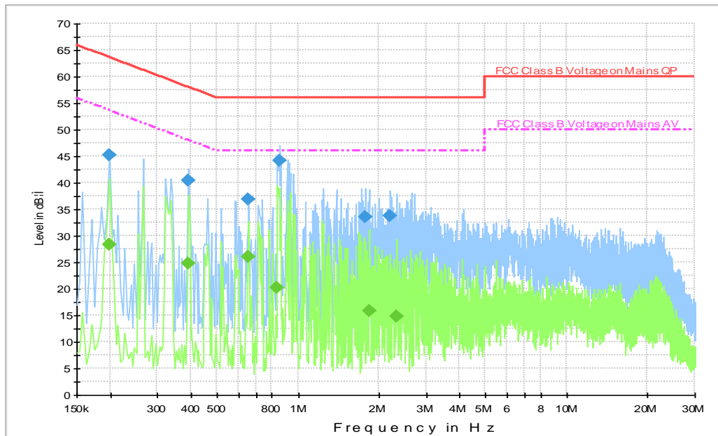
Fig. B11.5 AC Powerline Conducted Emission-802.11a (EUT4 + AE2-5 + AE1-3)
