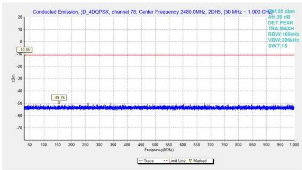
Fig.53. Conducted spurious emission: \pi/4 DQPSK, Channel 78, 30MHz - 1GHz
