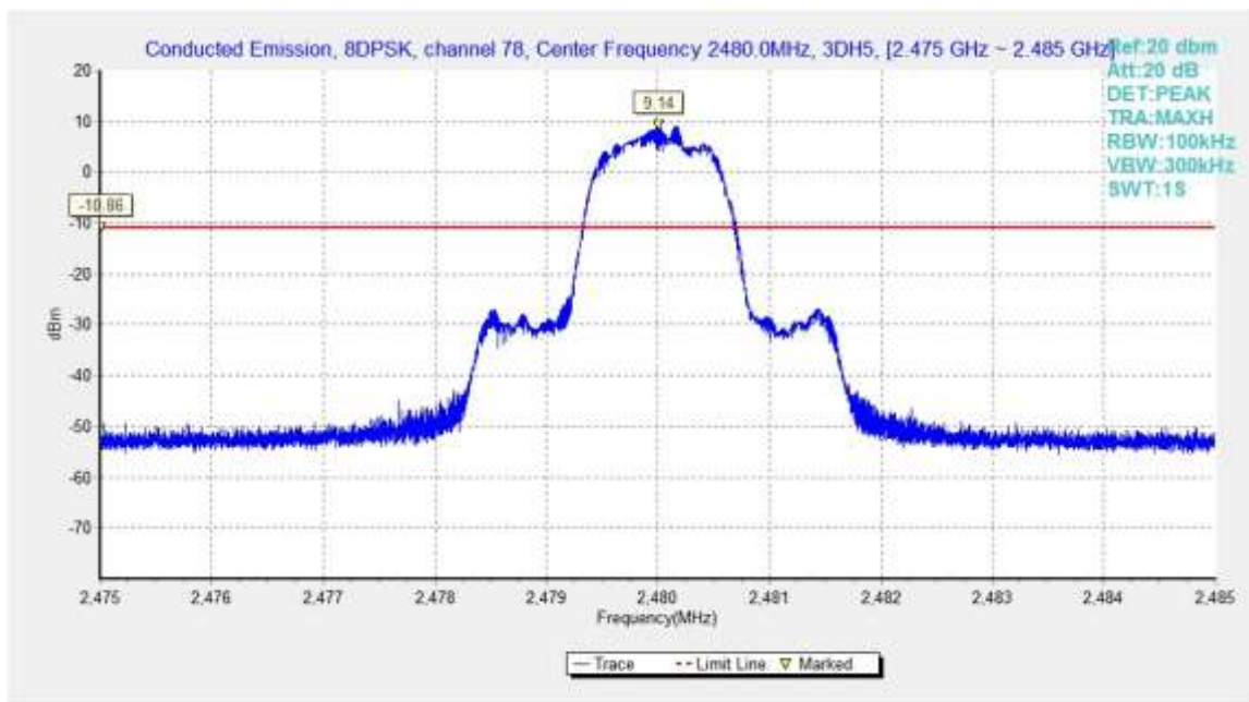
Fig.67. Conducted spurious emission: 8DPSK, Channel 78, 2480MHz
