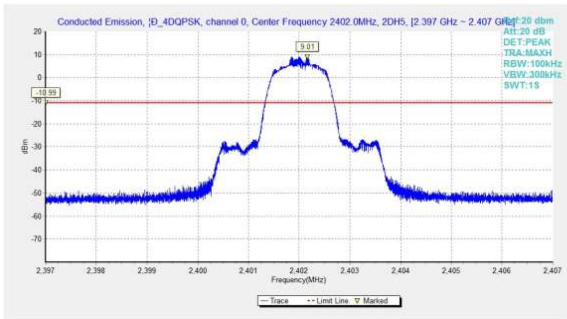
Fig.42. Conducted spurious emission: \pi/4 DQPSK, Channel 0, 2402MHz
