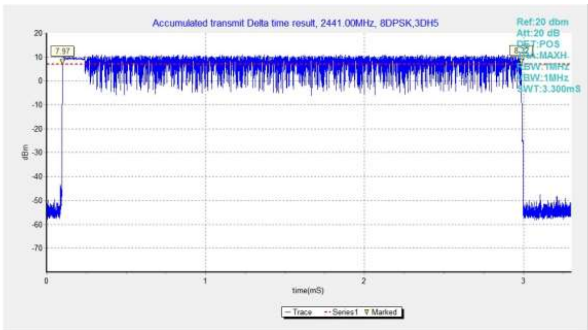
Fig.88. Time of occupancy (Dwell Time): Channel 39, Packet 3-DH5
