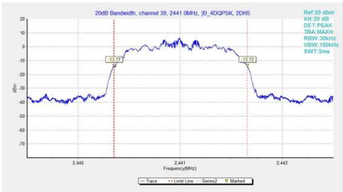
Fig.94. 20dB Bandwidth: \pi/4 DQPSK, Channel 39
