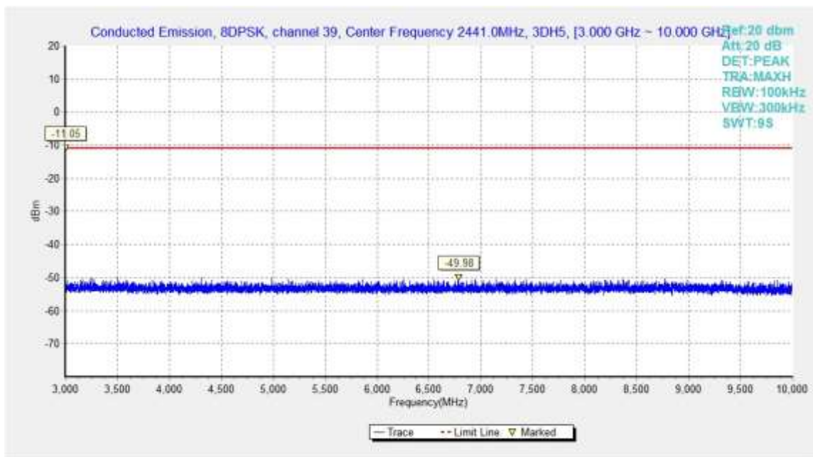
Fig.65. Conducted spurious emission: 8DPSK, Channel 39, 3GHz - 10GHz
