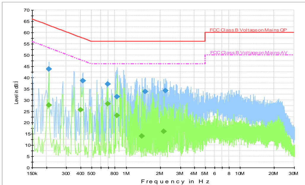
Fig. B11.2 AC Powerline Conducted Emission-802.11a (EUT4 + AE2-2 + AE1-3)
