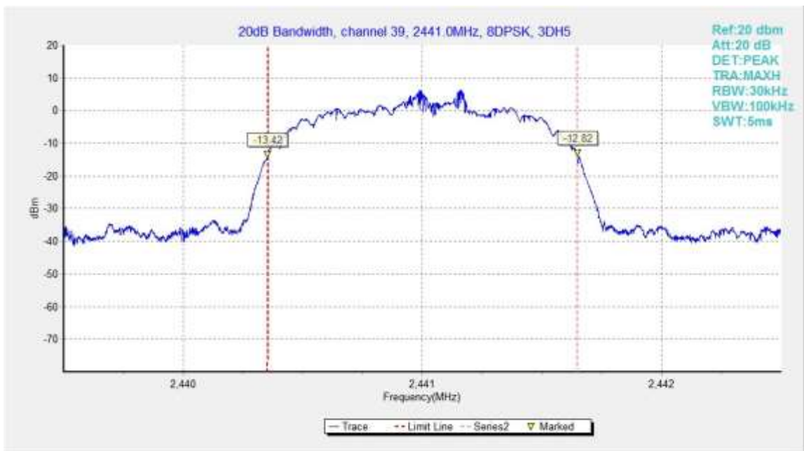
Fig.97. 20dB Bandwidth: 8DPSK, Channel 39
