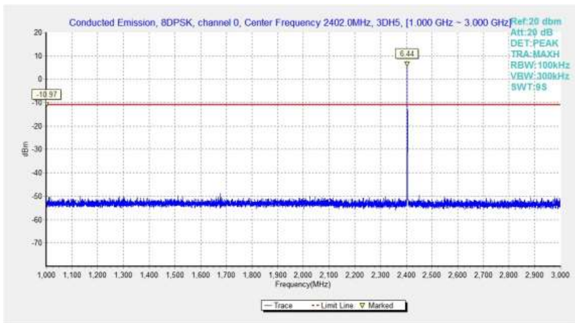
Fig.59. Conducted spurious emission: 8DPSK, Channel 0, 1GHz - 3GHz
