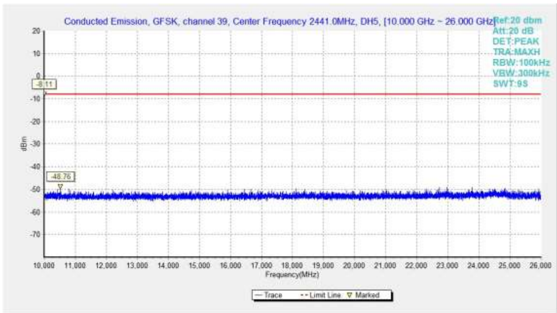
Fig.36. Conducted spurious emission: GFSK, Channel 39, 10GHz – 26GHz
