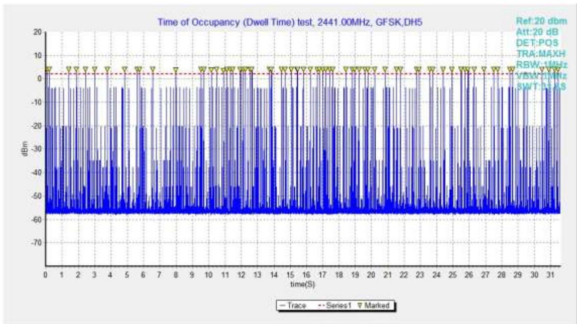
Fig.77. Number of Transmissions Measurement: Channel 39,Packet DH5
