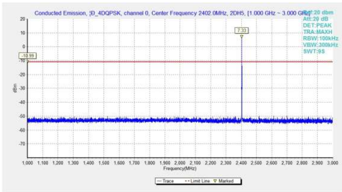
Fig.44. Conducted spurious emission: \pi/4 DQPSK, Channel 0, 1GHz - 3GHz
