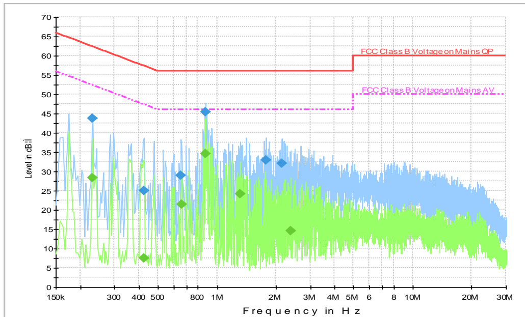
Fig. B11.1 AC Powerline Conducted Emission-Idle (EUT3 + AE2-1 + AE1-3)
