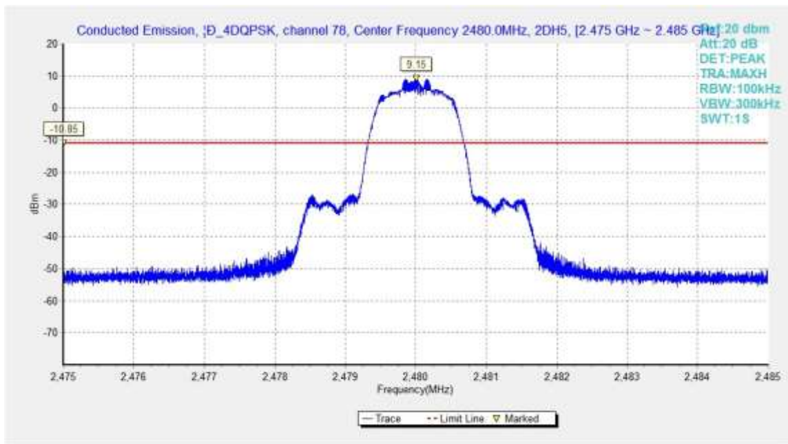
Fig.52. Conducted spurious emission: \pi/4 DQPSK, Channel 78, 2480MHz
