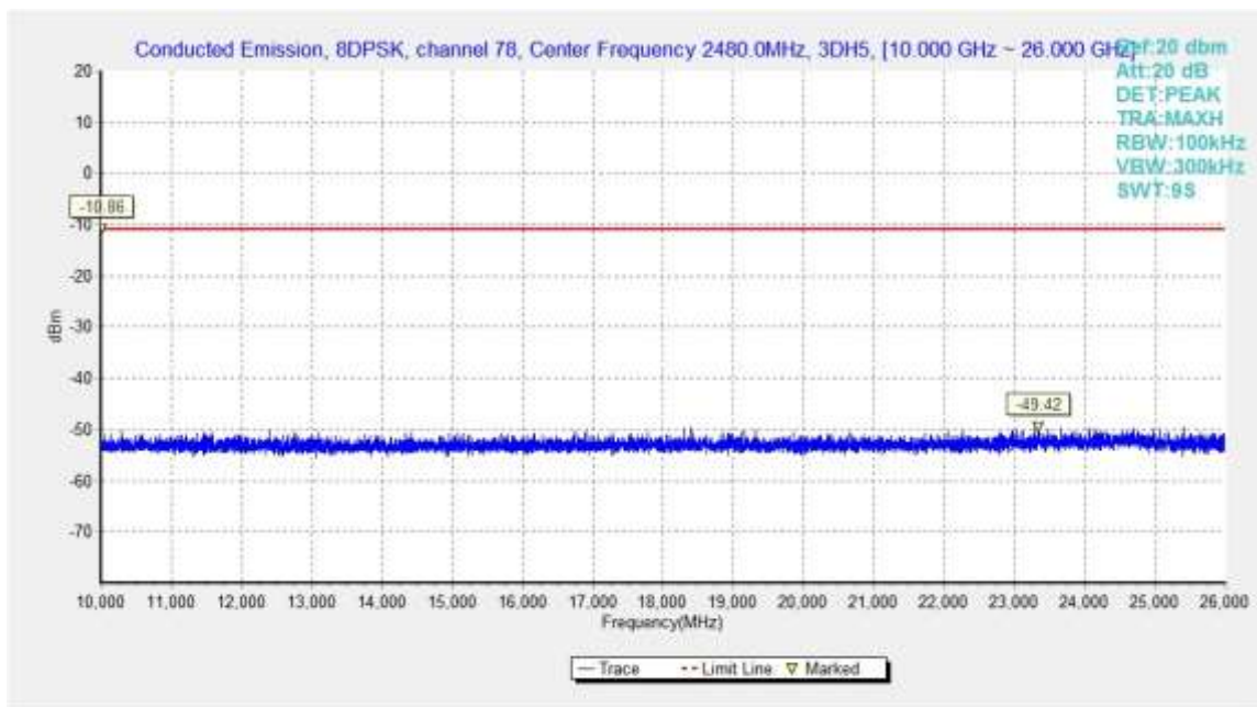
Fig.71. Conducted spurious emission: 8DPSK, Channel 78, 10GHz - 26GHz
