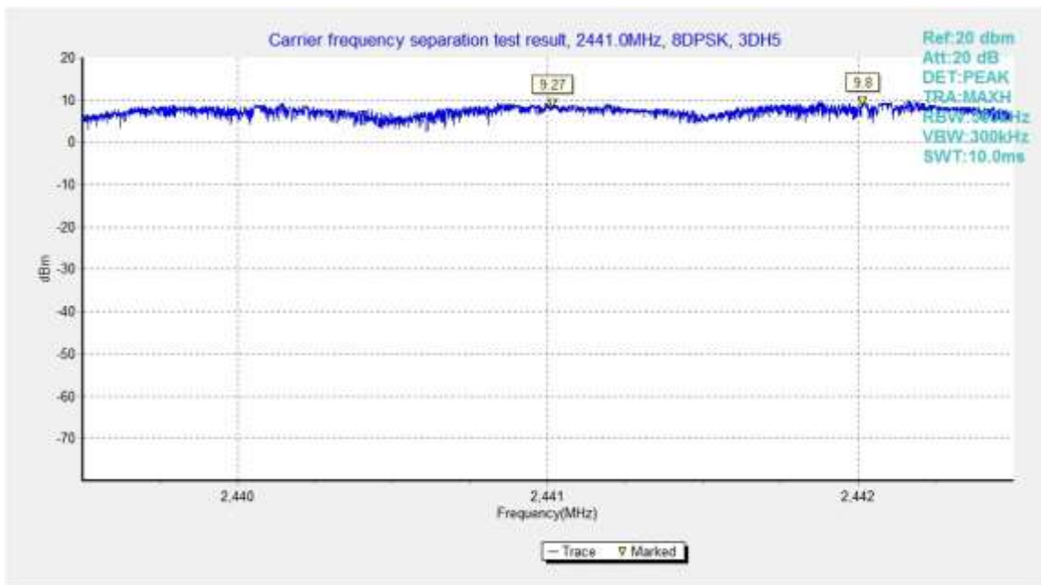
Fig.101. Carrier frequency separation measurement: 8DPSK, Channel 39
