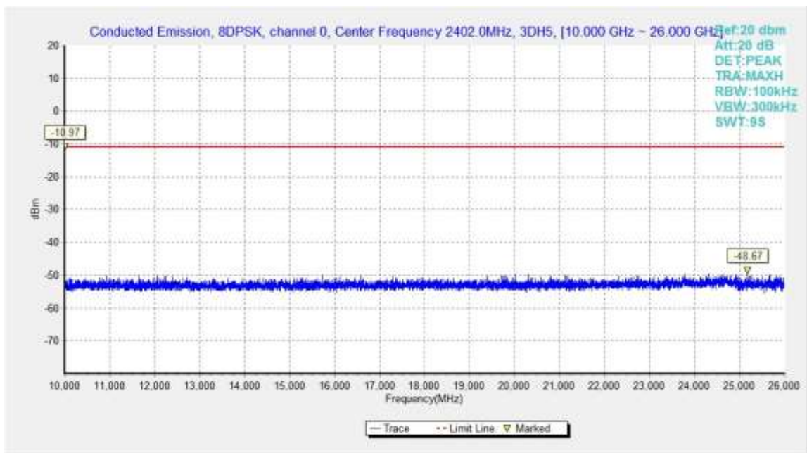
Fig.61. Conducted spurious emission: 8DPSK, Channel 0, 10GHz - 26GHz
