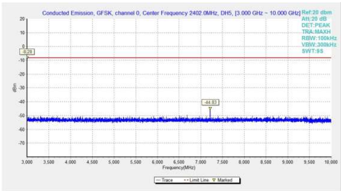
Fig.30. Conducted spurious emission: GFSK, Channel 0, 3GHz - 10GHz
