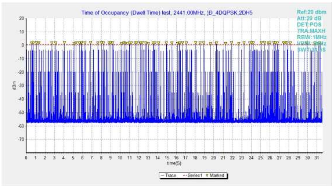
Fig.83. Number of Transmissions Measurement: Channel 39,Packet 2-DH5
