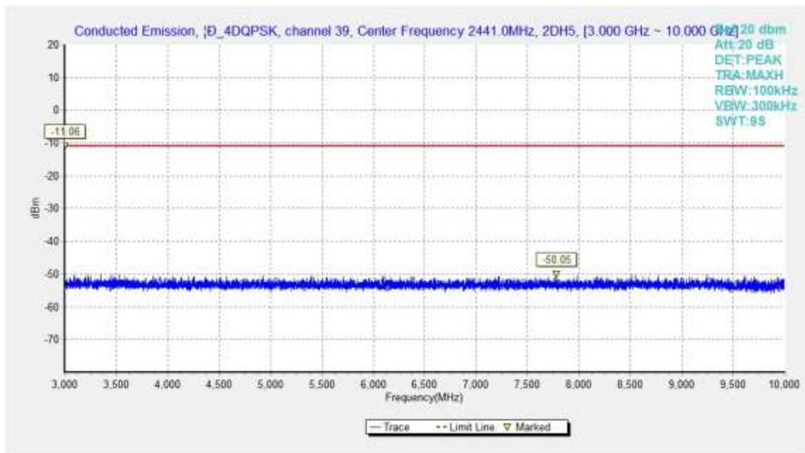
Fig.50. Conducted spurious emission: \pi/4 DQPSK, Channel 39, 3GHz - 10GHz
