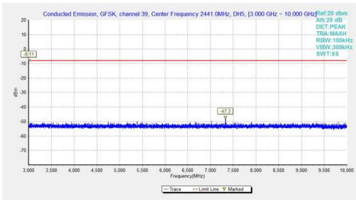
Fig.35. Conducted spurious emission: GFSK, Channel 39, 3GHz – 10GHz
