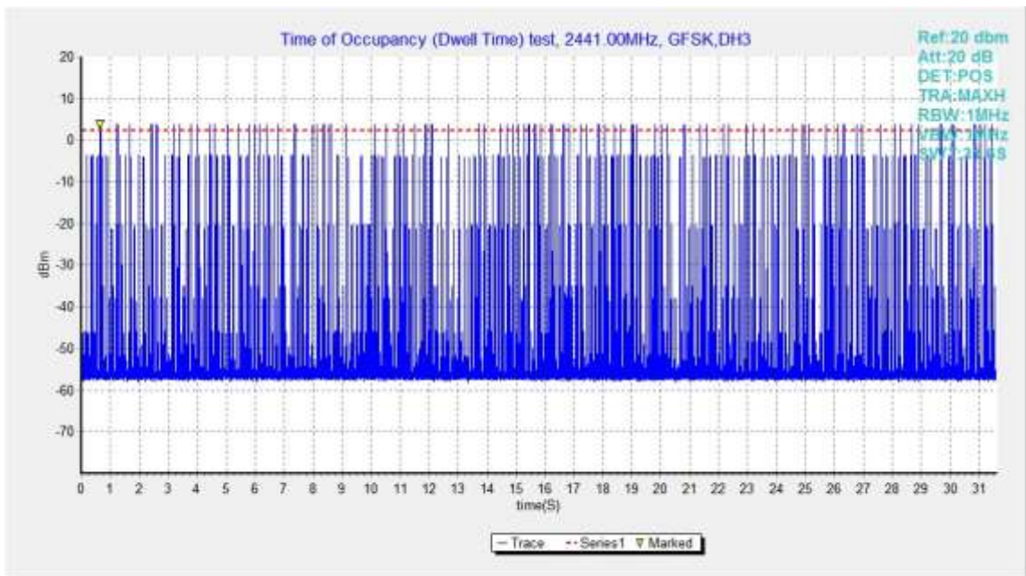
Fig.75. Number of Transmissions Measurement: Channel 39,Packet DH3
