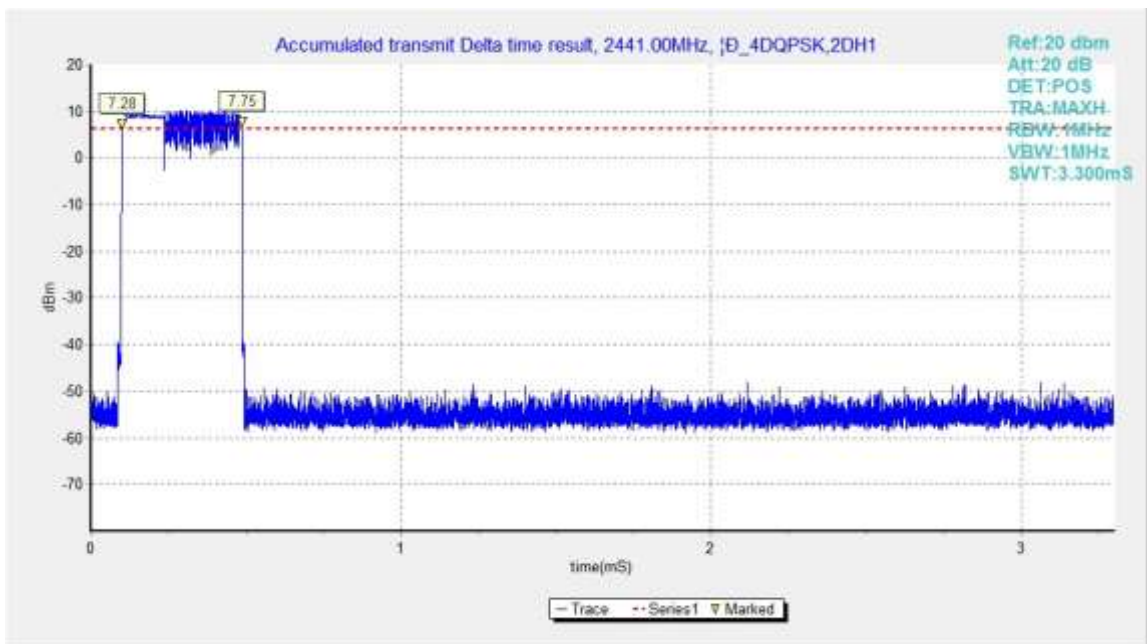
Fig.78. Time of occupancy (Dwell Time): Channel 39, Packet 2-DH1
