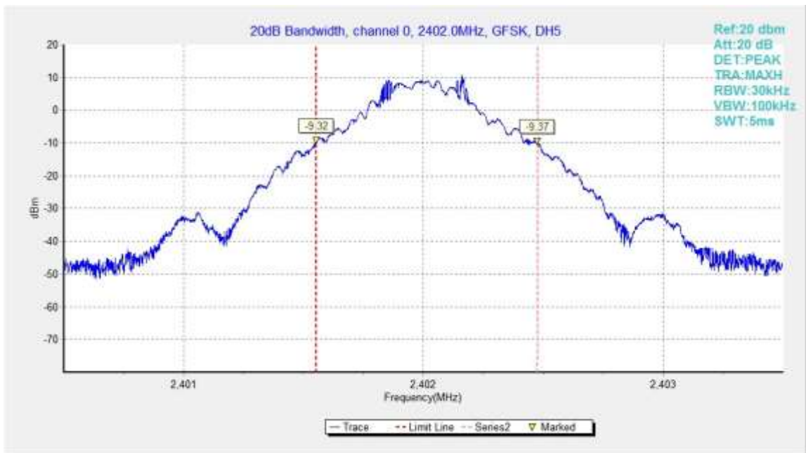
Fig.90. 20dB Bandwidth: GFSK, Channel 0
