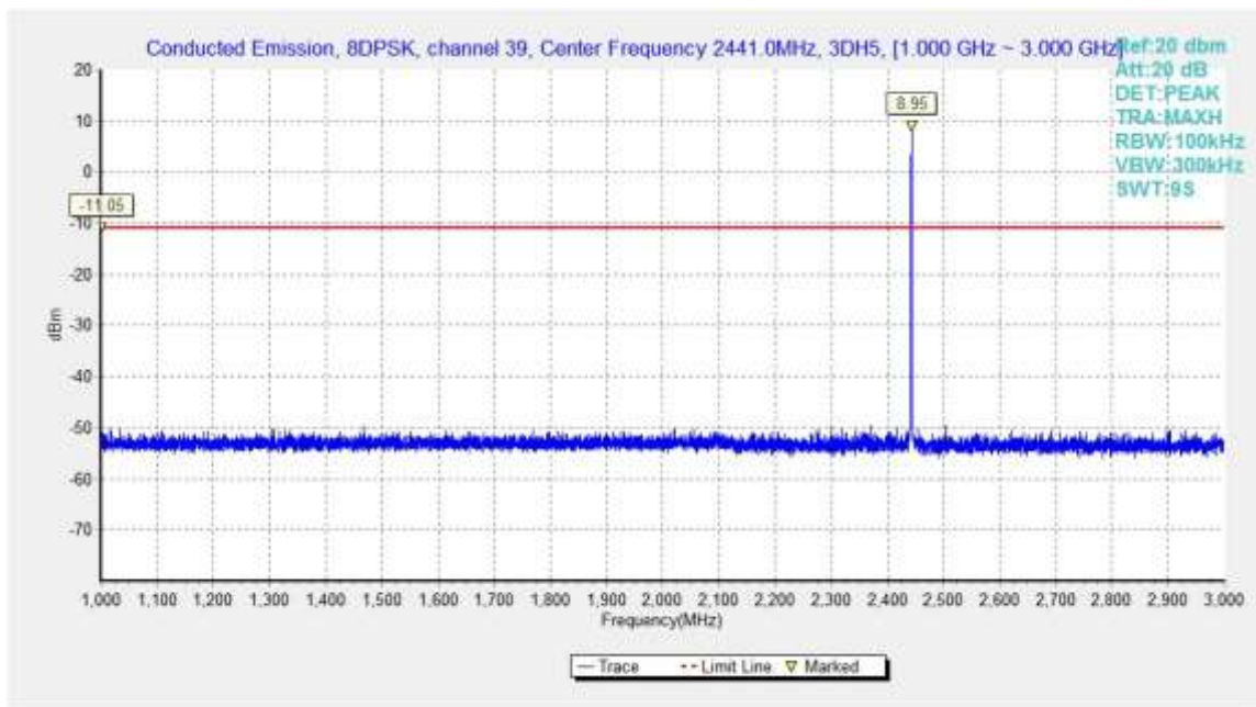
Fig.64. Conducted spurious emission: 8DPSK, Channel 39, 1GHz - 3GHz
