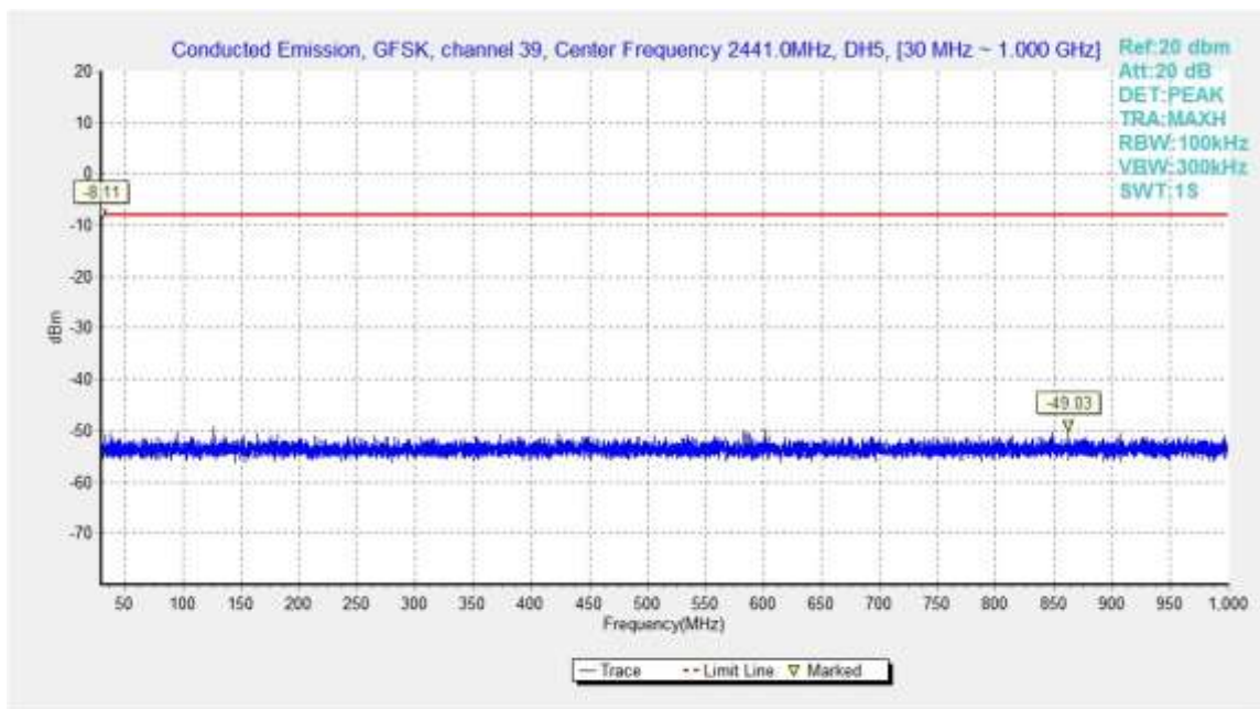
Fig.33. Conducted spurious emission: GFSK, Channel 39, 30MHz - 1GHz
