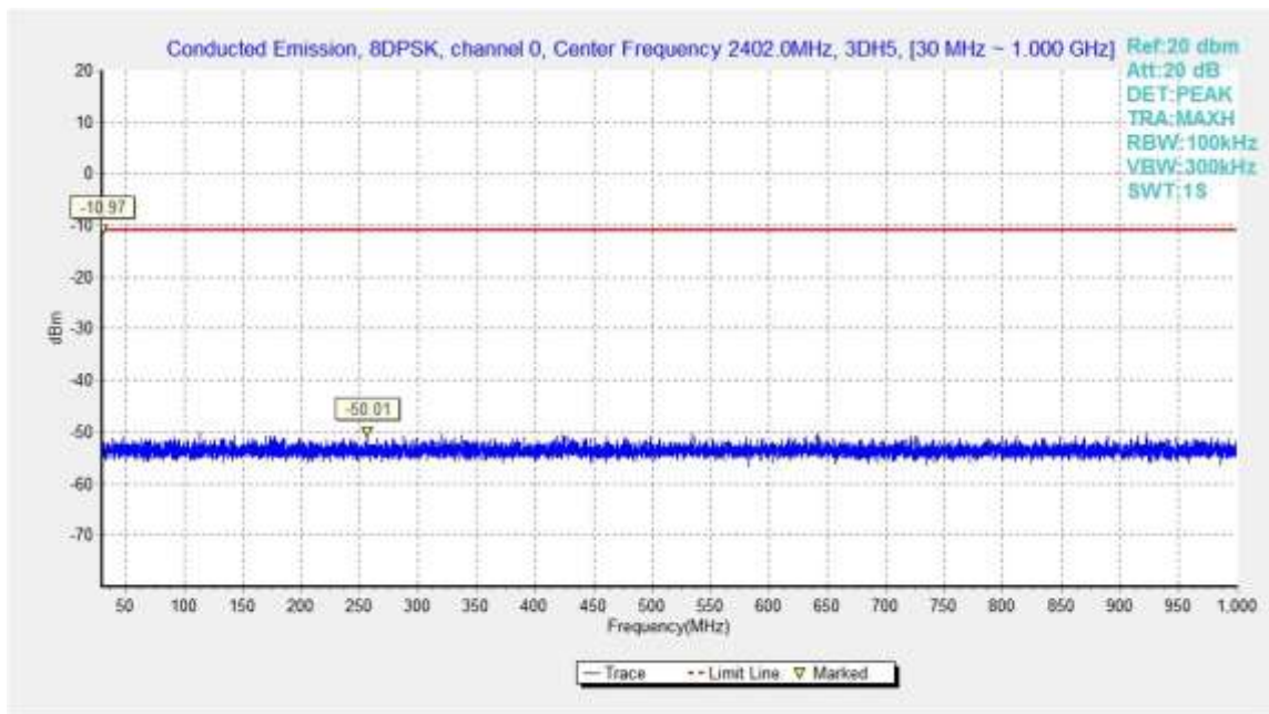
Fig.58. Conducted spurious emission: 8DPSK, Channel 0, 30MHz - 1GHz
