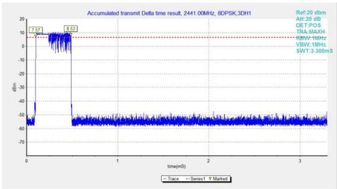
Fig.84. Time of occupancy (Dwell Time): Channel 39, Packet 3-DH1
