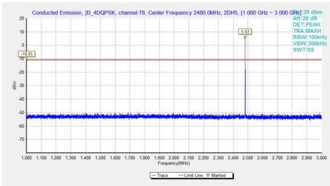
Fig.54. Conducted spurious emission: \pi/4 DQPSK, Channel 78, 1GHz - 3GHz
