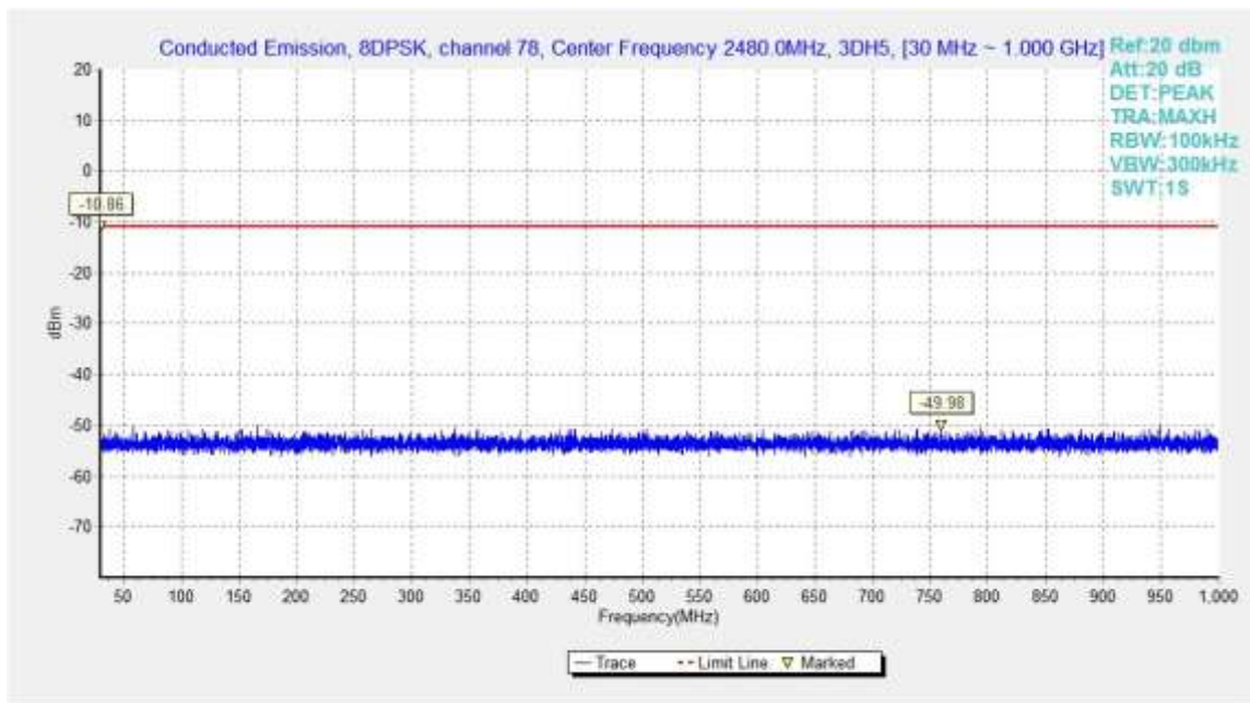
Fig.68. Conducted spurious emission: 8DPSK, Channel 78, 30MHz - 1GHz
