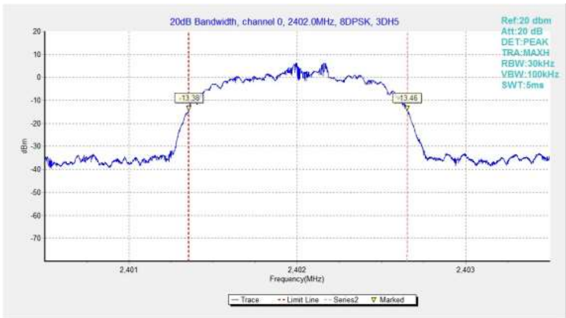
Fig.96. 20dB Bandwidth: 8DPSK, Channel 0
