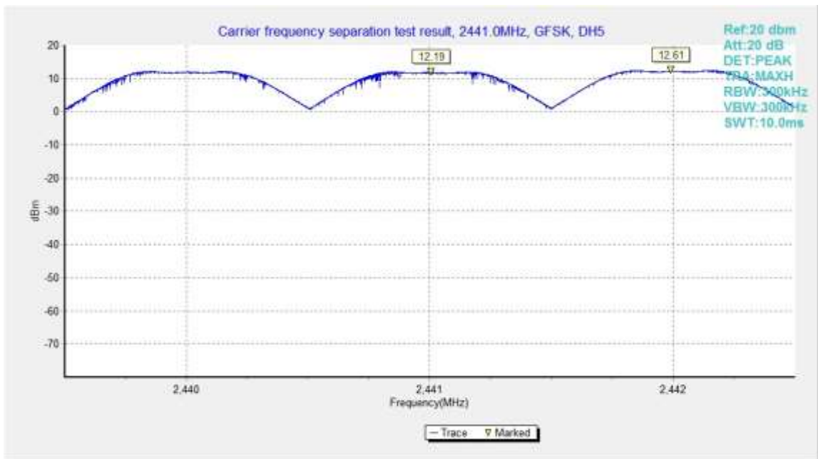
Fig.99. Carrier frequency separation measurement: GFSK, Channel 39
