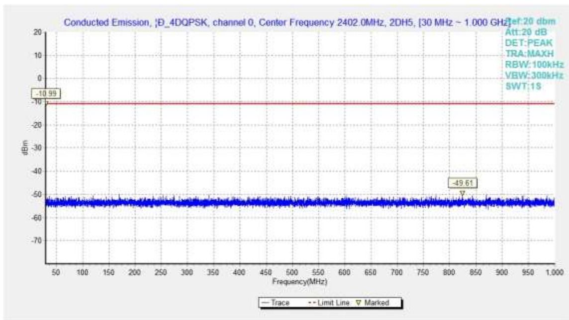
Fig.43. Conducted spurious emission: \pi/4 DQPSK, Channel 0, 30MHz - 1GHz
