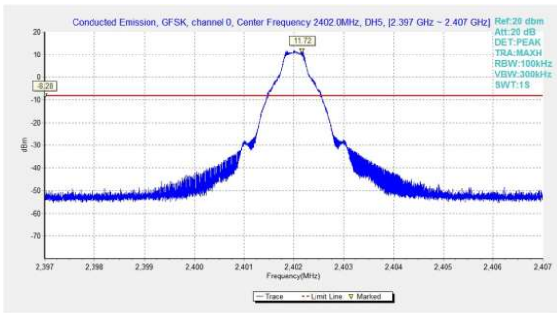
Fig.27. Conducted spurious emission: GFSK, Channel 0, 2402MHz
