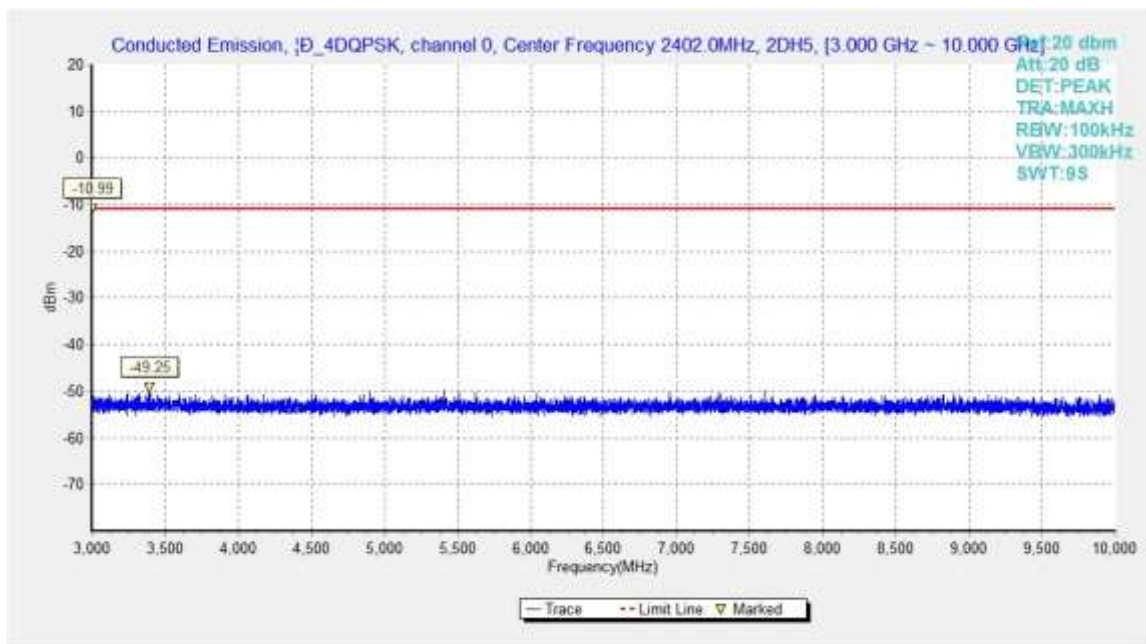
Fig.45. Conducted spurious emission: \pi/4 DQPSK, Channel 0, 3GHz - 10GHz
