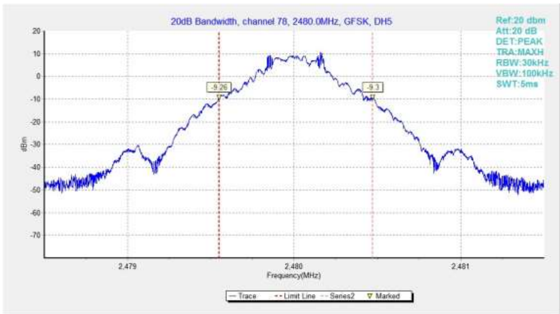
Fig.92. 20dB Bandwidth: GFSK, Channel 78
