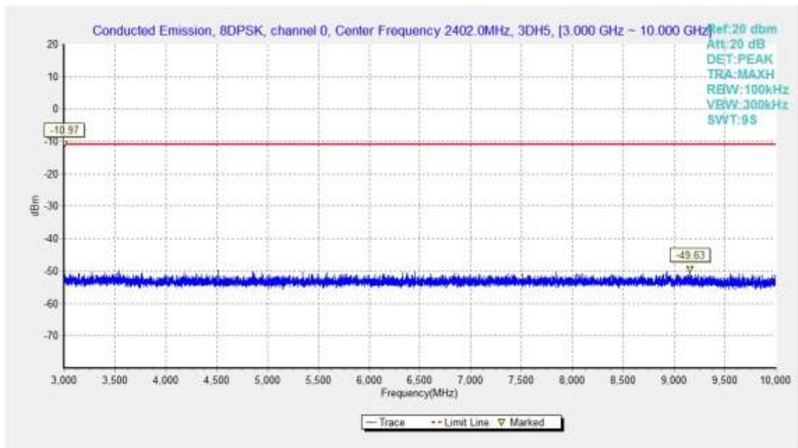
Fig.60. Conducted spurious emission: 8DPSK, Channel 0, 3GHz - 10GHz
