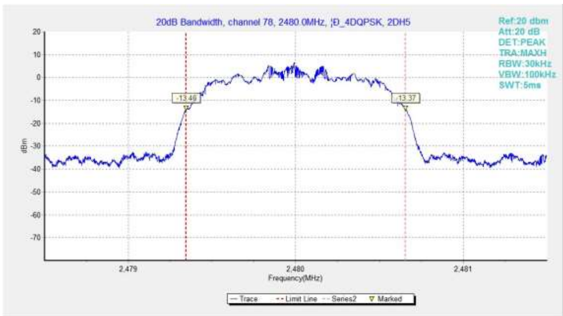
Fig.95. 20dB Bandwidth: \pi/4 DQPSK, Channel 78
