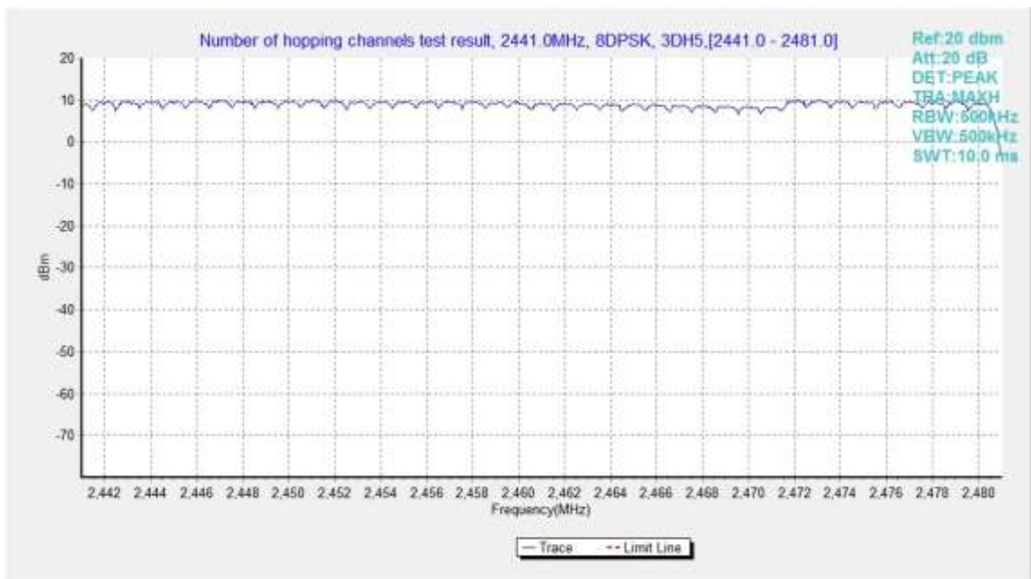
Fig.107. Number of hopping frequencies: 8DPSK, Channel 40 - 78
