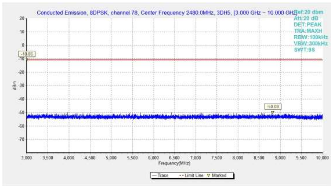
Fig.70. Conducted spurious emission: 8DPSK, Channel 78, 3GHz - 10GHz
