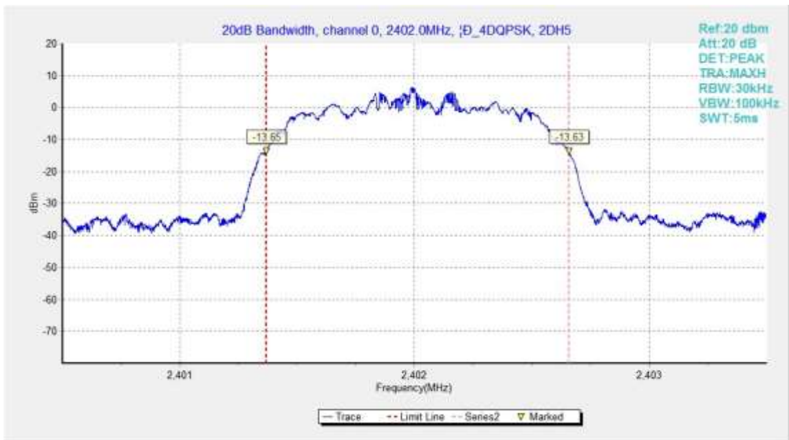
Fig.93. 20dB Bandwidth: \pi/4 DQPSK, Channel 0
