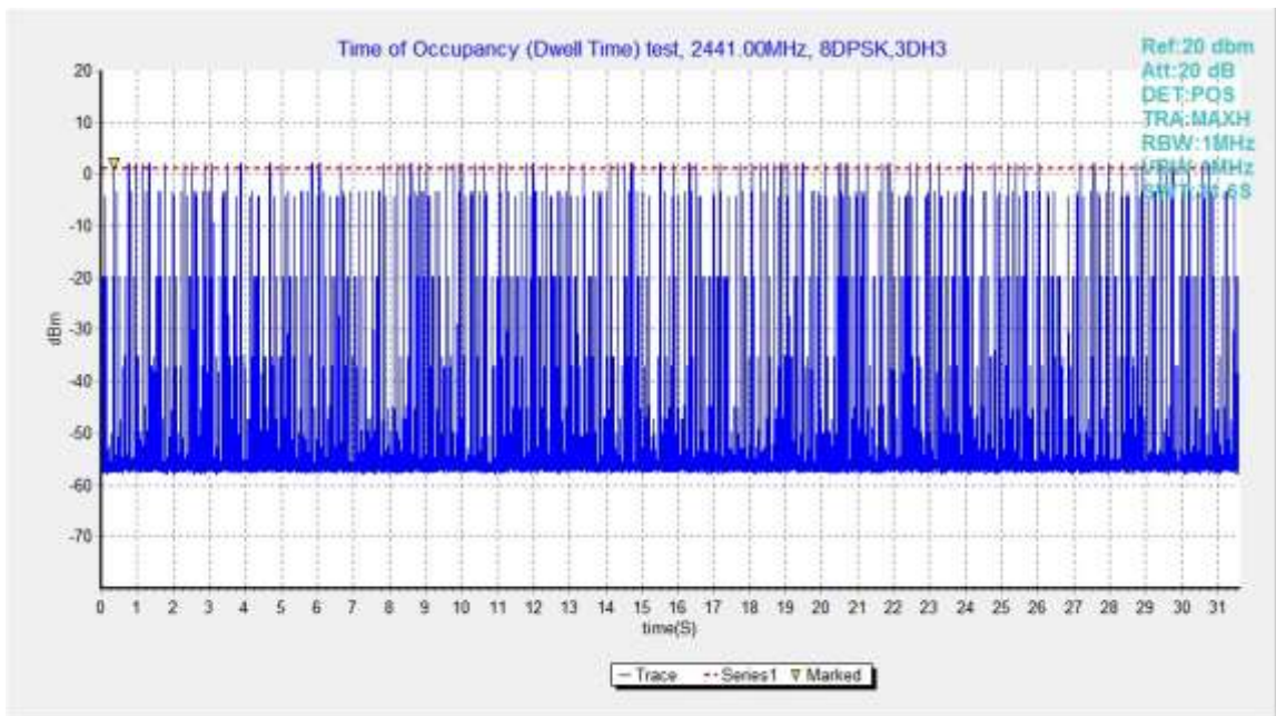
Fig.87. Number of Transmissions Measurement: Channel 39,Packet 3-DH3
