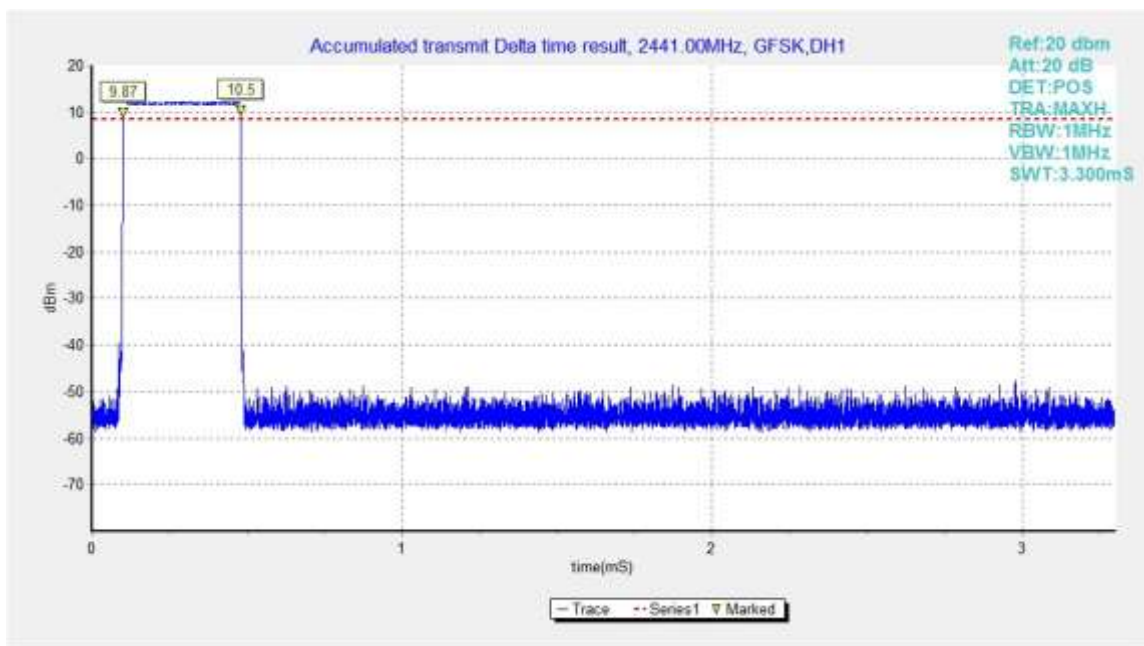
Fig.72. Time of occupancy (Dwell Time): Channel 39, Packet DH1
