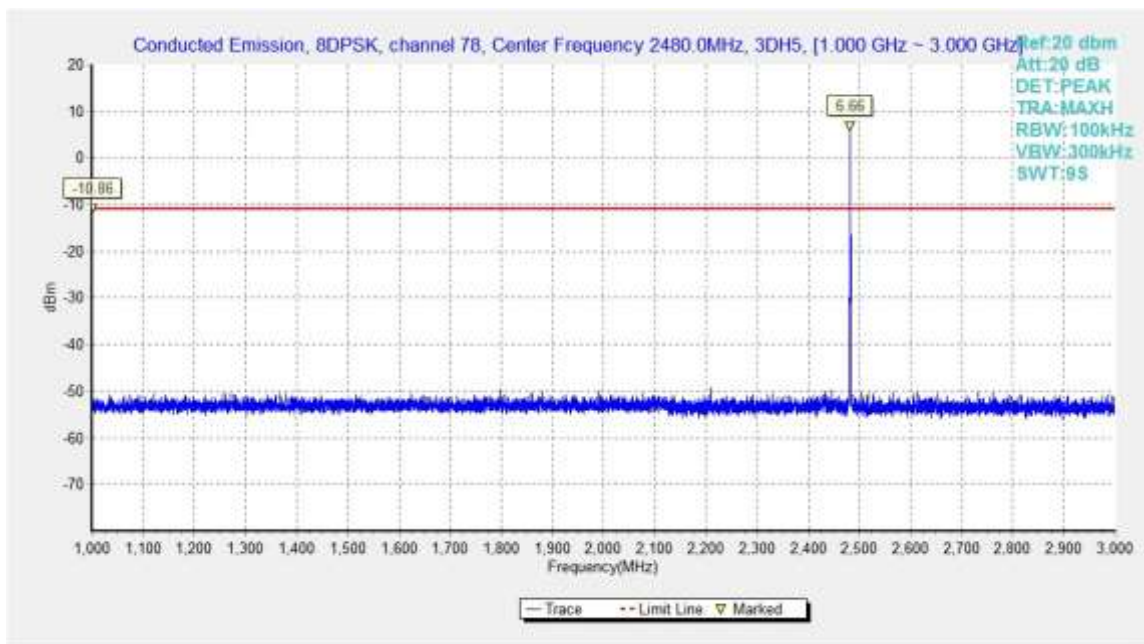
Fig.69. Conducted spurious emission: 8DPSK, Channel 78, 1GHz - 3GHz
