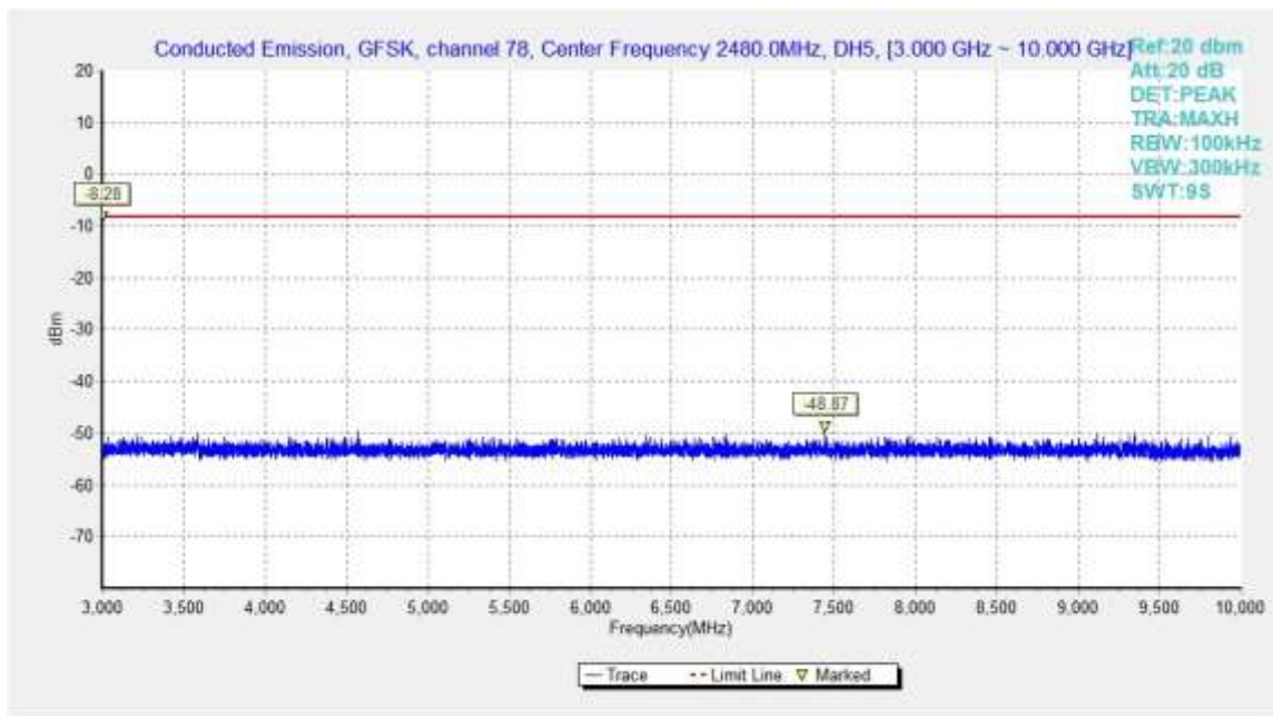
Fig.40. Conducted spurious emission: GFSK, Channel 78, 3GHz - 10GHz
