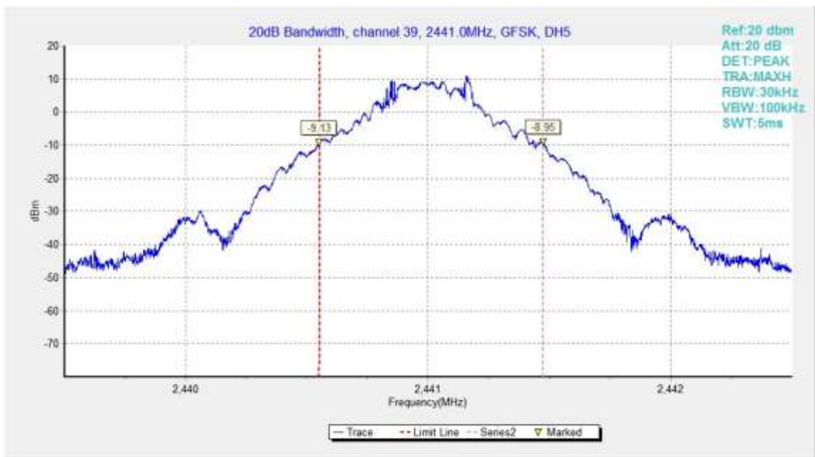
Fig.91. 20dB Bandwidth: GFSK, Channel 39
