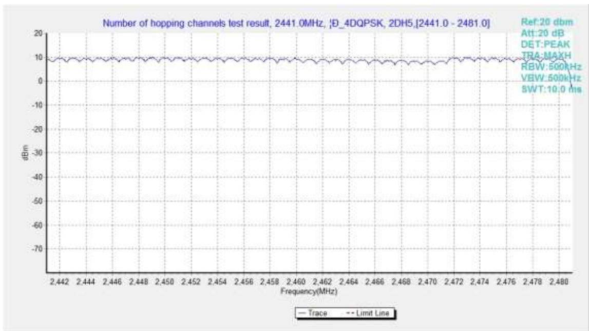
Fig.105. Number of hopping frequencies: \pi/4 DQPSK, Channel 40 - 78
