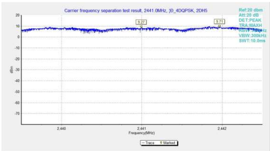
Fig.100. Carrier frequency separation measurement: \pi/4 DQPSK, Channel 39
