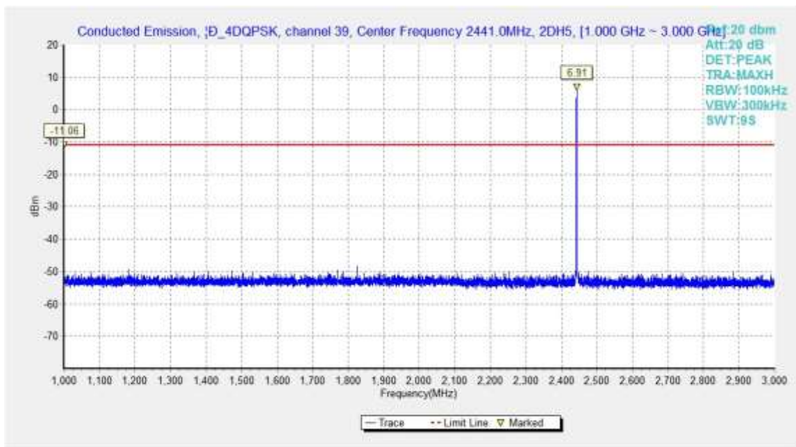
Fig.49. Conducted spurious emission: \pi/4 DQPSK, Channel 39, 1GHz - 3GHz
