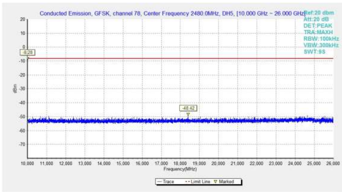
Fig.41. Conducted spurious emission: GFSK, Channel 78, 10GHz - 26GHz
