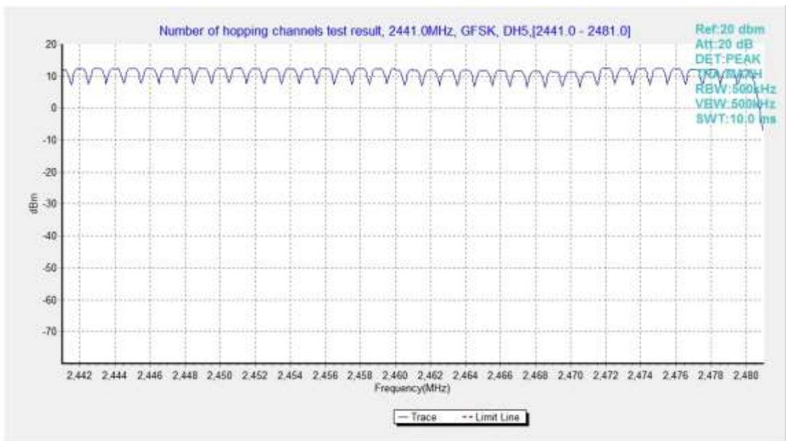
Fig.103. Number of hopping frequencies: GFSK, Channel 40 - 78
