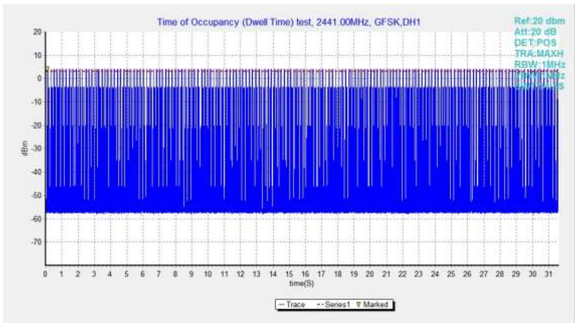
Fig.73. Number of Transmissions Measurement: Channel 39,Packet DH1
