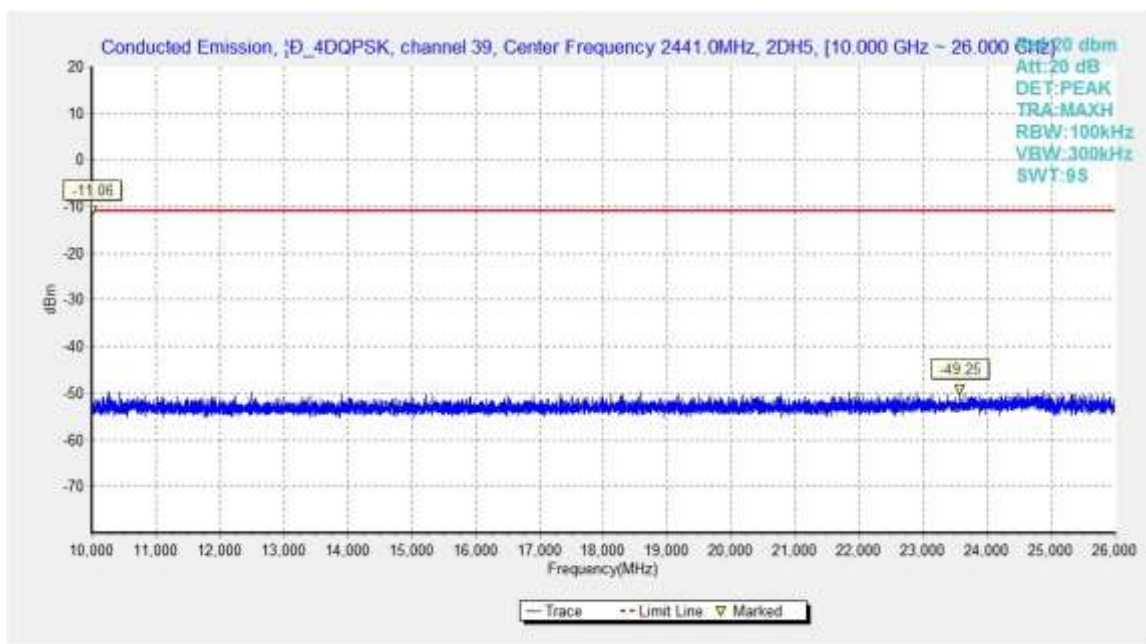
Fig.51. Conducted spurious emission: \pi/4 DQPSK, Channel 39, 10GHz – 26GHz
