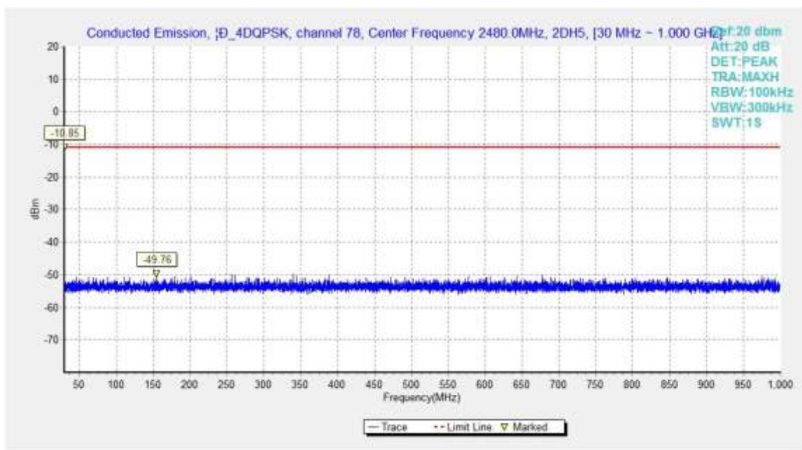
Fig.53. Conducted spurious emission: \pi/4 DQPSK, Channel 78, 30MHz - 1GHz
