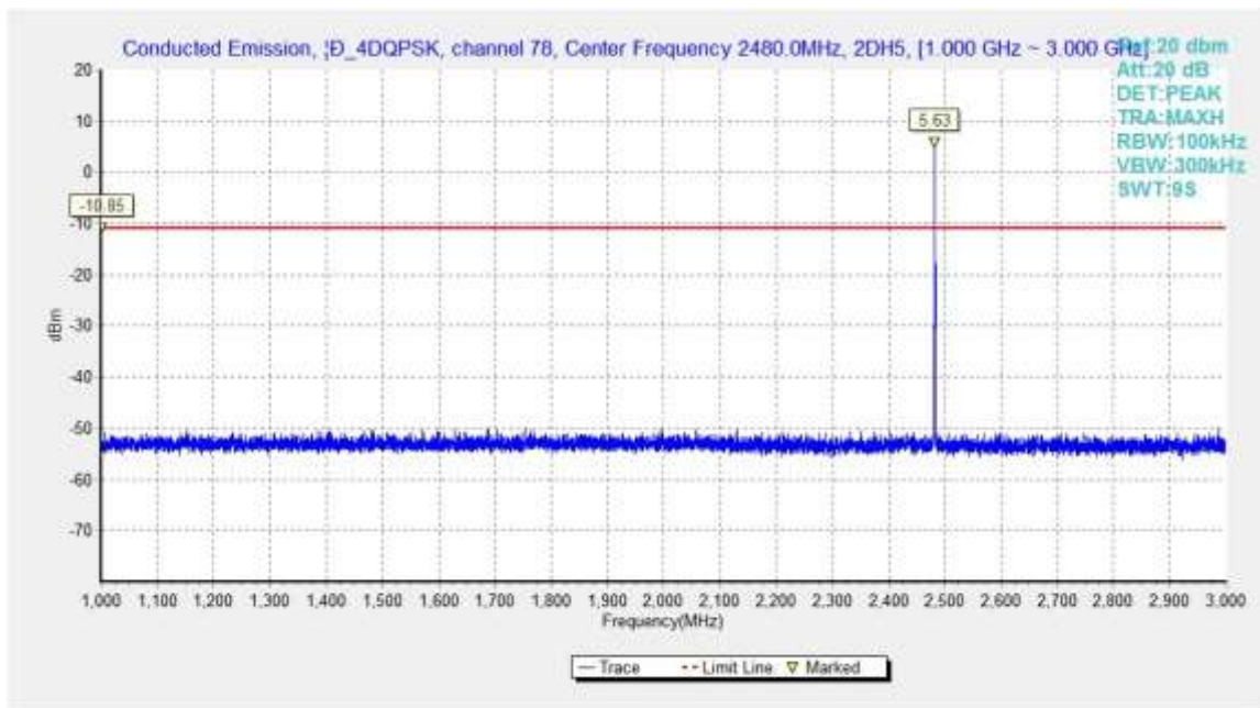
Fig.54. Conducted spurious emission: \pi/4 DQPSK, Channel 78, 1GHz - 3GHz
