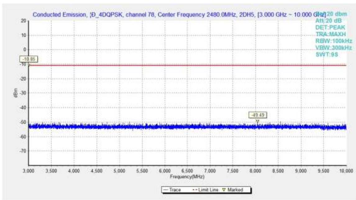
Fig.55. Conducted spurious emission: \pi/4 DQPSK, Channel 78, 3GHz - 10GHz
