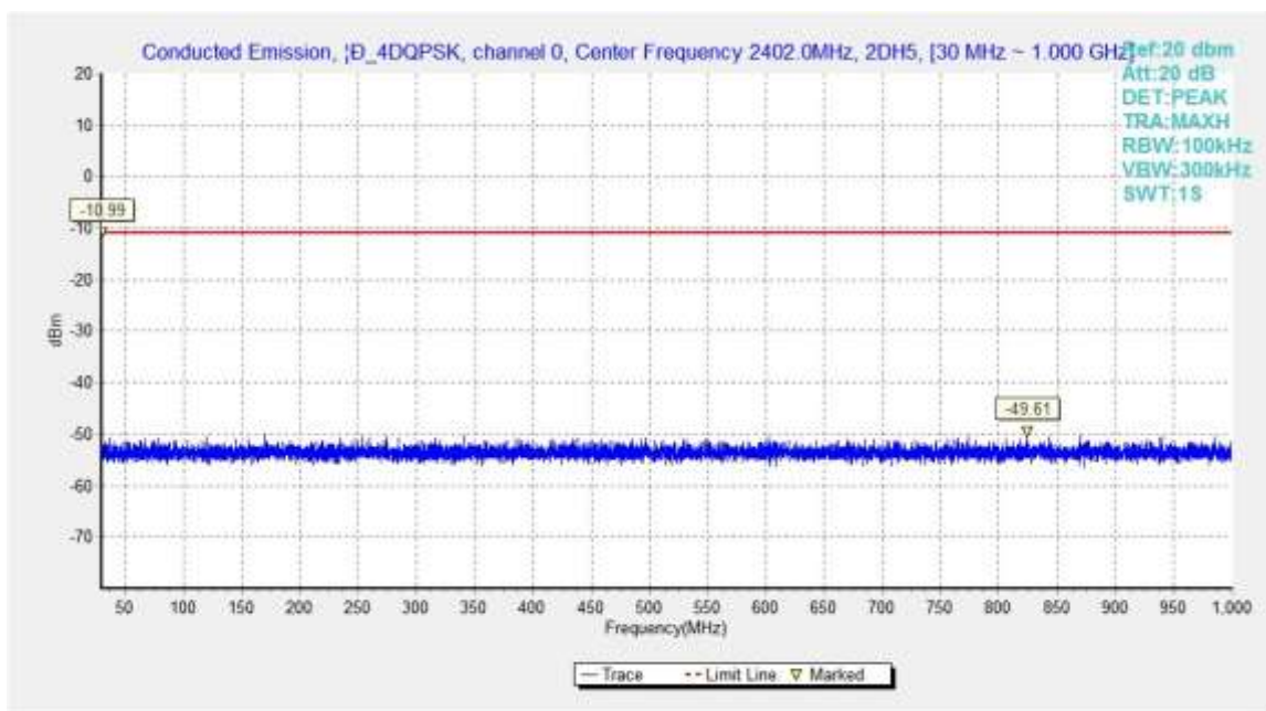
Fig.43. Conducted spurious emission: \pi/4 DQPSK, Channel 0, 30 MHz - 1 GHz
