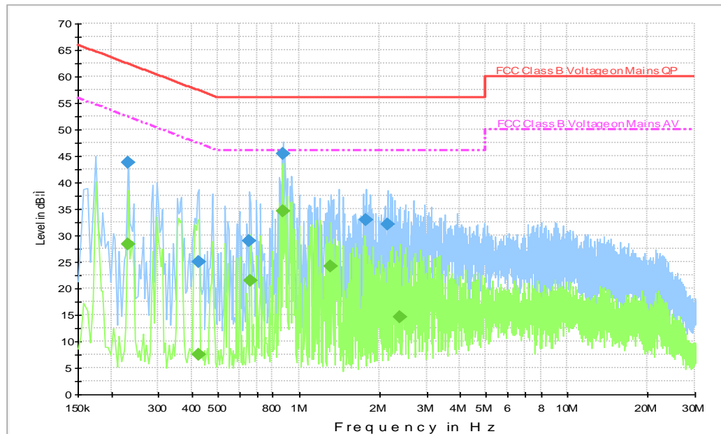
Fig. B11.1 AC Powerline Conducted Emission-Iidle (EUT3 + AE2-1 + AE1-3)
