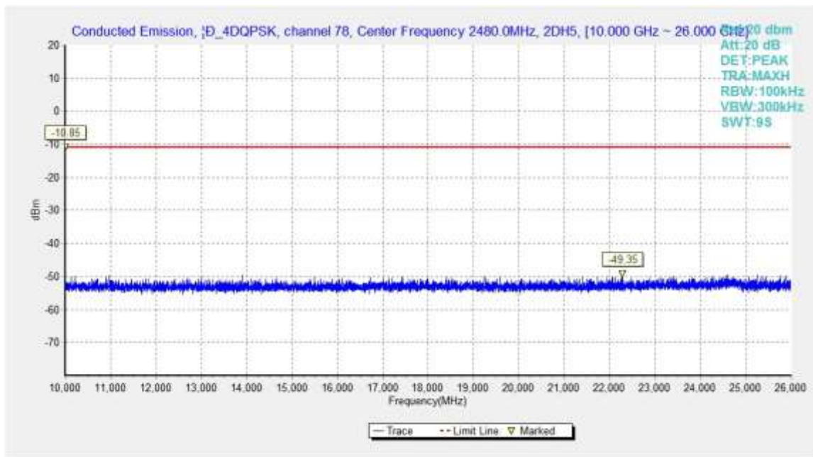
Fig.56. Conducted spurious emission: \pi/4 DQPSK, Channel 78, 10GHz - 26GHz
