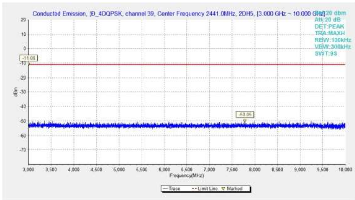
Fig.50. Conducted spurious emission: \pi/4 DQPSK, Channel 39, 3GHz - 10GHz
