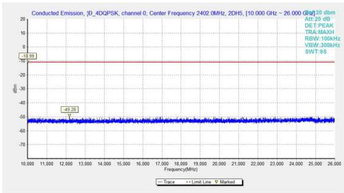
Fig.46. Conducted spurious emission: \pi/4 DQPSK, Channel 0, 10GHz - 26GHz
