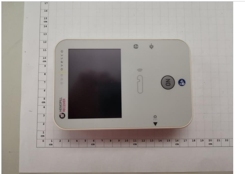
Photograph 7: EUT 3_Front side view
