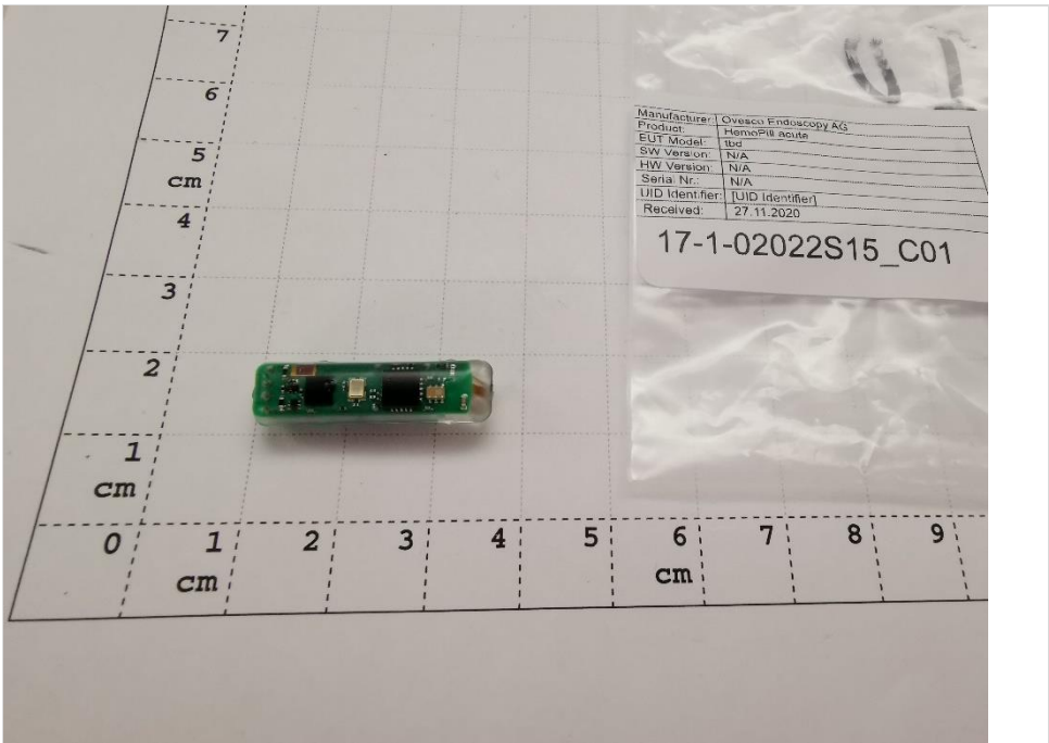
Photograph 6: EUT 2_Bottom side view
