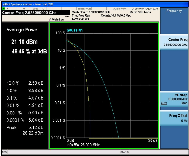
Band7-20MHz-QPSK-21100-1RB#0-PASS
