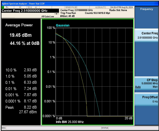
Band7-20MHz-16QAM-20850-100RB#0-PASS
