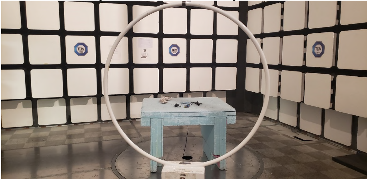
Figure 1 – Radiated Emissions Setup – Photo 1
