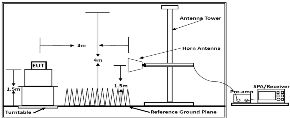
Above 1GHz
