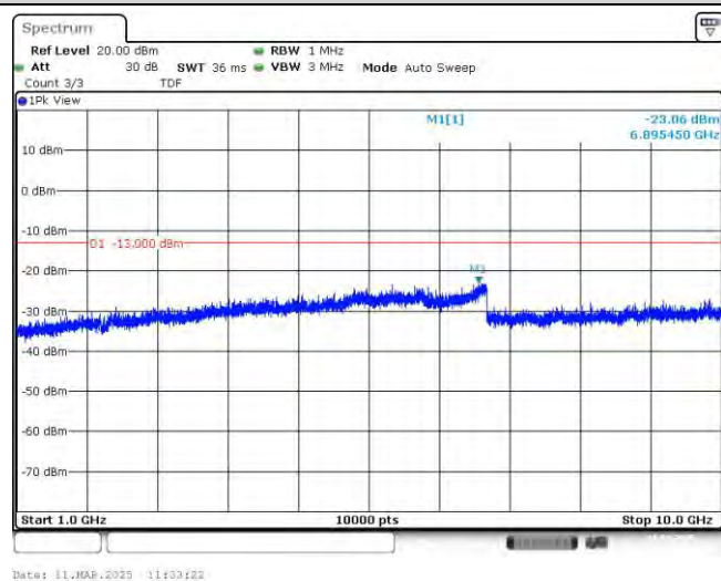
Band26-15MHz-16QAM-26965-75RB#0-Range2:1000~10000MHz
