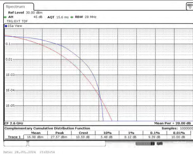
Band41-20MHz-16QAM-41490-100RB#0
