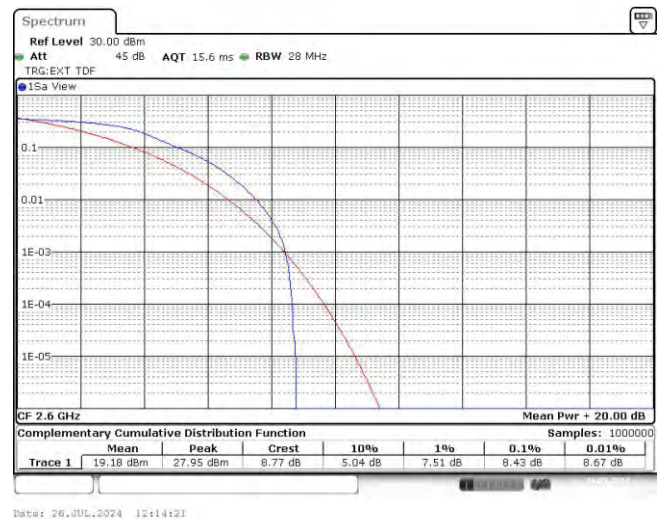
Band41-5MHz-QPSK-41565-25RB#0
