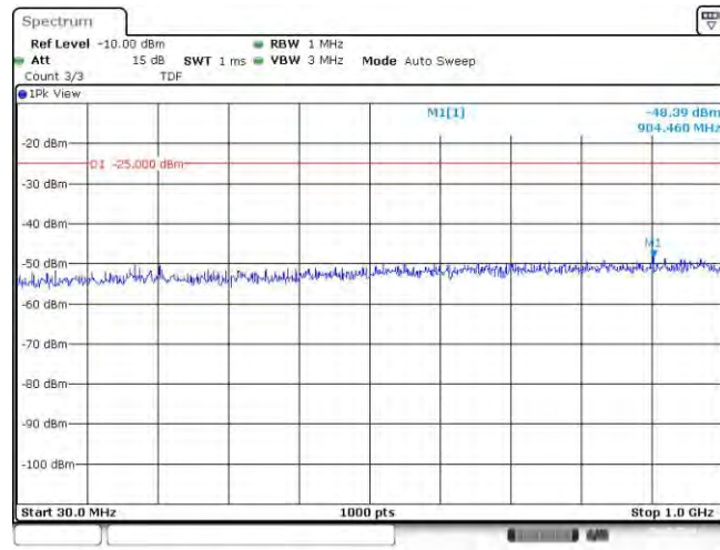
Band41-5MHz-QPSK-39675-25RB#0-Range1:30~1000MHz
