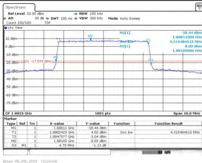
Band25-5MHz-16QAM-26665-25RB#0
