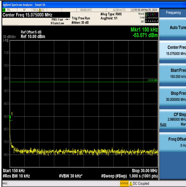
Band5_1.4MHz_16QAM_20525_1RB#0_0.15~30_0.15~30
