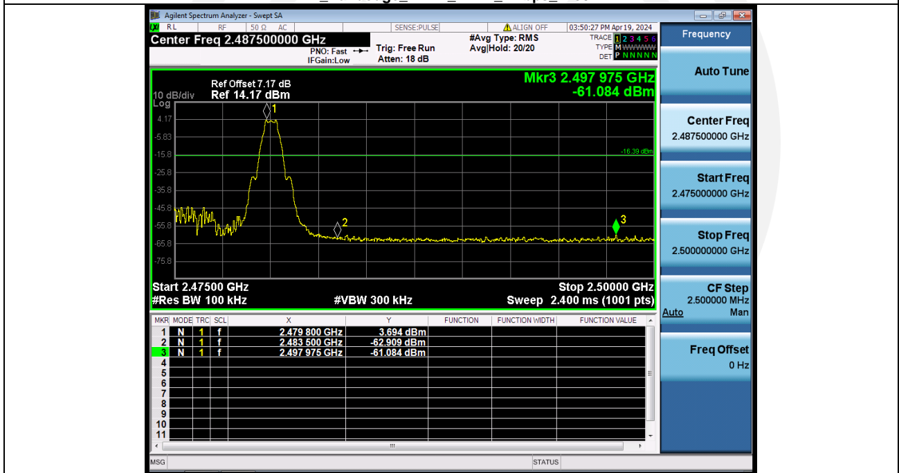
2_Bandedge_NVNT_ANT1_1Mbps_2480
