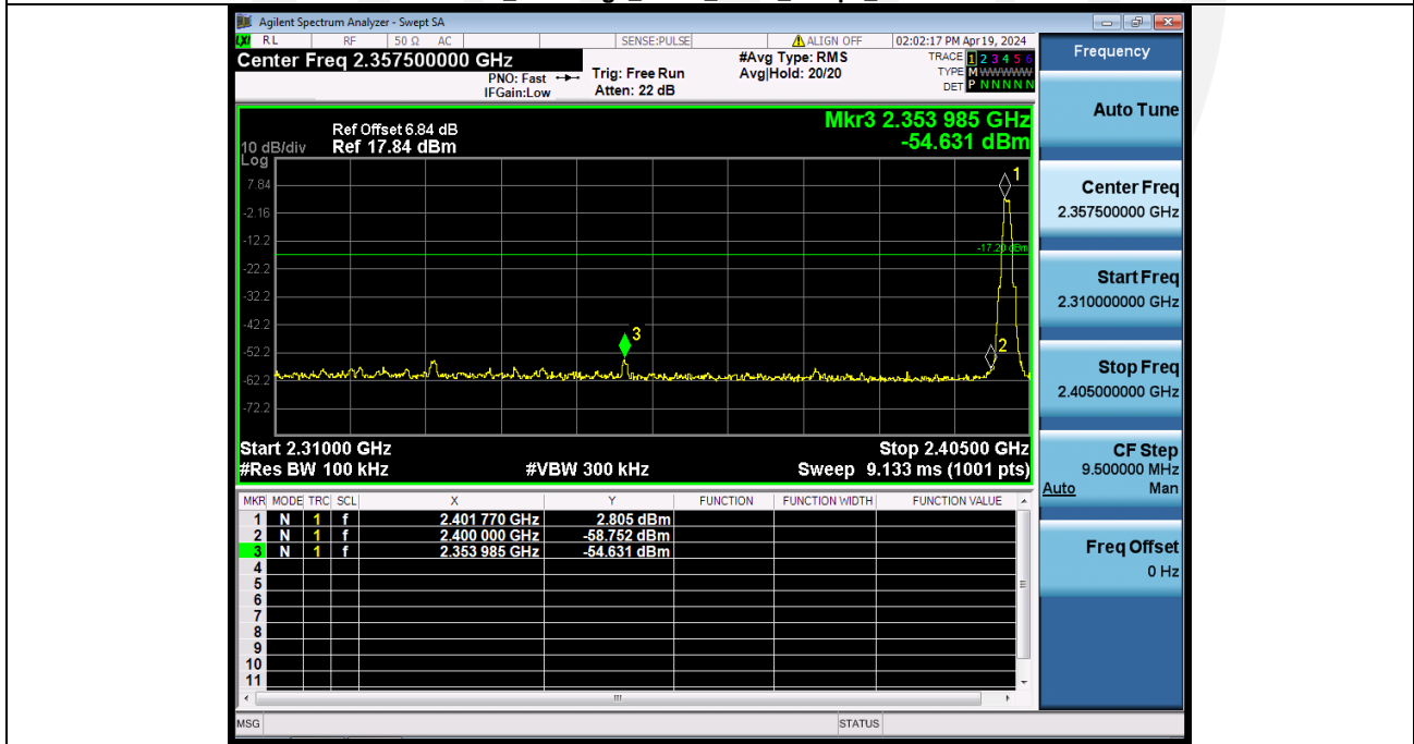
2_Bandedge_NVNT_ANT1_1Mbps_2402
