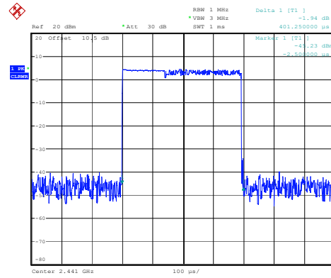
2DH1_Hopping 0.401ms
