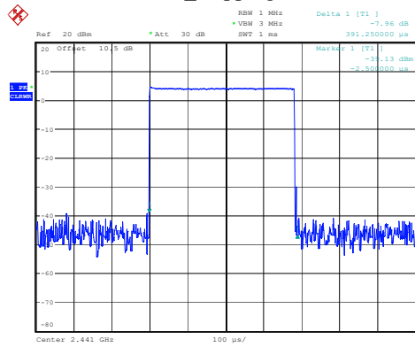
DH1_Hopping 0.391ms
