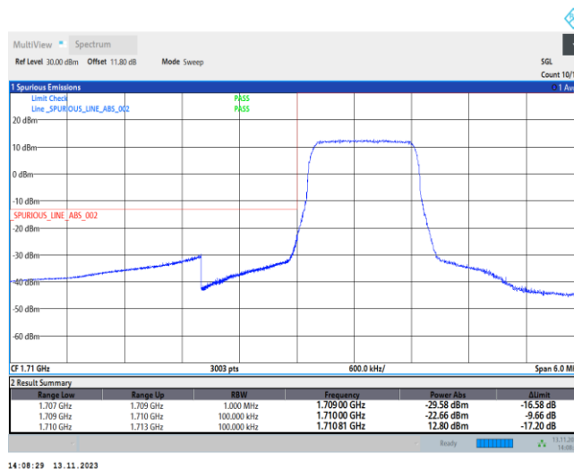
Band4-1.4MHz-QPSK-19957-6RB#0
