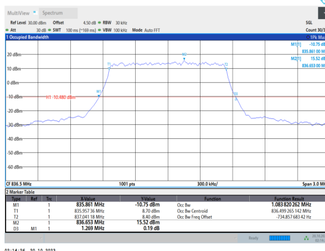
Band5-1.4MHz-16QAM-20525-6RB#0
