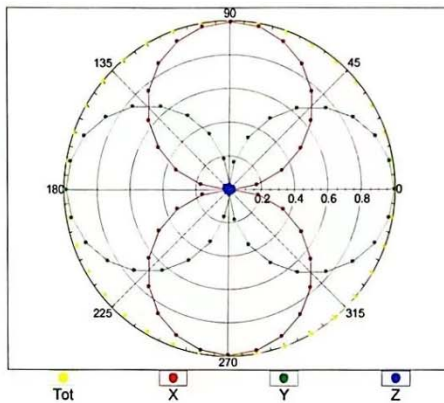
f=1800 MHz,R22,0°
