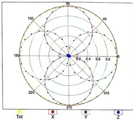
f=600 MHz,TEM,0°
