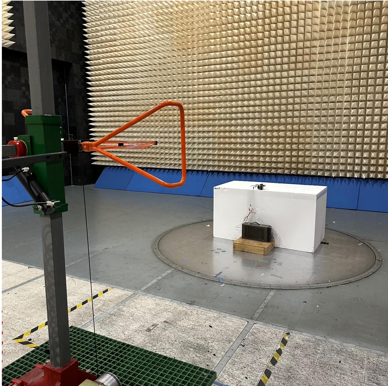
Radiated spurious emissions, 30MHz – 1GHz
