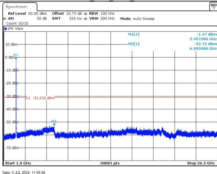
11AC40SISO_Ant1_2452_1000~26500
