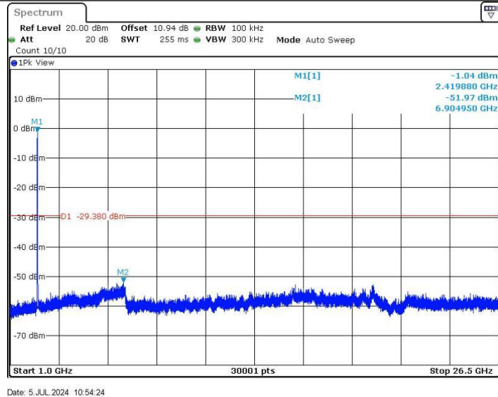
11AC20SISO_Ant1_2412_1000~26500
