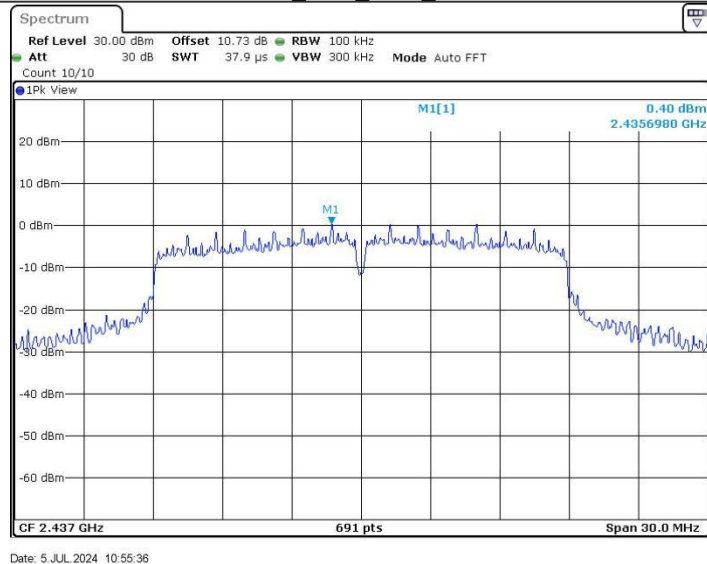
11AC20SISO_Ant1_2437_0~Reference
