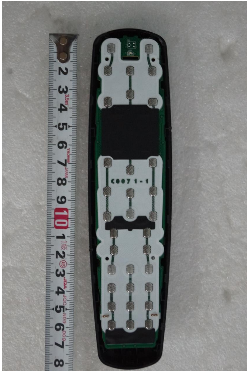
< Inside view >
