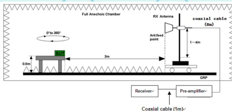
Above 1GHz
