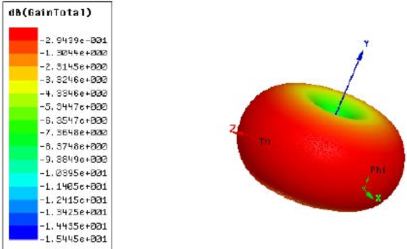
Antenna gain
