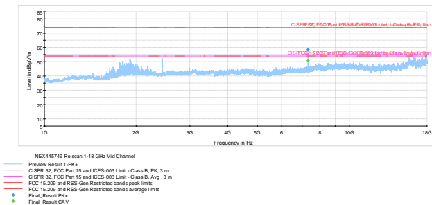
Figure 8.6-10: Radiated spurious emissions on Mid channel
