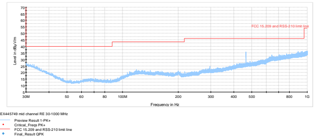
Figure 8.6-7: Radiated spurious emissions on Mid channel
