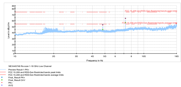
Figure 8.6-9: Radiated spurious emissions on Low channel
