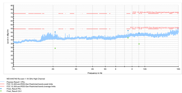
Figure 8.6-11: Radiated spurious emissions on High channel
