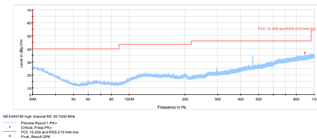
Figure 8.6-8: Radiated spurious emissions on High channel
