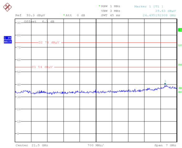
Figure 8.6-12: Radiated spurious emissions on Low channel
