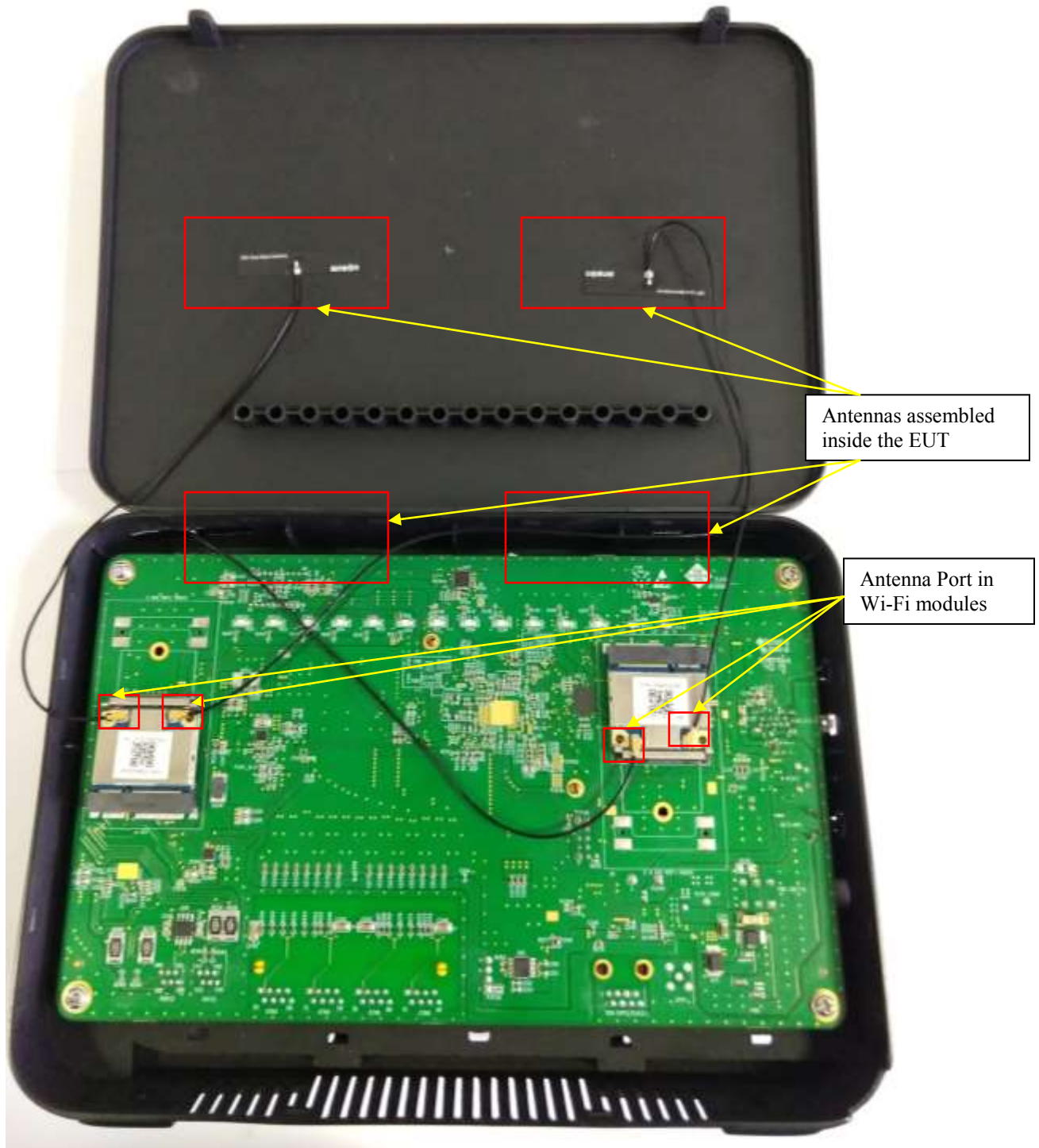
Picture – 3: Antenna connection
