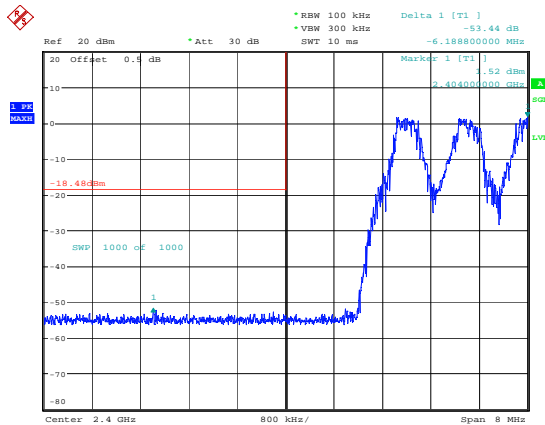
DH1_Hopping_Lower 53.44dB
