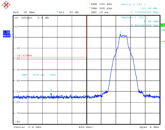
DH1_Low 53.26dB
