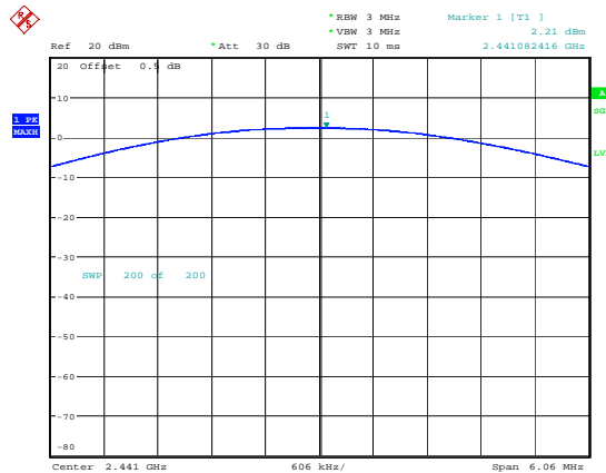
2DH1_2441 2.21dBm
