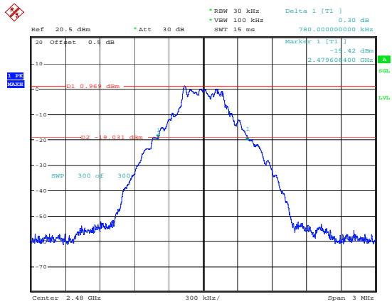
DH1_High 0.780MHz
