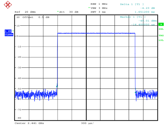
DH3_Hopping 1.651ms
