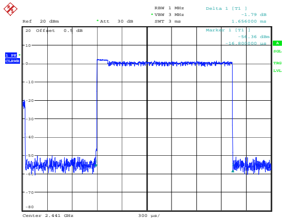
2DH3_Hopping 1.656ms
