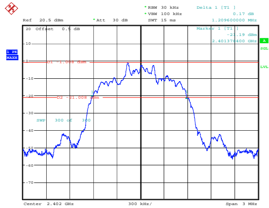
2DH1_Low 1.210MHz
