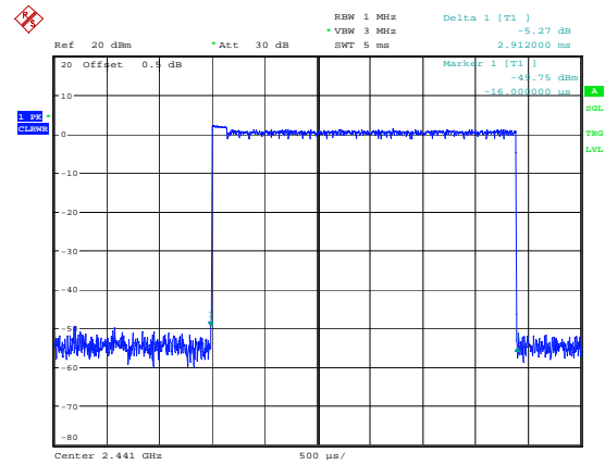
2DH5_Hopping 2.912ms
