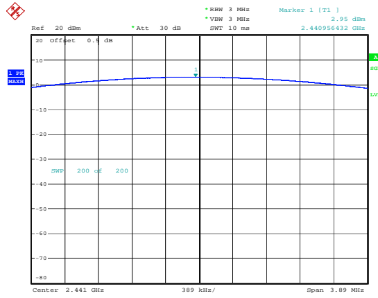
DH1_2440 2.95dBm
