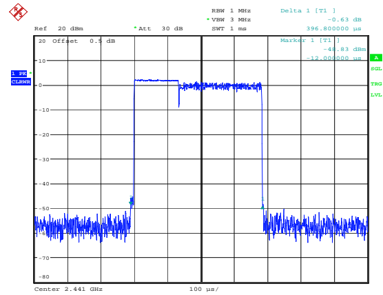
2DH1_Hopping 0.397ms
