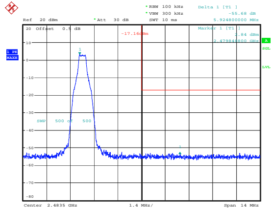
DH1_High 55.68dB
