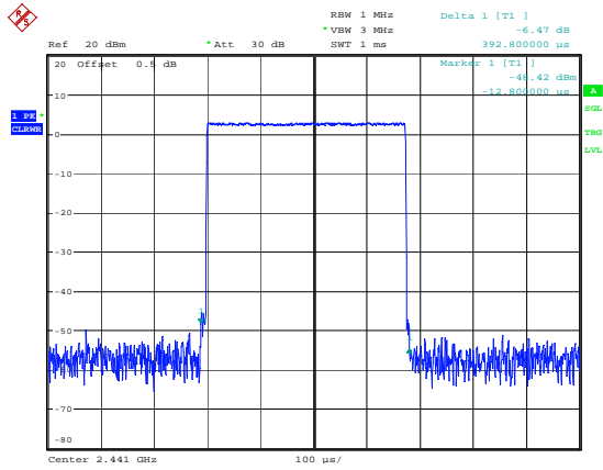
DH1_Hopping 0.393ms
