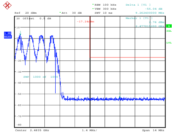
DH1_Hopping_Upper 55.04dB
