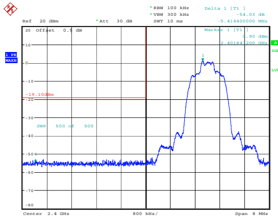
2DH1_Low 54.03dB
