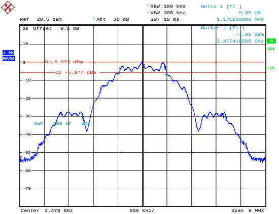
BLE_2M_High_Channel
