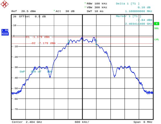
BLE_2M_Low_Channel
