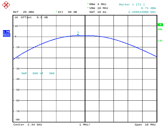
BLE_2M_Middle_Channel
