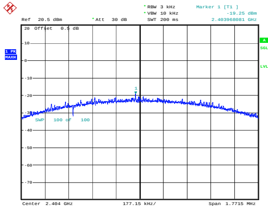
BLE_2M_Low_Channel
