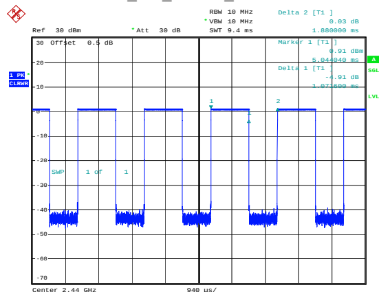
BLE_2M_Middle_Channel
