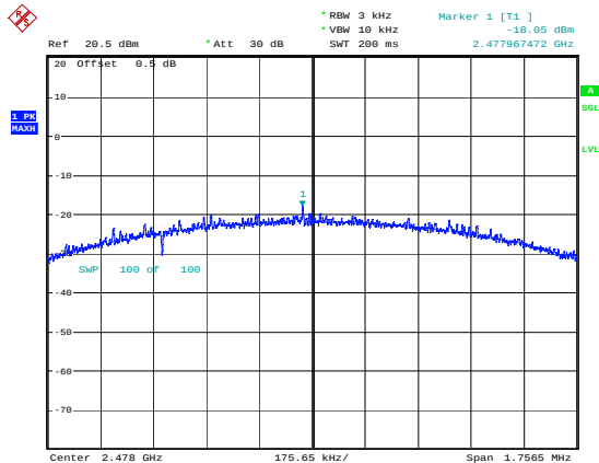
BLE_2M_High_Channel
