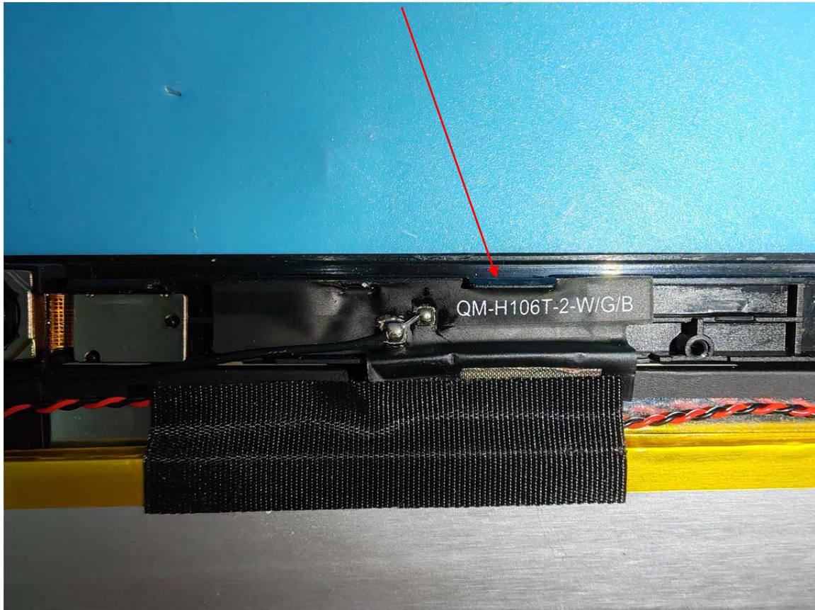
WiFi/GPS/BT Antenna
