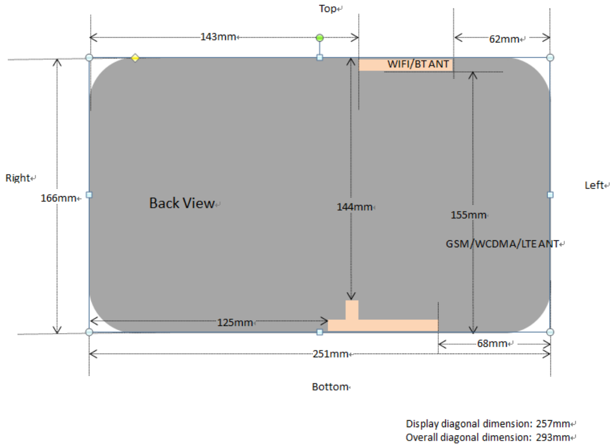
Fig.14.1 EUT Antenna Locations
