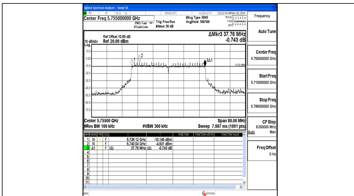
11AX40MIMO-Ant2-5755-PASS
