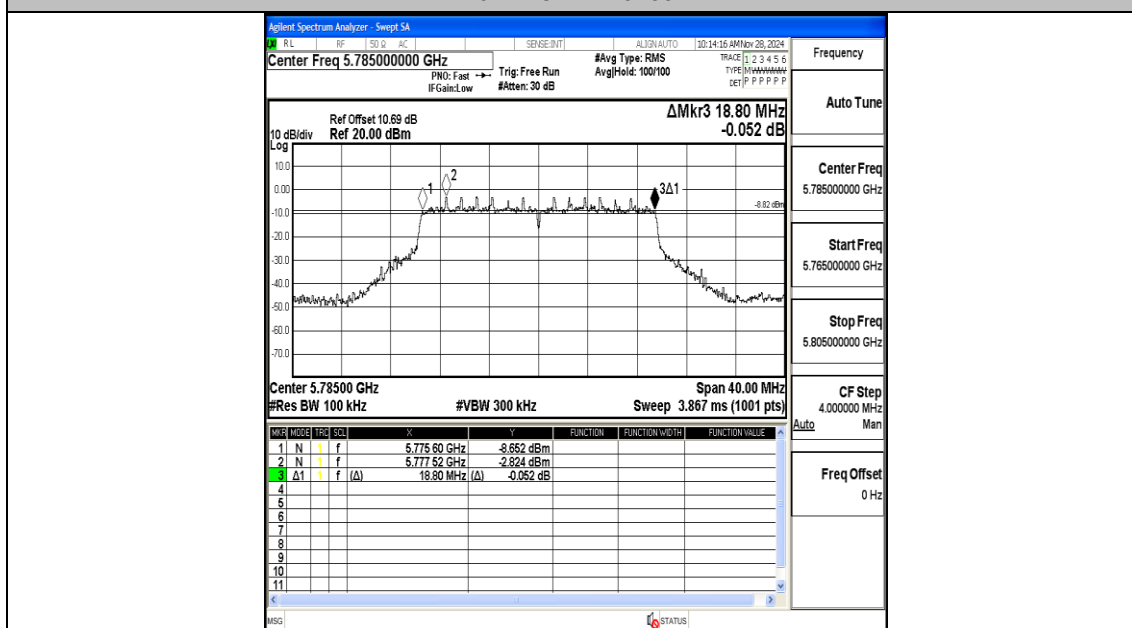
11AX20MIMO-Ant2-5785-PASS
