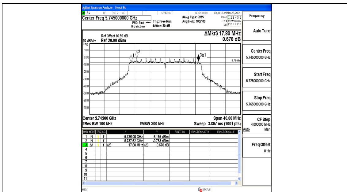
11AX20MIMO-Ant2-5745-PASS
