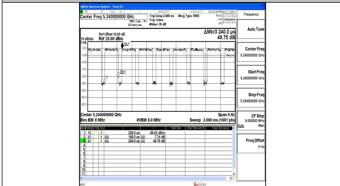
NTNV-11AC20MIMO-Ant2-5240
