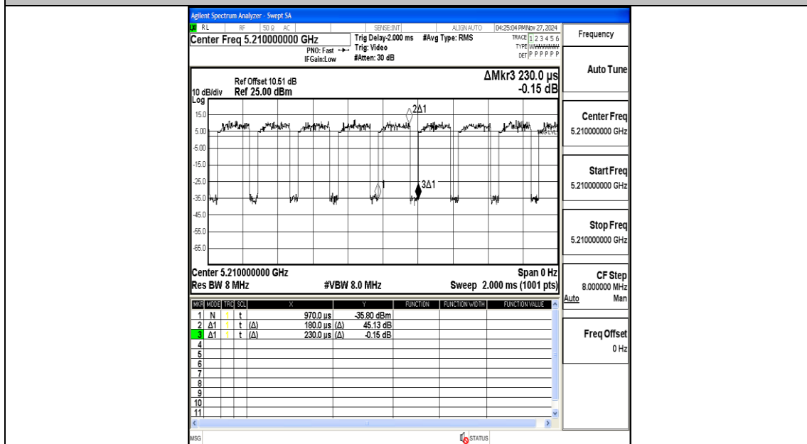
NTNV-11AX80MIMO-Ant2-5210
