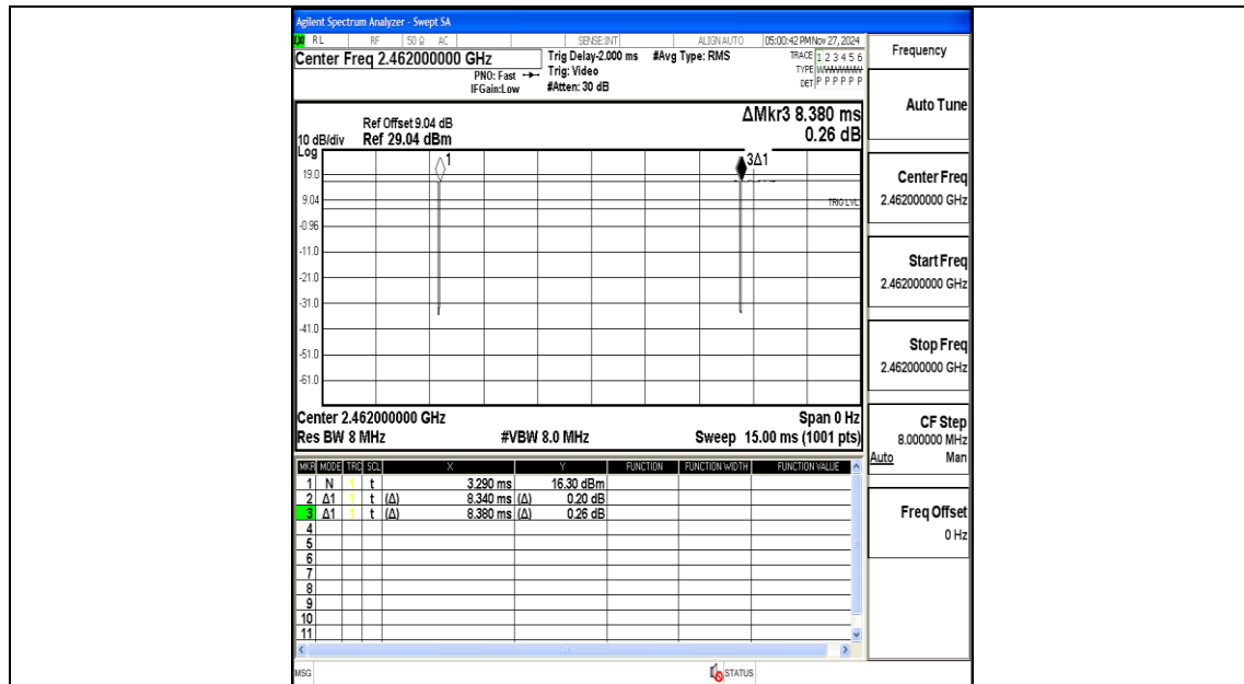
NTNV-11B-Ant2-2462
