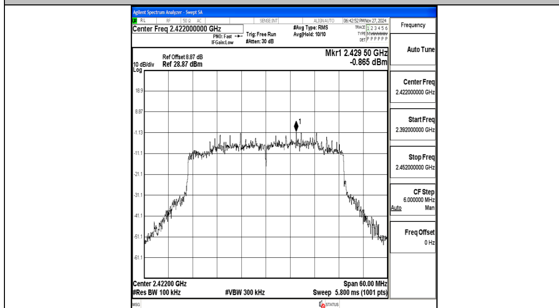
11AX40MIMO-Ant2-2422-0~Reference-PASS
