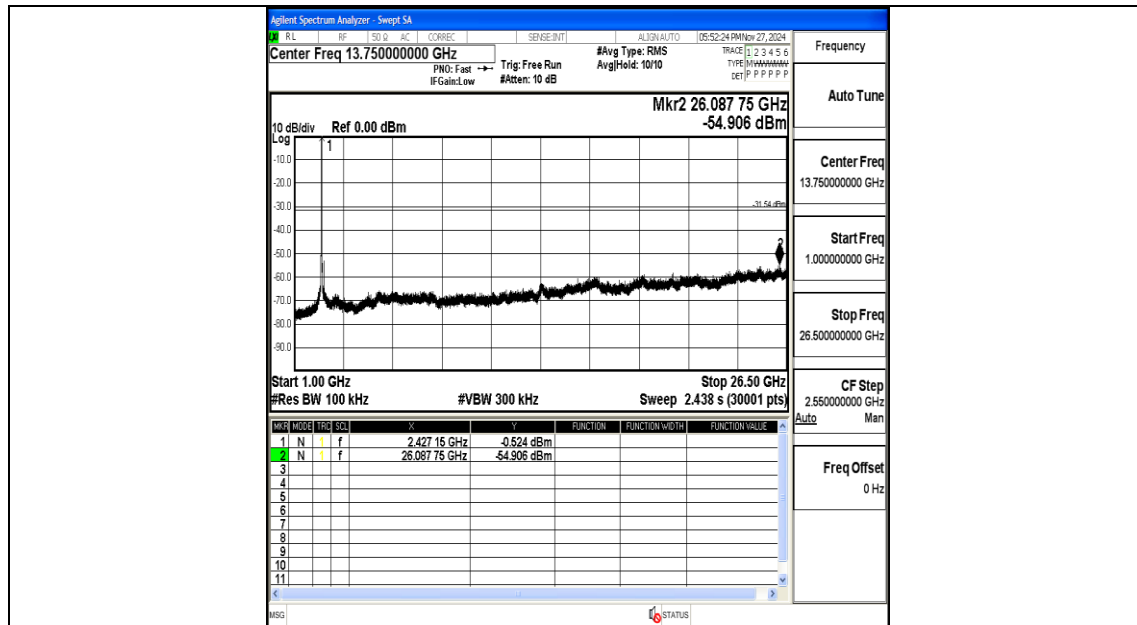
11N40MIMO-Ant2-2422-1000~26500-PASS
