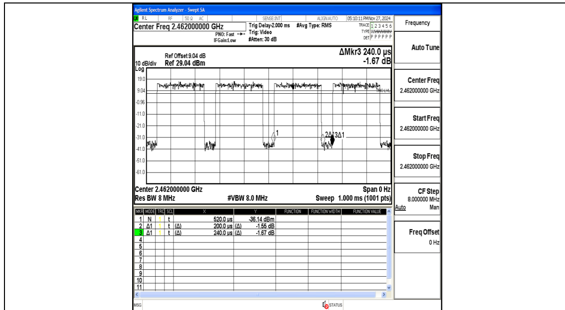
NTNV-11G-Ant2-2462
