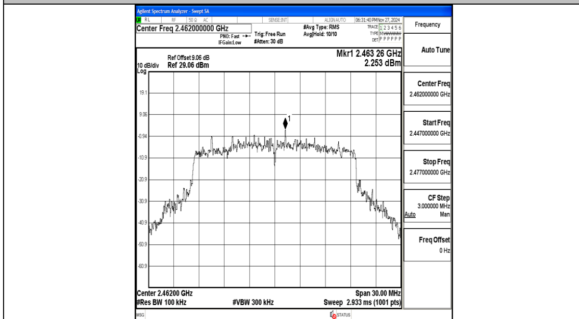
11AX20MIMO-Ant1-2462-0~Reference-PASS
