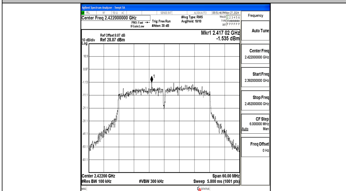
11N40MIMO-Ant2-2422-0~Reference-PASS
