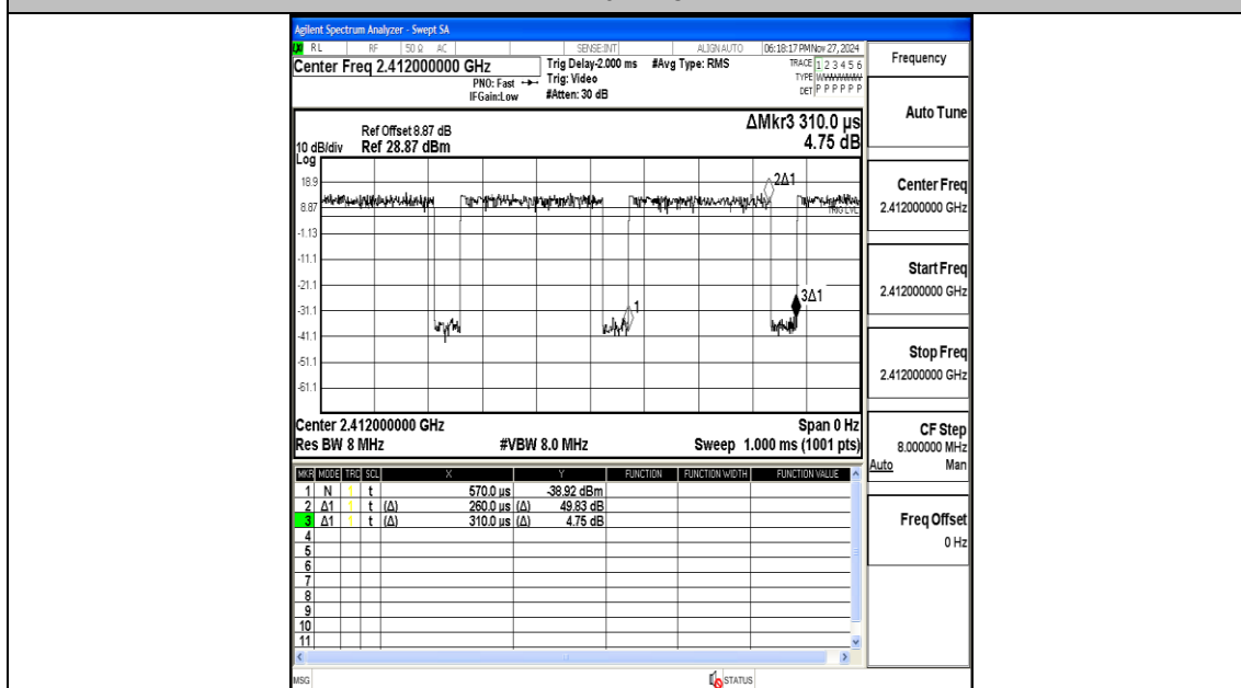
NTNV-11AX20MIMO-Ant2-2412
