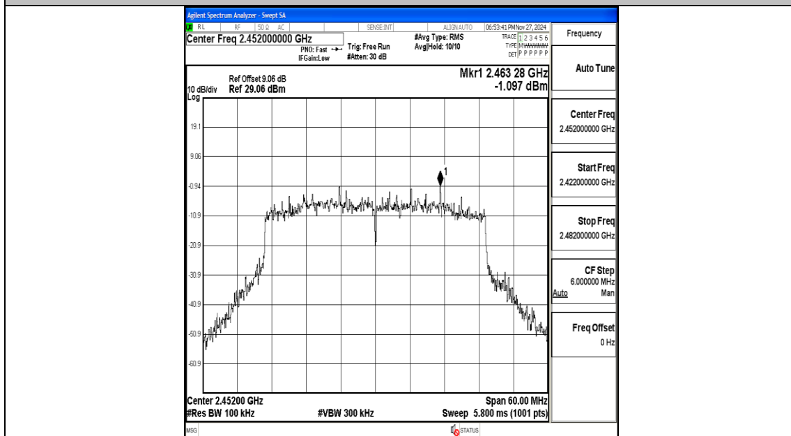
11AX40MIMO-Ant1-2452-0~Reference-PASS
