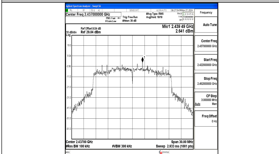
11AX20MIMO-Ant2-2437-0~Reference-PASS
