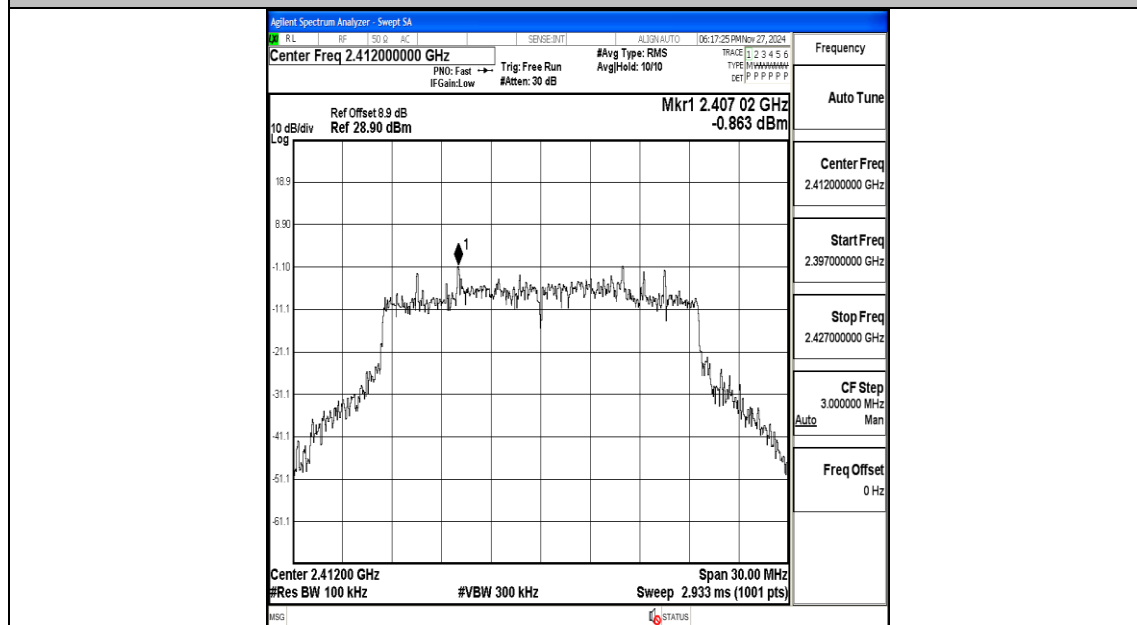
11AX20MIMO-Ant1-2412-0~Reference-PASS
