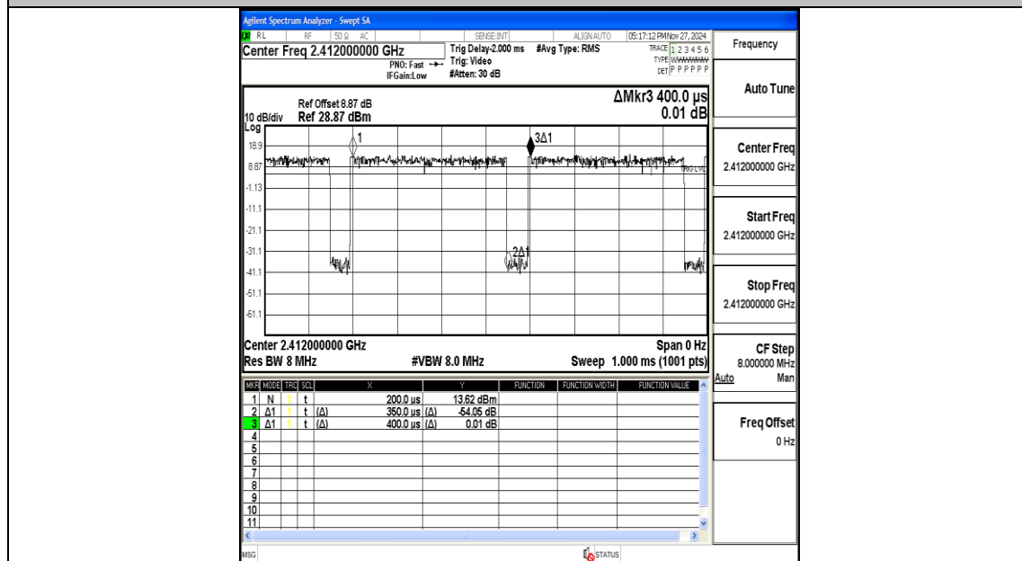
NTNV-11N20MIMO-Ant2-2412
