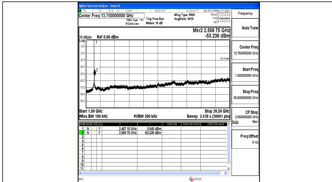
11AX20MIMO-Ant2-2462-1000~26500-PASS
