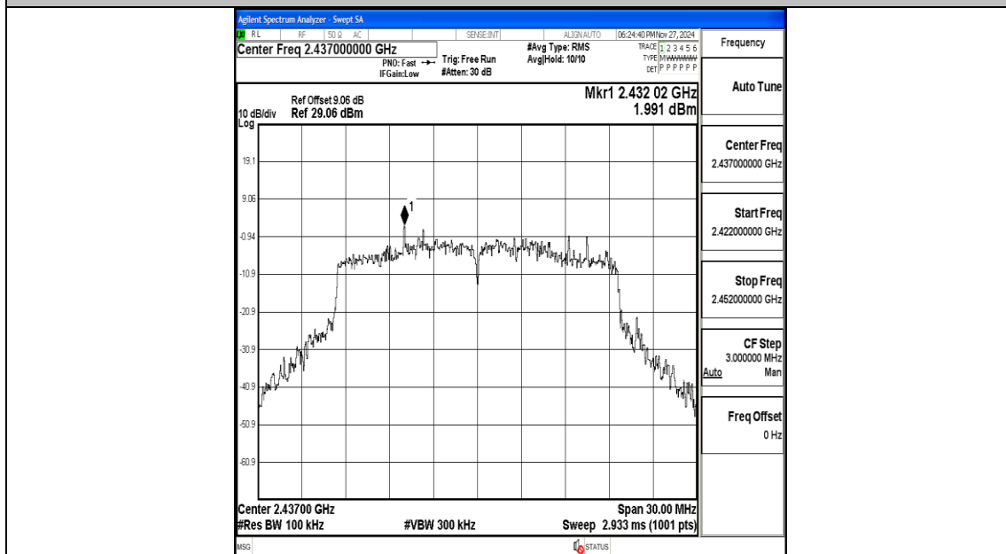
11AX20MIMO-Ant1-2437-0~Reference-PASS
