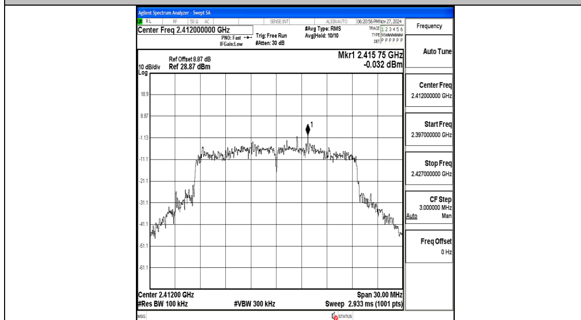
11AX20MIMO-Ant2-2412-0~Reference-PASS
