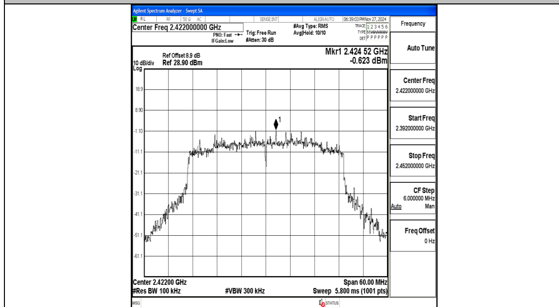
11AX40MIMO-Ant1-2422-0~Reference-PASS
