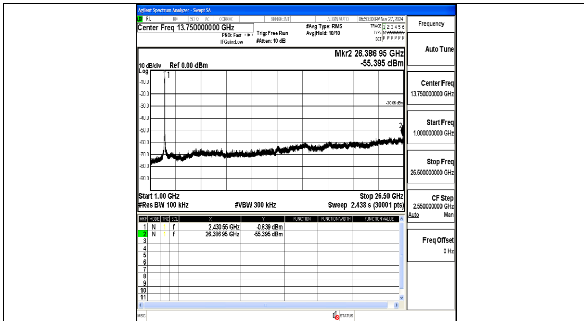
11AX40MIMO-Ant2-2437-1000~26500-PASS
