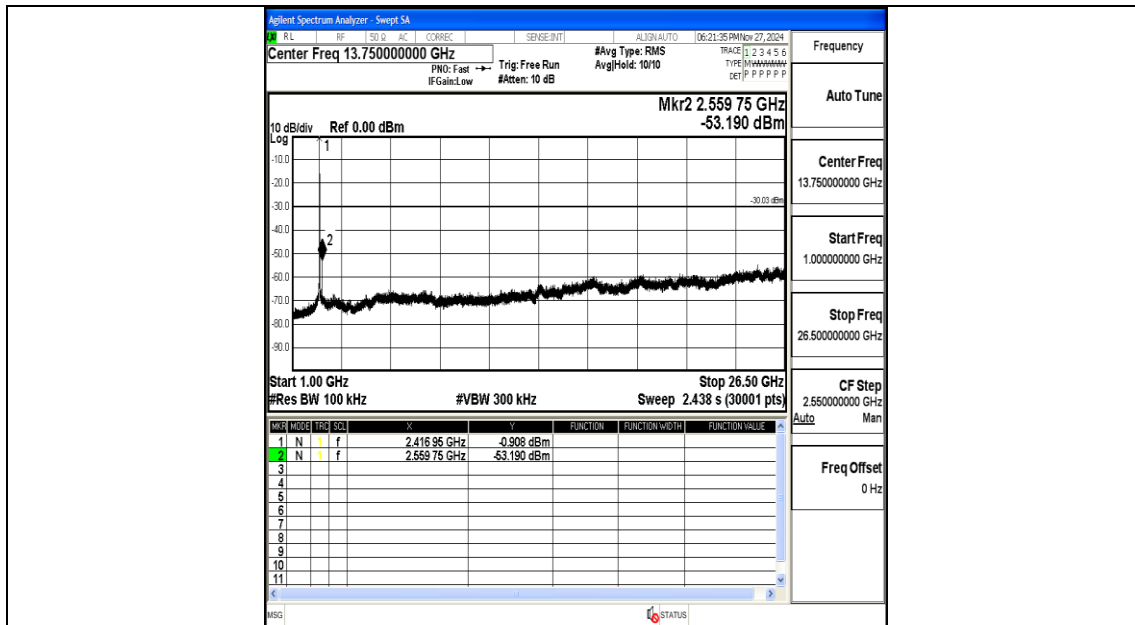
11AX20MIMO-Ant2-2412-1000~26500-PASS
