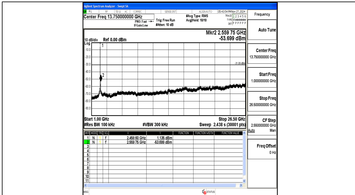
11N20MIMO-Ant2-2462-1000~26500-PASS
