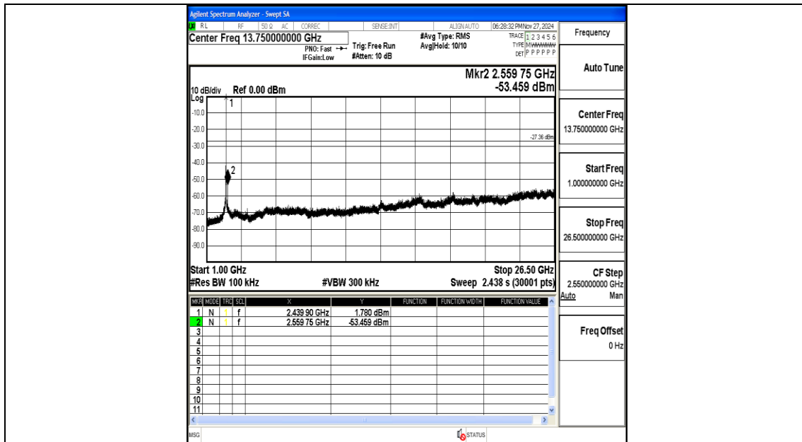
11AX20MIMO-Ant2-2437-1000~26500-PASS
