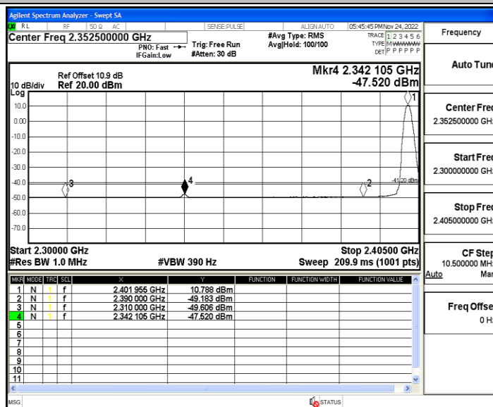
DH5_Ant2_Low_2402_Peak
