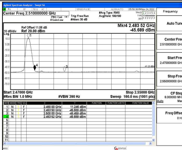
DH5_Ant2_High_2480_Peak
