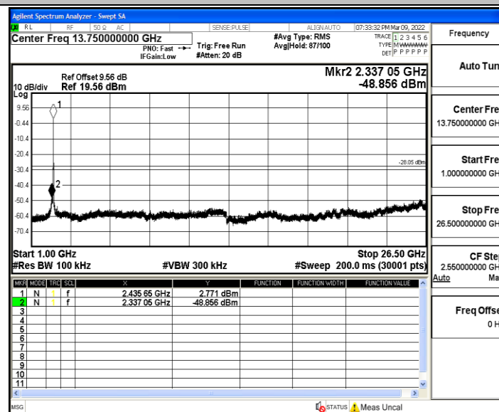
11G_Ant2_2437_0~Reference
