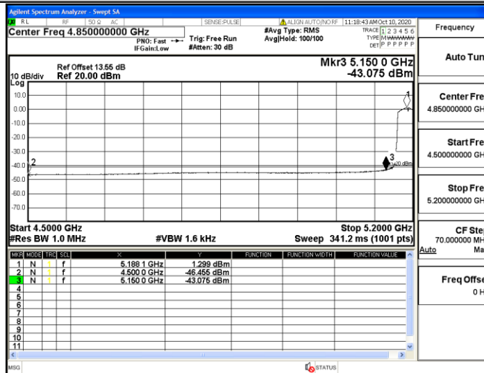
11AC40SISO_Ant1_Low_5190_Peak
