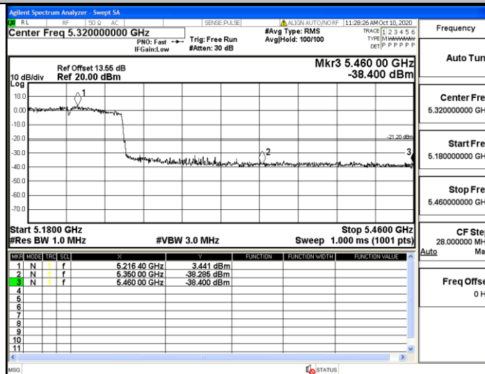
11AC80SISO_Ant1_High_5210_Peak
