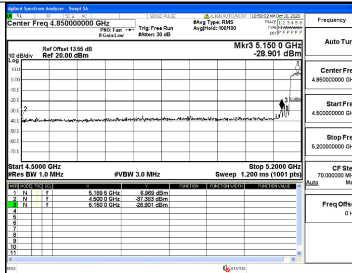
11N40SISO_Ant1_High_5230_AV
