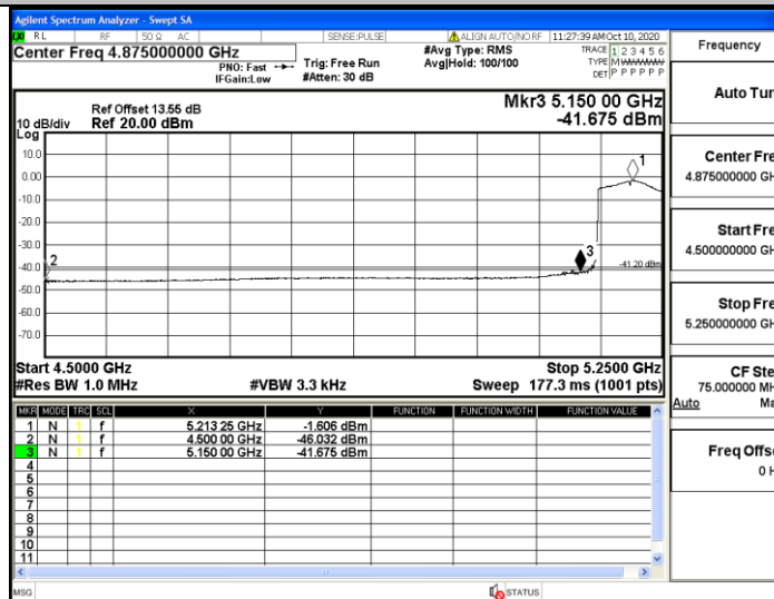
11AC80SISO_Ant1_Low_5210_Peak
