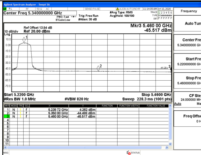
11AC20SISO_Ant1_High_5240_Peak
