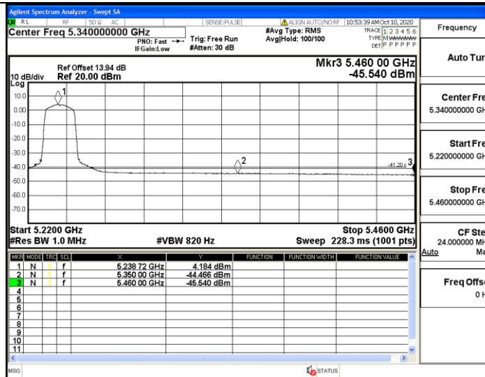
11N20SISO_Ant1_High_5240_Peak
