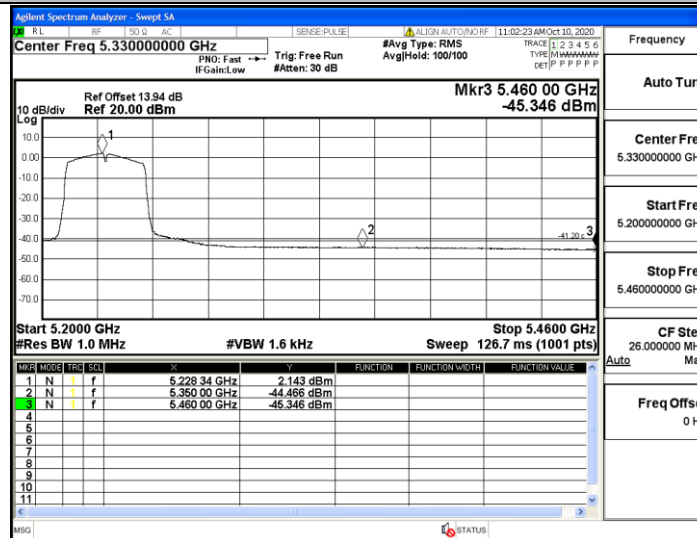
11N40SISO_Ant1_High_5230_Peak
