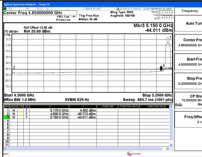
11AC20SISO_Ant1_Low_5180_Peak
