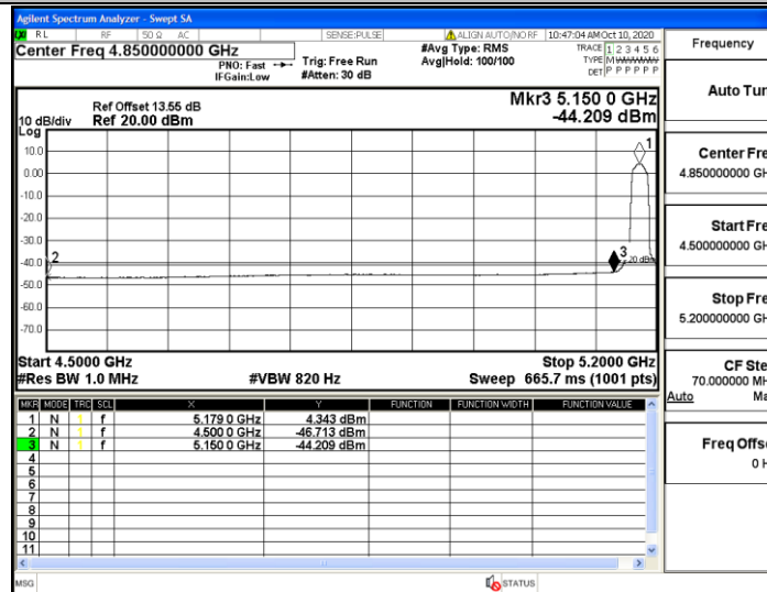
11N20SISO_Ant1_Low_5180_Peak
