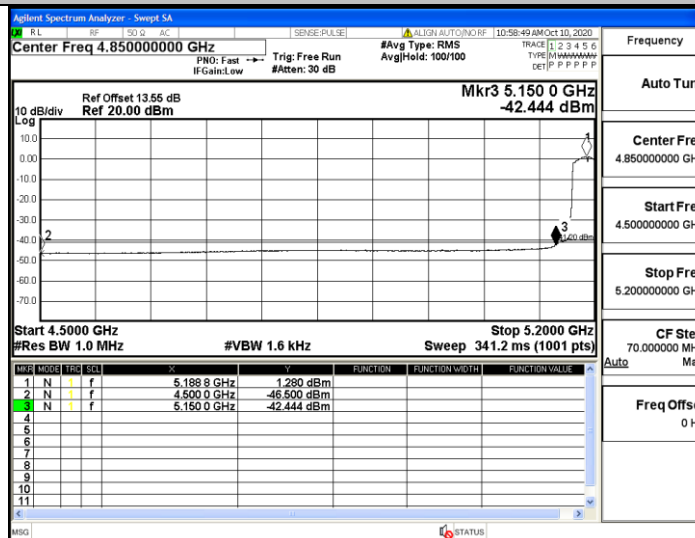
11N40SISO_Ant1_Low_5190_Peak
