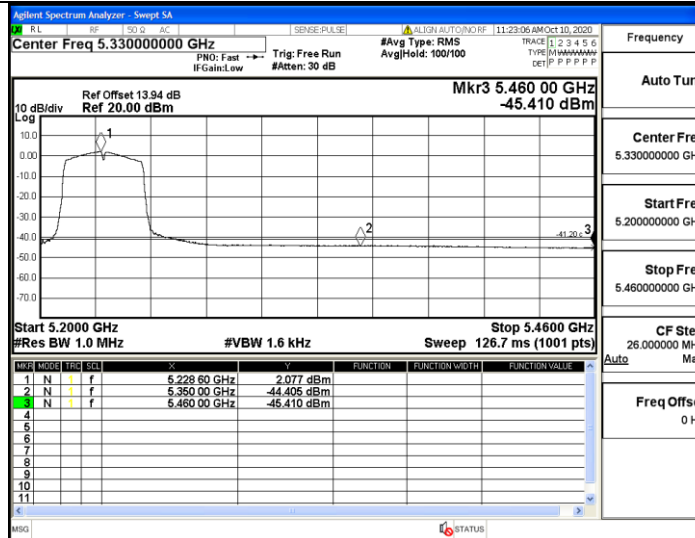
11AC40SISO_Ant1_High_5230_Peak
