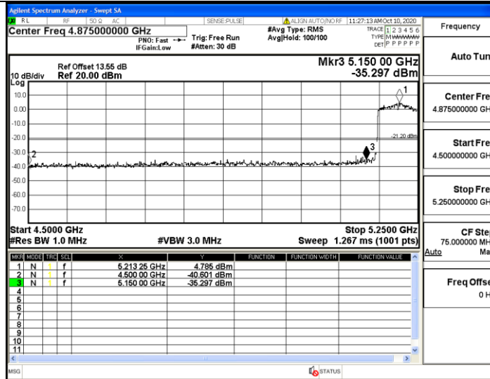
11AC80SISO_Ant1_High_5210_AV
