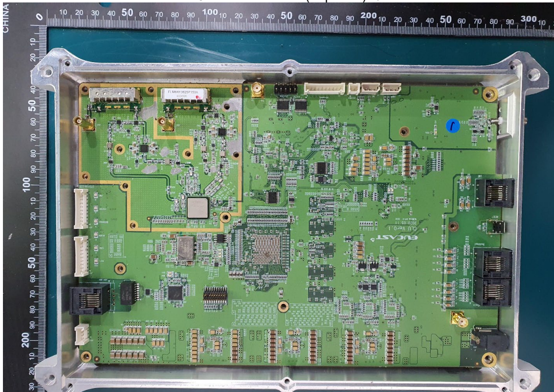
4. Internal Photo (Top view) 2/2
