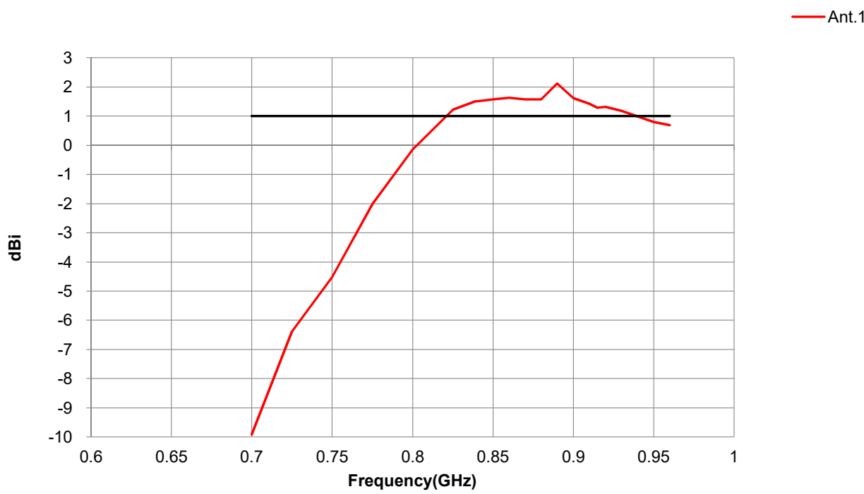
Peak Gain
