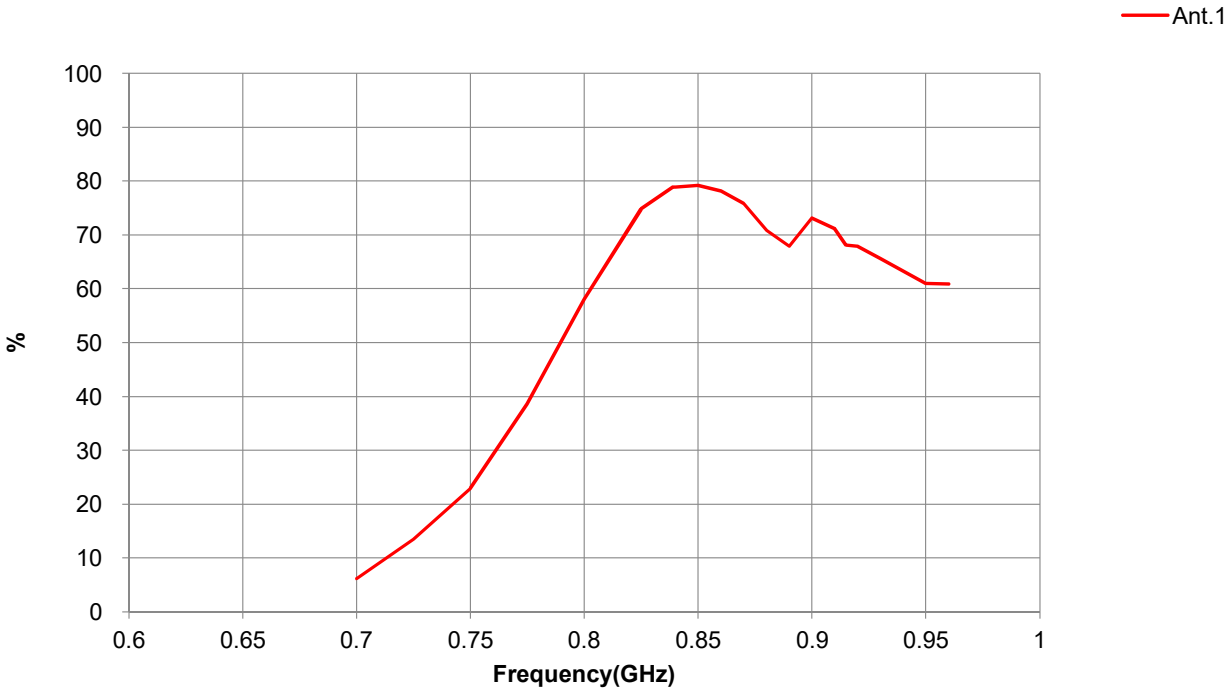
Efficiency
