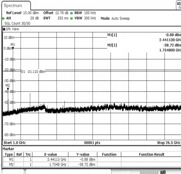
DH5-Ant1-2441-1000~26500-PASS
