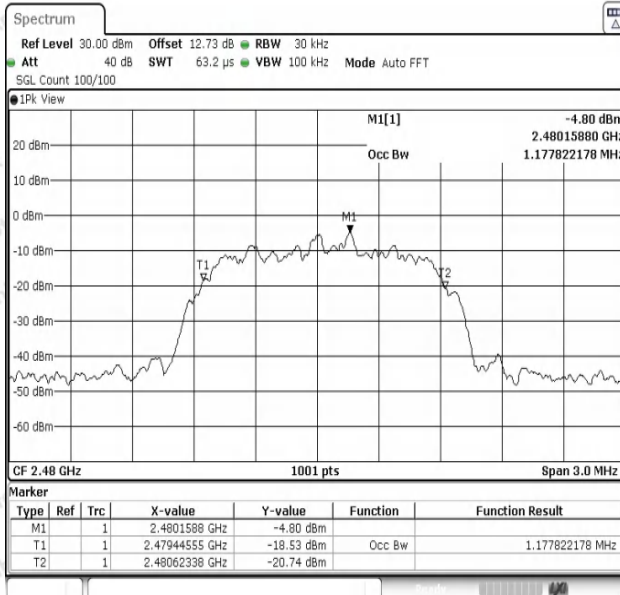
2DH5-Ant1-2480
