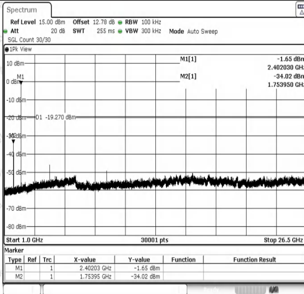
3DH5-Ant1-2402-1000~26500-PASS
