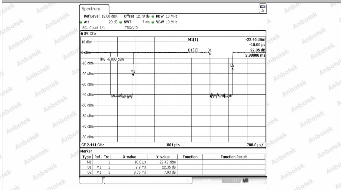
NTNV-DH5-Ant1-2441
