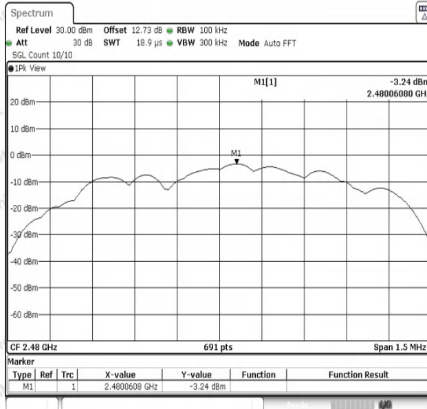
2DH5-Ant1-2480-0~Reference-PASS
