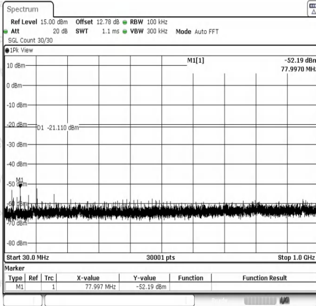
DH5-Ant1-2441-30~1000-PASS
