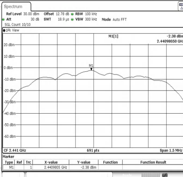
3DH5-Ant1-2441-0~Reference-PASS
