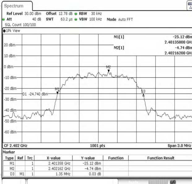
2DH5-Ant1-2402
