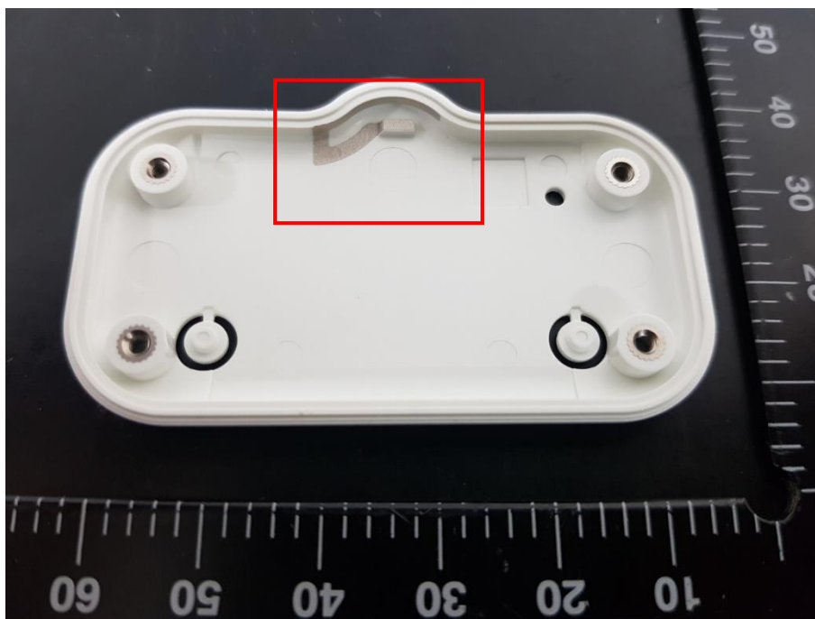
Main board – LDS Antenna
