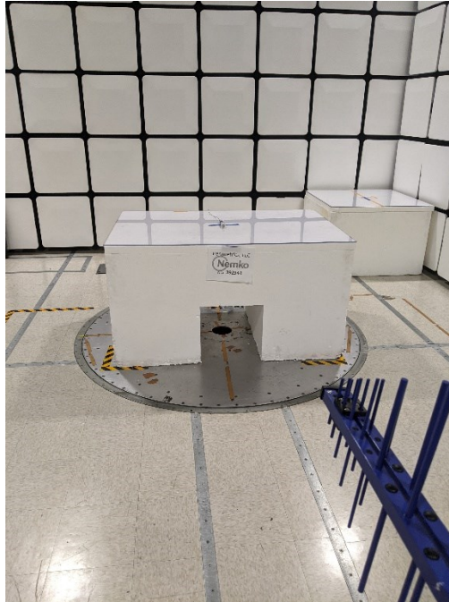
Figure 1 - Radiated emissions below 1 GHz, front view
