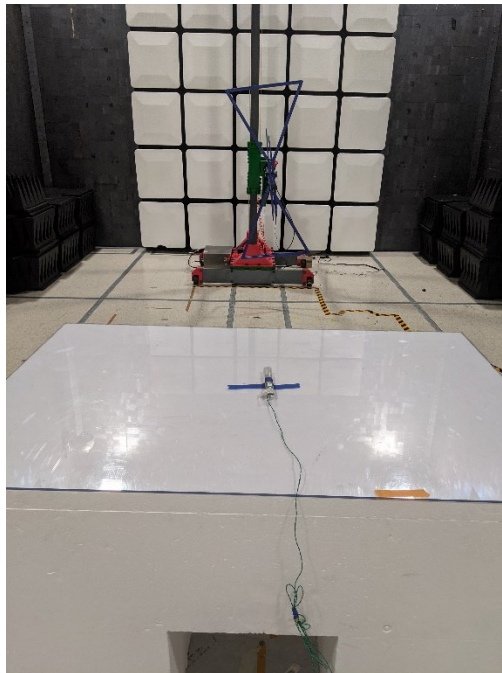
Figure 2 - Radiated emissions below 1 GHz, back view
