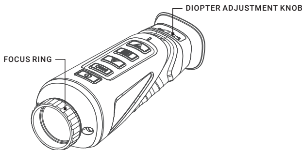
FIGURE 2-4. DIOPTER ADJUSTMENT KNOB AND FOCUS RING
