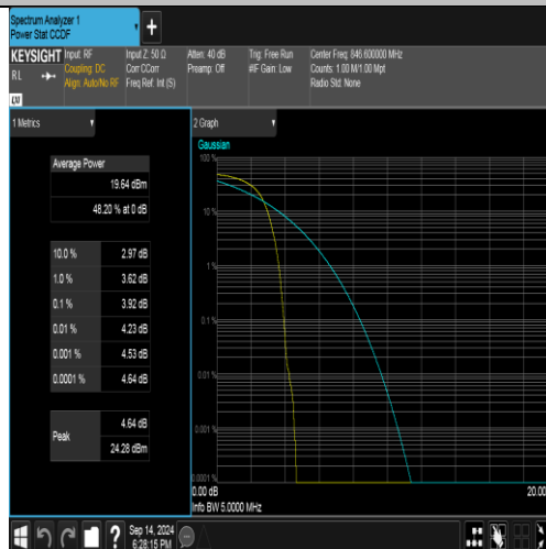
Band5-4233-4-PASS
