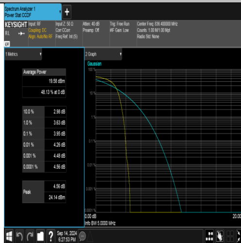
Band5-4182-4-PASS
