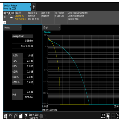
Band5-4182-PASS
