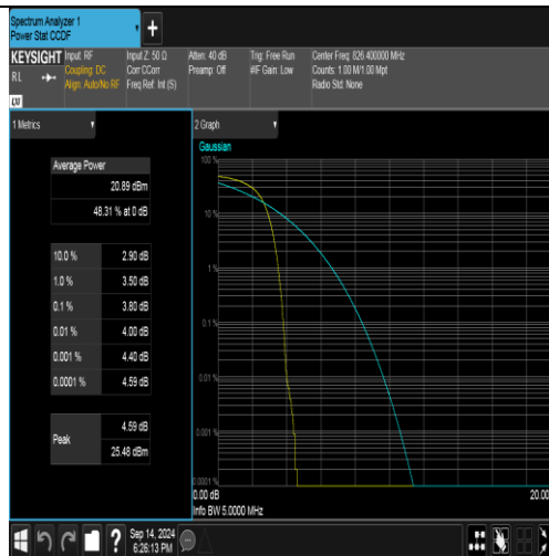
Band5-4132-3-PASS
