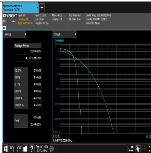
Band5-4132-4-PASS
