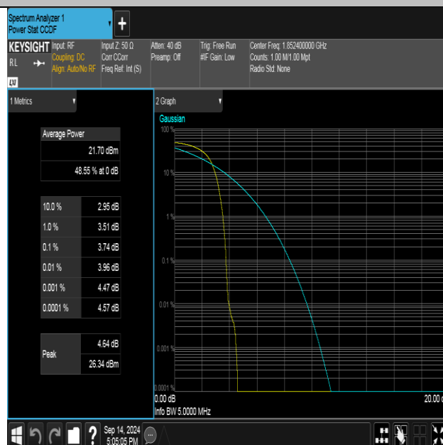
Band2-9262-4-PASS
