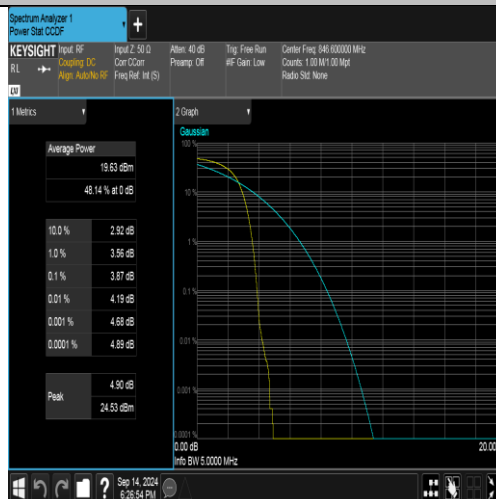
Band5-4233-3-PASS
