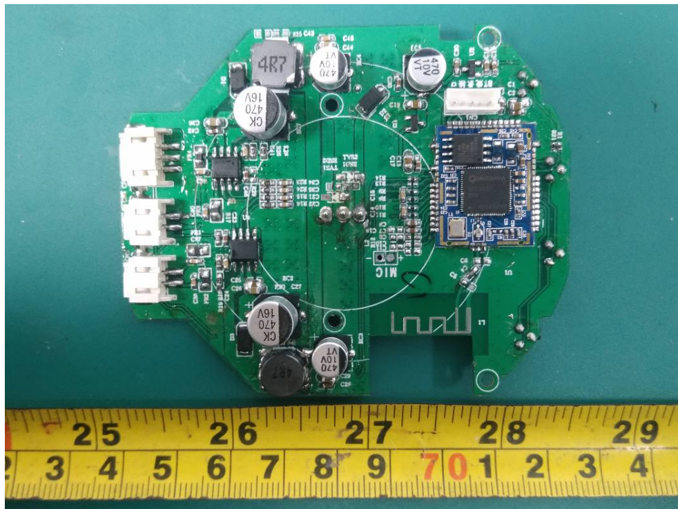
BT&BLE Antenna
