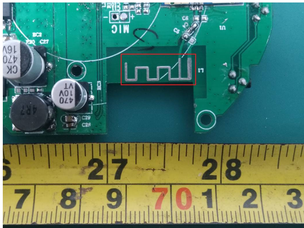
BT&BLE Antenna
