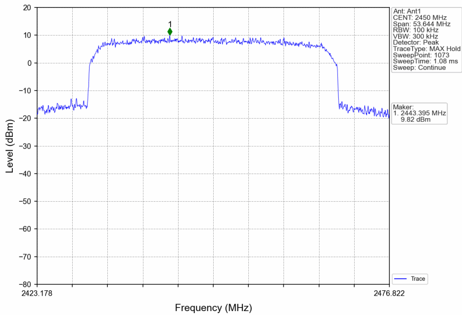
Slot40_HCH_2450MHz_Ant1_NTNV
