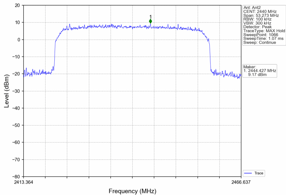
Slot40_MCH_2440MHz_Ant2_NTNV
