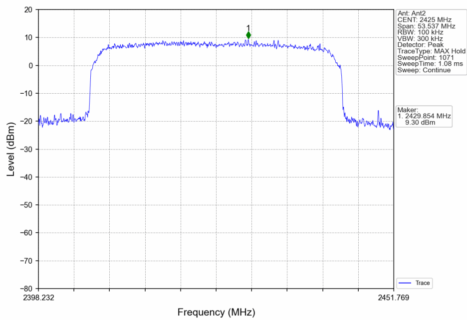
Slot40_LCH_2425MHz_Ant2_NTNV
