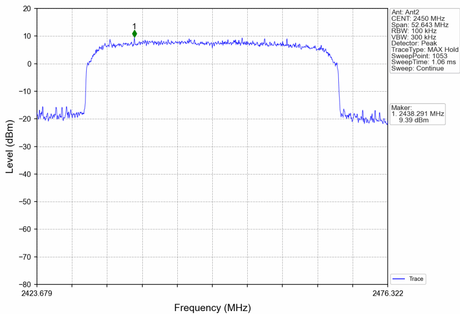
Slot40_HCH_2450MHz_Ant2_NTNV
