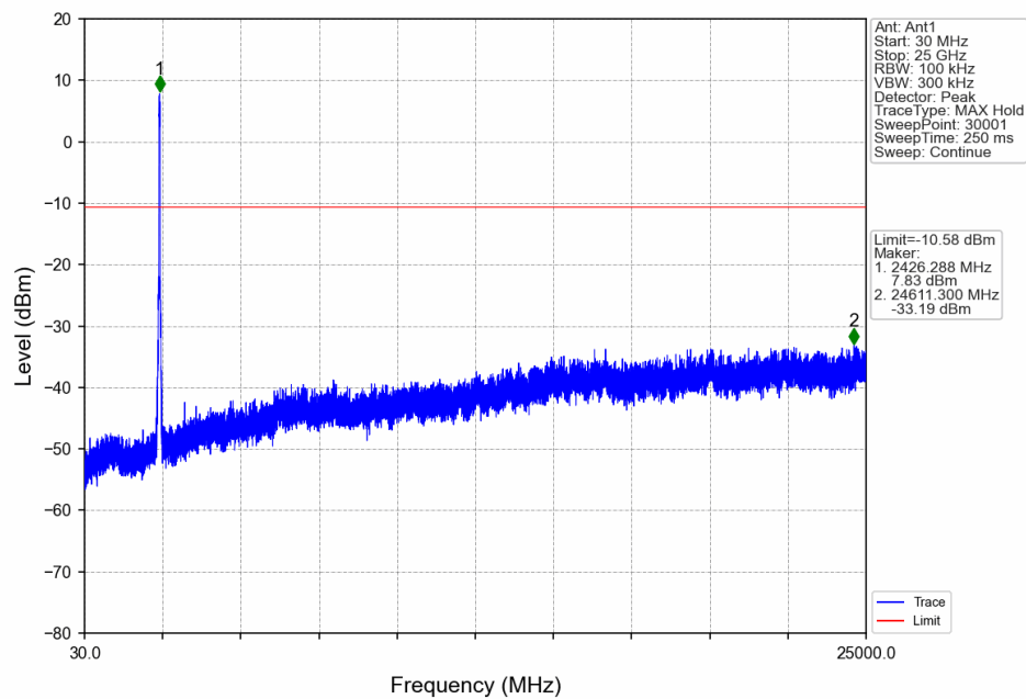
Slot40_LCH_2425MHz_Ant1_NTNV
