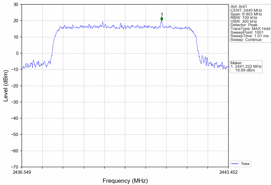
Slot5_MCH_2440MHz_Ant1_NTNV
