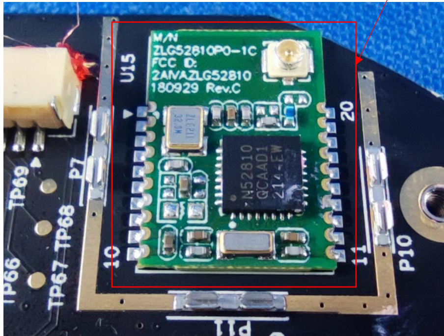
Bluetooth module(disable)
