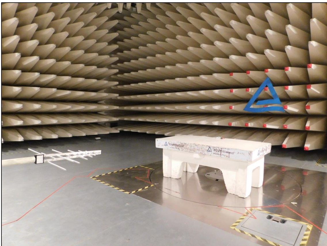
Frequency range :200MHz–1GHz
