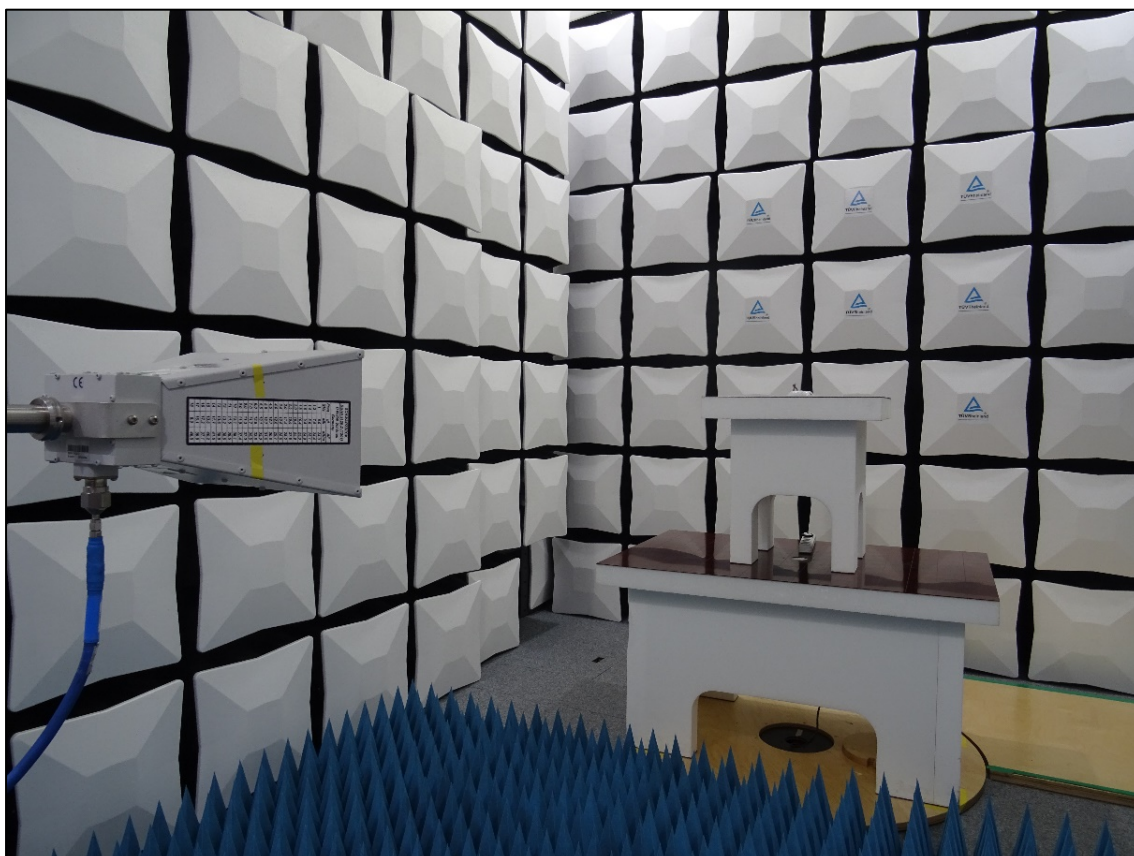
Frequency range :1GHz-18GHz
