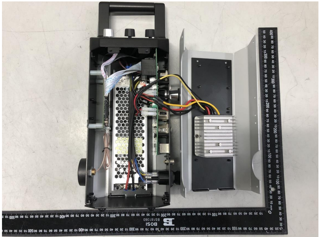
Photo 2 Inside of EUT (Control box)
