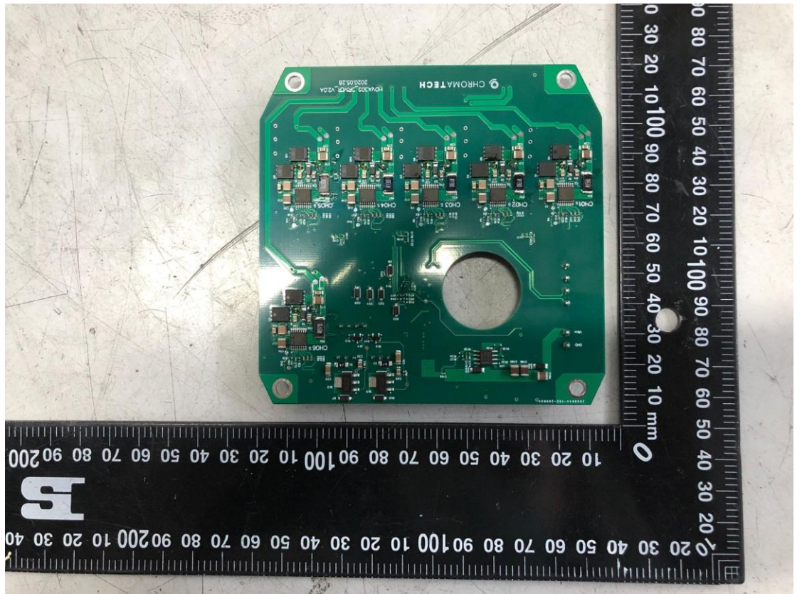
Photo 9 Inside of EUT (Lamp head)
