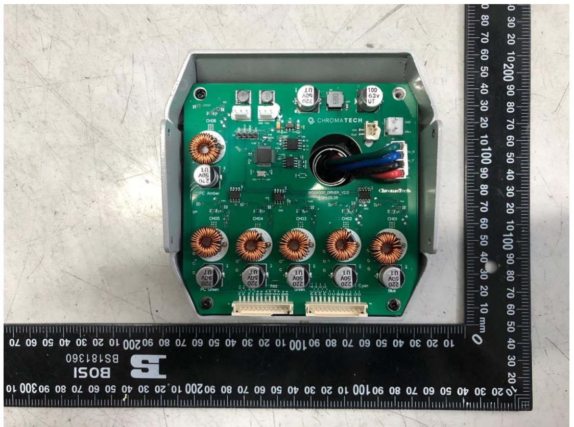
Photo 8 Inside of EUT (Lamp head)
