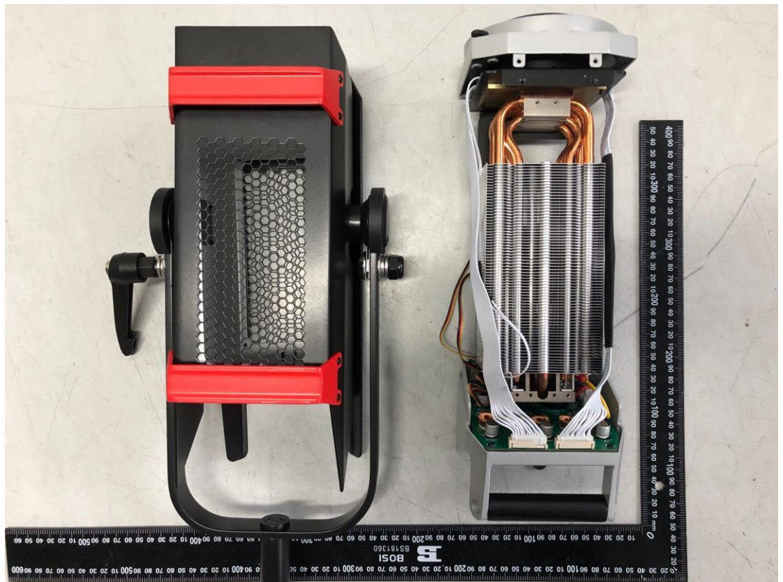
Photo 6 Inside of EUT (Lamp head)
