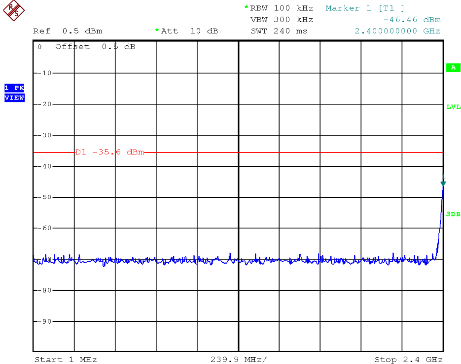
802.11g, Lowest Channel, Plot A
