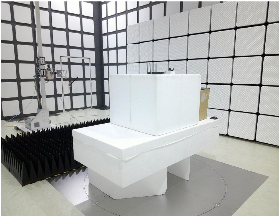
Description: Radiated Emission Test Setup for above 1GHz
